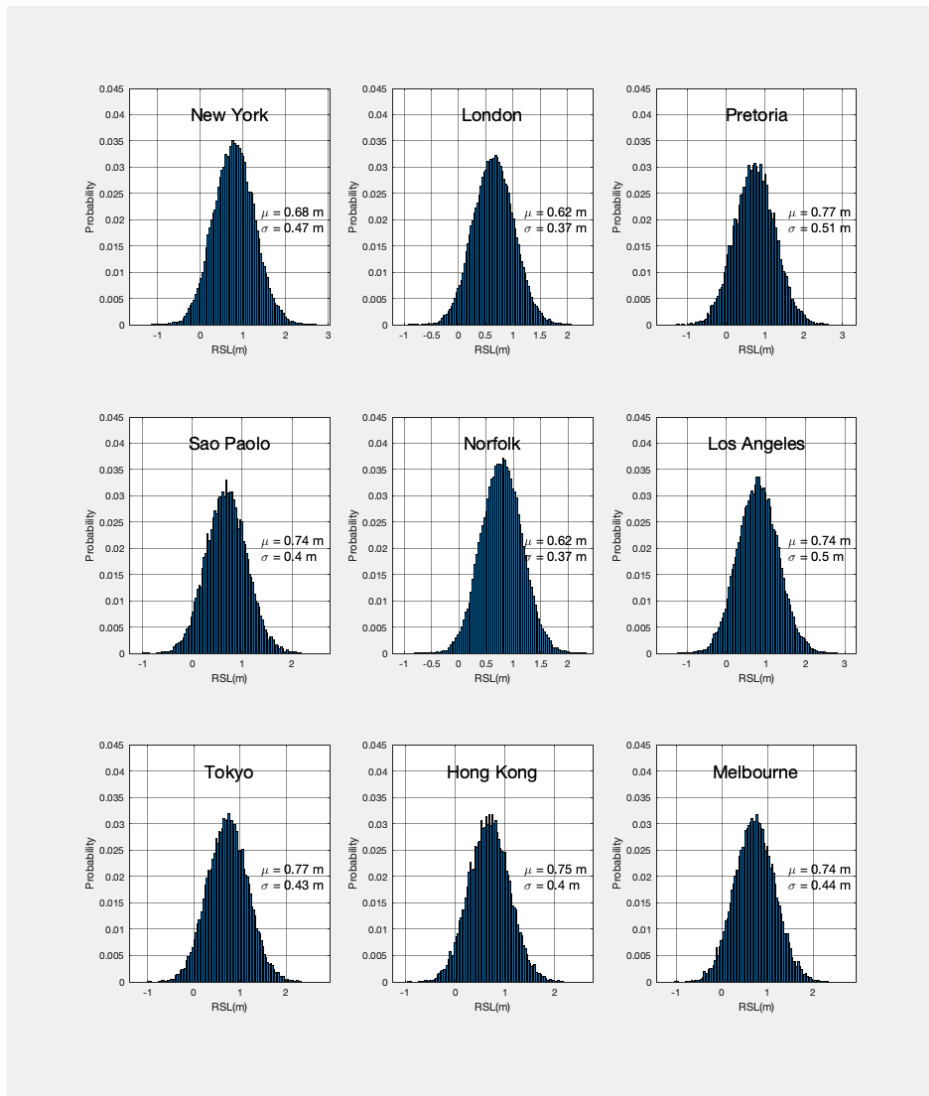
Figure 10. AR5 calibrated projection of RSL for nine cities around the world [.. 39 ] from 2007 to 2100. Sampling was carried out for H_{AIS} , H_{GIS} , H_{GLA} , STR and H_{TWS} using mean and standard deviations from AR5 (Church et al., 2013a). The patterns for ice thickness are from GRACE 2003-2016 trends (Adhikari and Ivins, 2016). DSL is fully deterministic, from the CMIP5 NorESM runs (Bentsen et al., 2013). RSL_{GIA} was deterministically set to 0. Each time step was sampled for using 10,000 LHS samples.
