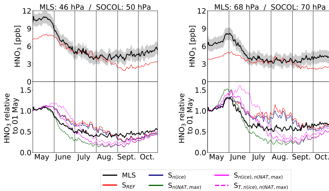
Figure 7. Temporal evolution of polar (60°S-82°S) mean gas-phase HNO 3 from MLS measurements and the different model simulations. The uncertainty-range (gray shading) represent the MLS accuracy.
