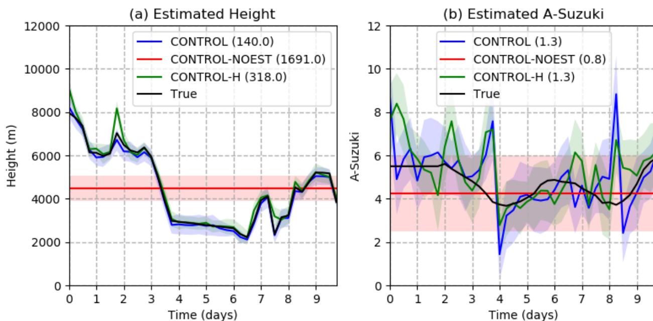
Figure 6. Optimized parameters as a function of time in the CONTROL (blue line) and CONTROL-NOEST (red line) experiments. The shade surrounding the estimated values represents +/- one standard deviation. (a) h parameter and (b) A - Suzuki parameter. The black line indicates the value of the parameters in the true run.
