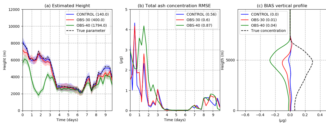
Figure 11. As in Figure 9 but for the experiments CONTROL, OBS-30 and OBS-40.
