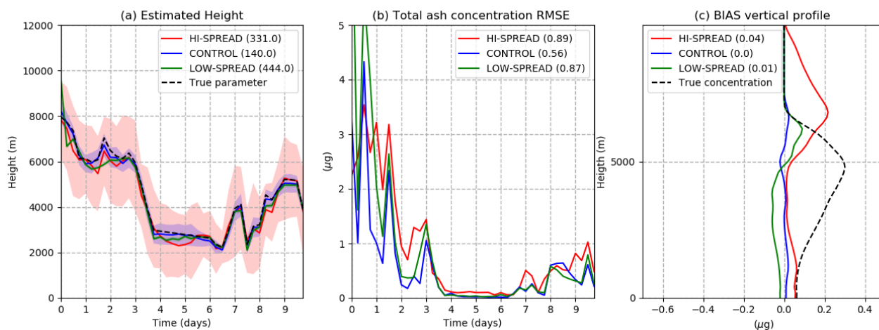
Figure 9. (a) Estimated h as a function of time for the HI-SPREAD (red line), CONTROL (blue line) and LOW-SPREAD (green line). The shade surrounding the estimated values represents \pm one standard deviation and the black dashed line indicates the true parameter value. (b) Spatially averaged total ash concentration 6-hour forecast RMSE as a function of time. Line color code as in (a). (c) Temporally averaged 6-hour forecast bias as a function of height. Line color code as in (a).
