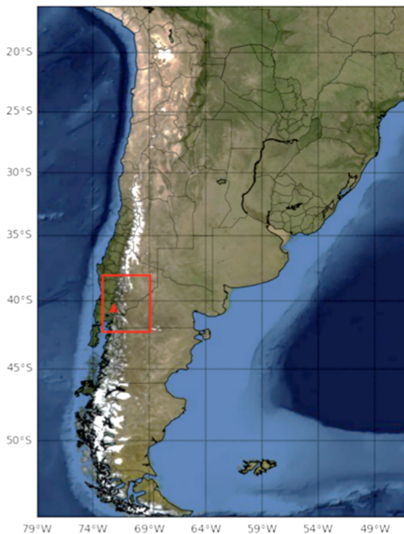
Figure 2. Domain used in the ETKF-FALL3D sensitivity tests (red square).
