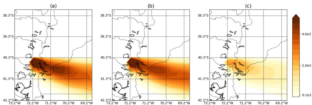
Figure 8. (a) Nature run ash concentration at flight level 200 (shaded, \mu g^{-1} ), (b) as in (a) but for the 6-hour forecast of ash concentration initialized from the CONTROL analysis experiment, (c) as in (b) but for the NOOPT experiment, corresponding to the 12 th assimilation cycle.
