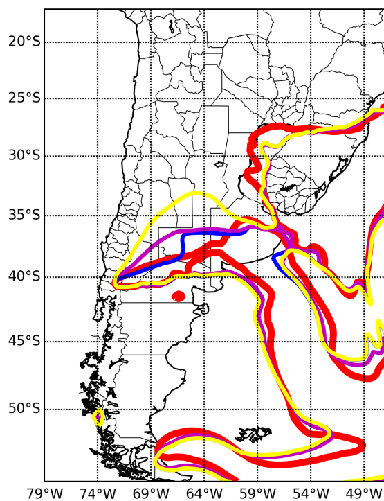
Figure 12. Ash mass loading 0.2 \text{ gm}^{-2} contours from: the nature run (red), ensemble mean optimized parameters run (blue) and the 12 (magenta) and 24 (yellow) hours forecasts verifying at the 8 th of June at 00:00 UTC over a larger domain (see the text for details).
