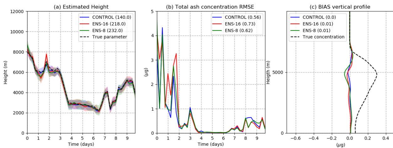
Figure 10. As in Figure 9 but for the experiments CONTROL, ENS-16 and ENS-8.
