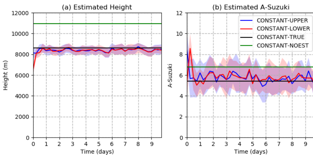
Figure 4. Optimized parameters as a function of time in the CONSTANT-UPPER (blue line), CONSTANT-LOWER (red line), CONSTANT-TRUE (black line) and CONSTANT-NOEST (green line) experiments. The shade surrounding the CONSTANT-UPPER and CONSTANT-LOWER estimated values represents \pm one standard deviation. (a) h parameter and (b) A - Suzuki parameter.
