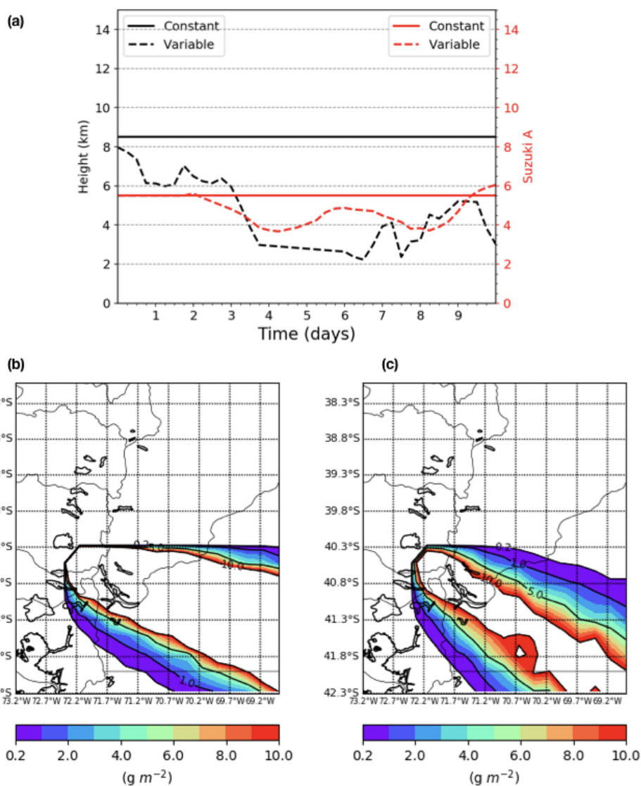
Figure 3. (a) Nature run parameters time series for the constant (solid lines) and variable emission profiles (dashed lines) and for h (black lines) and A - Suzuki (red lines). Ash mass loading on 7th June 12:00 UTC with for the (b) constant parameters nature run and the (c) time dependent parameters nature run. Ash mass loading values outside the 0.2 - 10.0 g m^{-2} interval are masked out.
