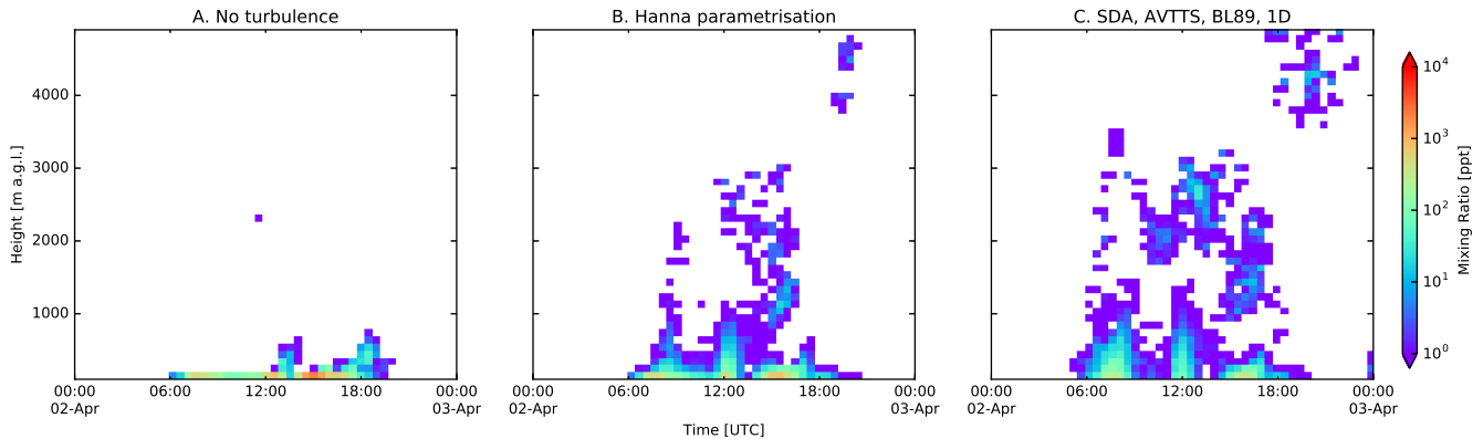
Figure 6. Marine boundary layer tracer profile evolution at the Maïdo observatory. On the left a simulation without turbulent motions taken into account. The middle panel shows the traditional FLEXPART turbulent mode. On the right hand side we show the results with the new turbulent mode.
