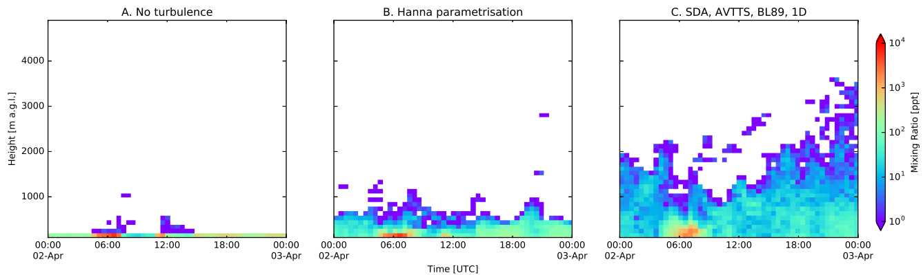
Figure 7. Marine boundary layer tracer profile evolution above sea. On the left a simulation without turbulent motions taken into account. The middle panel shows the traditional FLEXPART turbulent mode. On the right hand side we show the results with the new turbulent mode.
