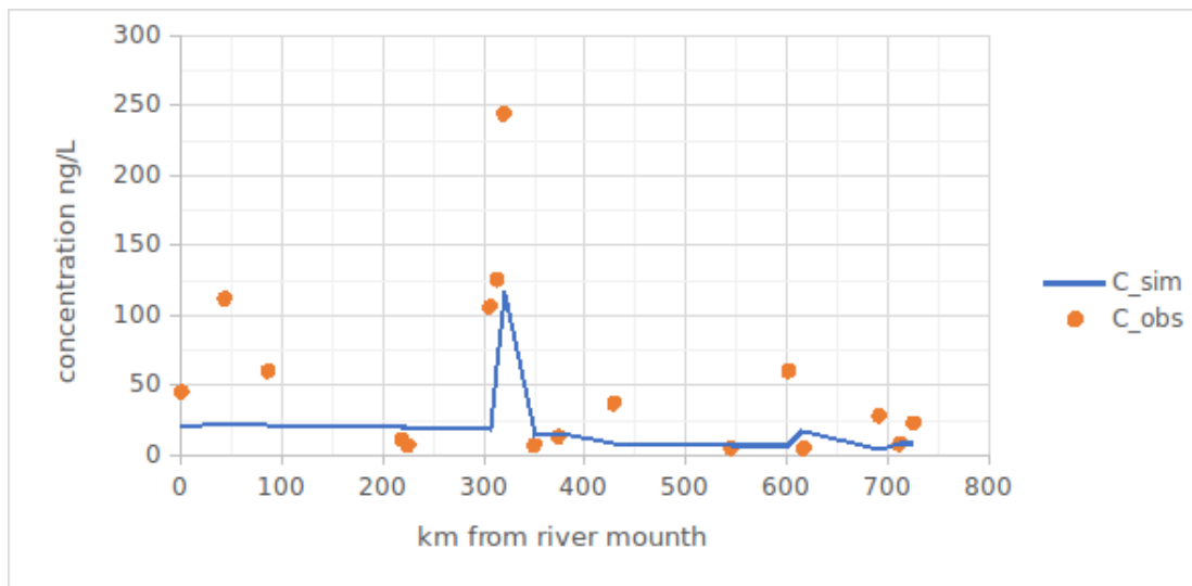
Fig. 1. Example of simulation along the Rhine river
