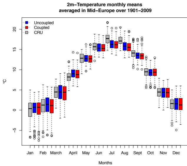
Figure 12: Boxplots showing the annual cycle during the 20 th century of the 2m-Temperature monthly means averaged over Mid-Europe for the CRU observations (grey), uncoupled system (blue) and coupled system (red) (a) and the annual cycle of the model errors compared to CRU observations over Mid-Europe (b).
