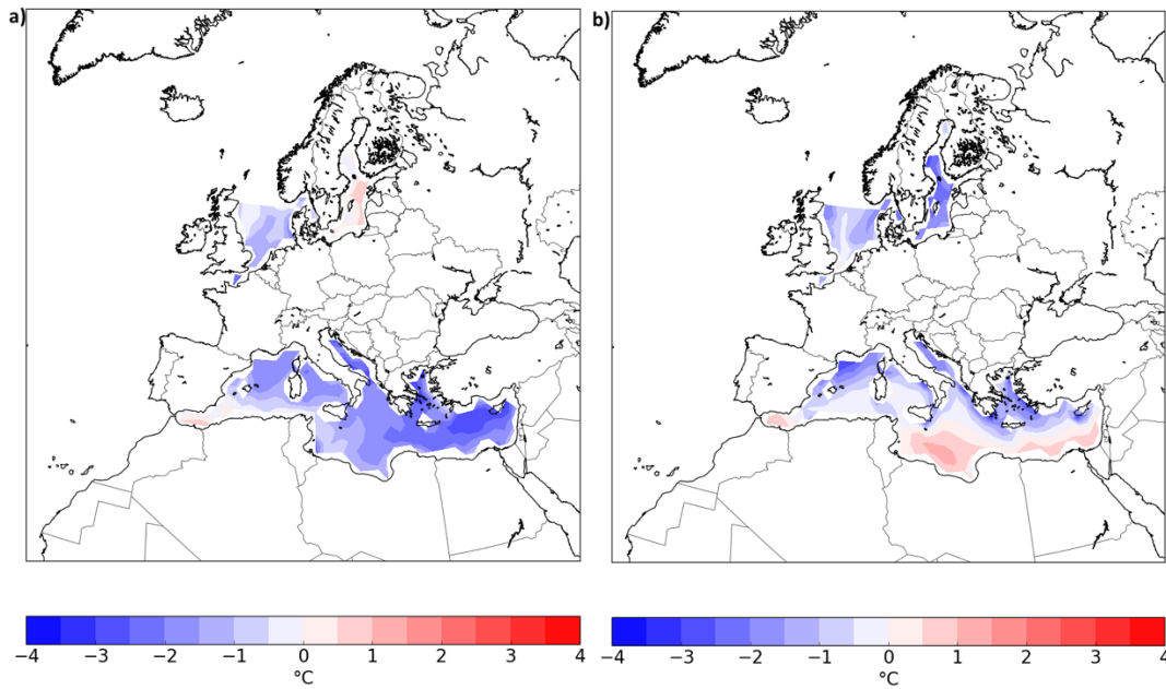
Figure 7: a) Winter and b) summer SST spatial distribution difference between the coupled simulation and the observation.
