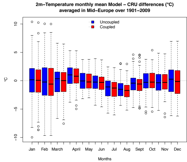
Figure 12: Boxplots showing the annual cycle during the 20 th century of the 2m-Temperature monthly means averaged over Mid-Europe for the CRU observations (grey), uncoupled system (blue) and coupled system (red) (a) and the annual cycle of the model errors compared to CRU observations over Mid-Europe (b).
