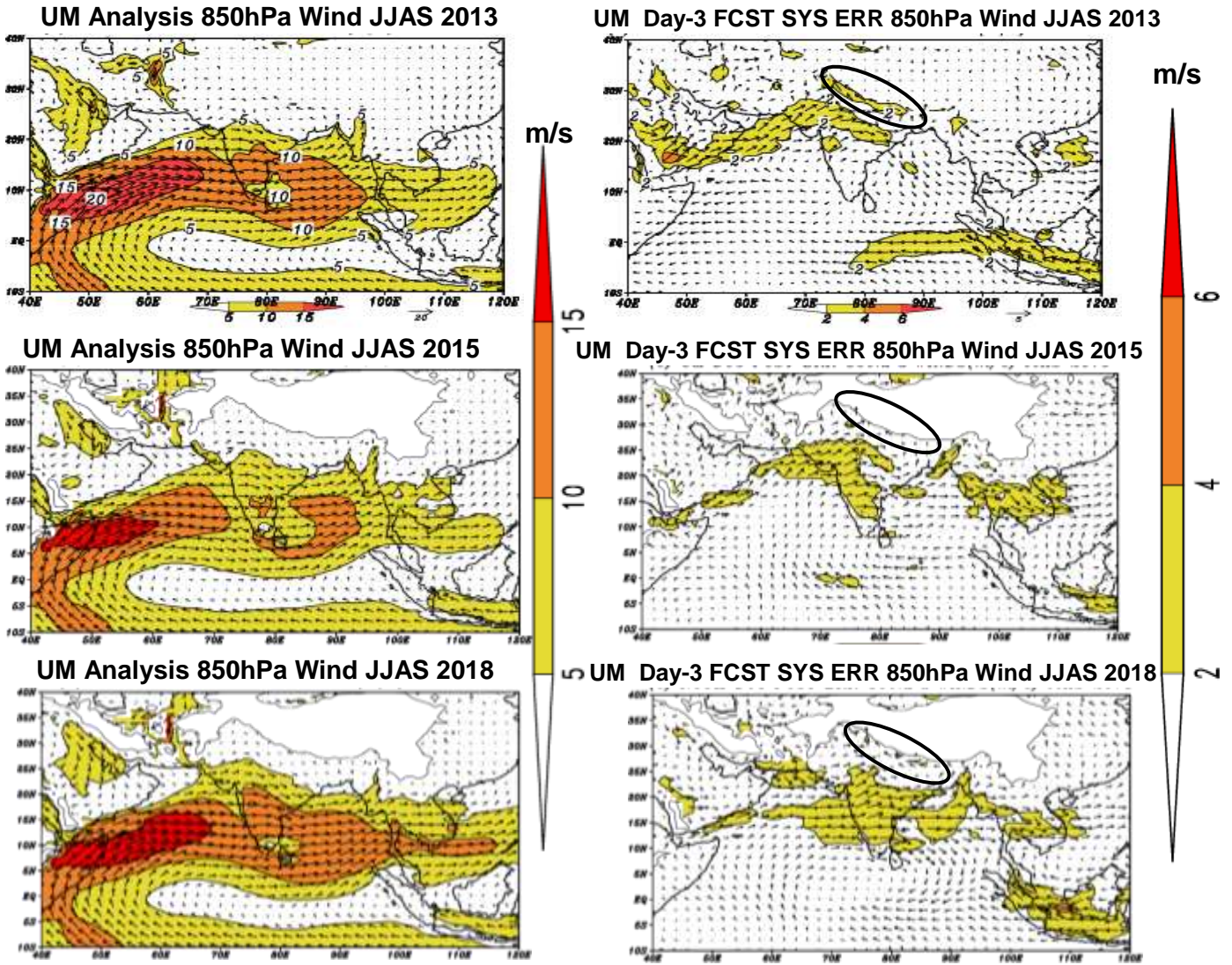
Figure S2 . UM analysis of wind at 850hPa (left panel) and Systematic Error (right panel) in m/s over India during JJAS 2013, 2015 and 2018.
