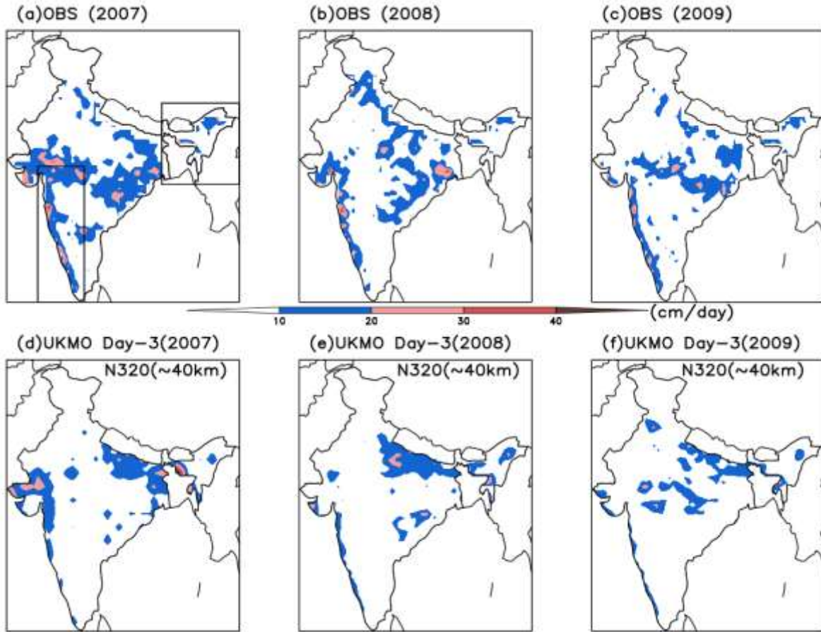
Figure S6. Observed (upper panel) and UM Day-3 highest rainfall Forecast (lower panel) at each grid point during JJAS 2007 , 2008 and 2009 over india
