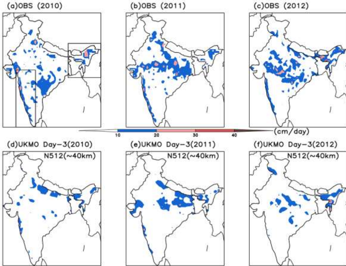
Figure S7. Observed (upper panel) and UM Day-3 highest rainfall Forecast (lower panel) at each grid point during JJAS 2010 , 2011 and 2012 over India
