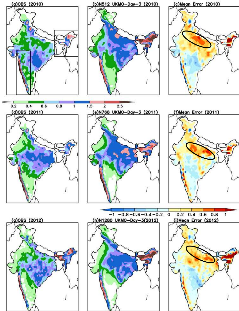
Figure S4. Observed (left panel), Day-3 Forecast mean rainfall (middle panel) and Mean Error (right panel) in \text{cm day}^{-1} over India during JJAS 2010, 2011 and 2012.
