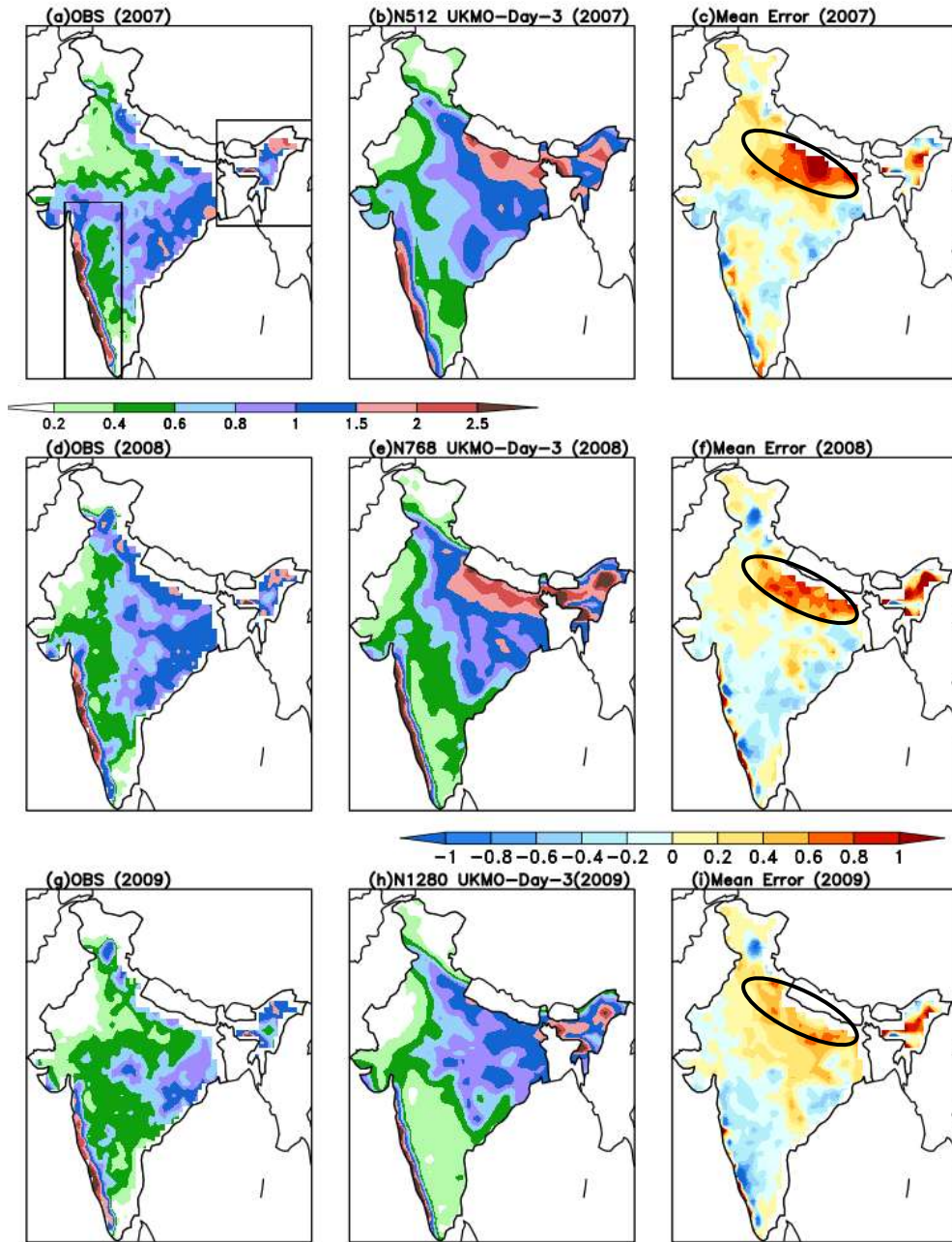
Figure S3. Observed (left panel), Day-3 Forecast mean rainfall (middle panel) and Mean Error (right panel) in \text{cm day}^{-1} over India during JJAS 2007, 2008 and 2009.
