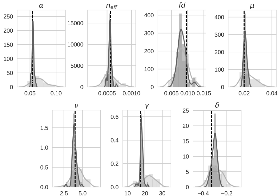
Figure 6. 4DnVar twin distributions for the 7 optimised parameters for both the prior ensemble (light grey) and posterior ensemble (dark grey). The value of the model truth is shown as a dashed vertical black line.
