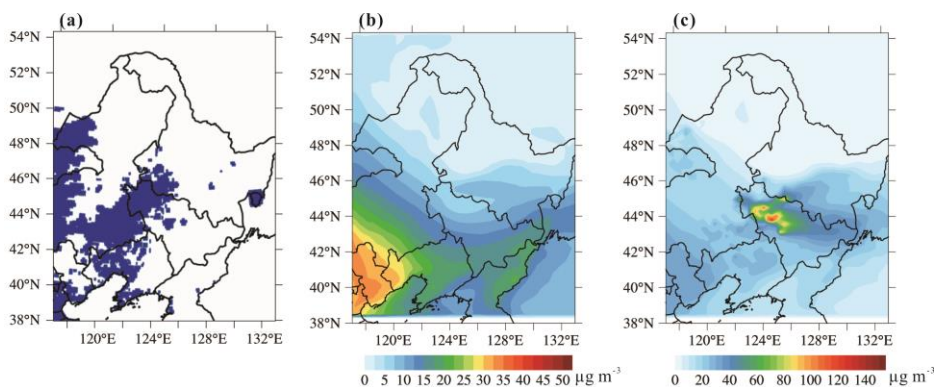
Figure 9. The substituted dust mask (a) and daily mean \text{PM}_{10} distributions with (b) and without (c) friction velocity limitation in NEC on May 5th, 2015.
