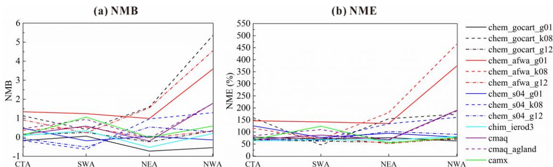
Figure 11. Normalized mean simulation bias (a) and error (b) relative to measurements of PM_{10} during the dust period in the four regions of NEC shown in Fig. 2 (these are CTA, SWA, NEA and NWA). Simulation labels follow Figure 9.
