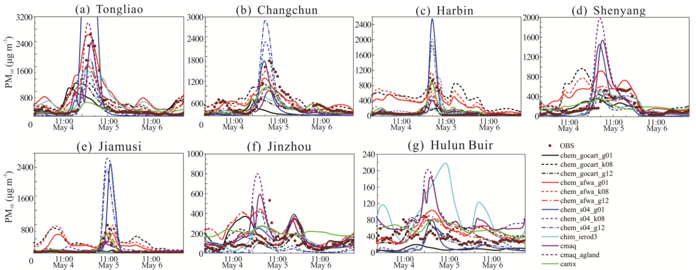
Figure 12. Time series (UTC) of hourly PM_{10} for the simulations and measurements at 4 central sites (Tongliao (a), Changchun (b), Harbin (c) and Shenyang (d)); 1 NE site, Jiamusi (e); 1 SW site, Jinzhou (f); and 1 NW site, Hulun Buir (g) between May 4th and May 6th, 2015. Simulation labels follow Figure 10.
