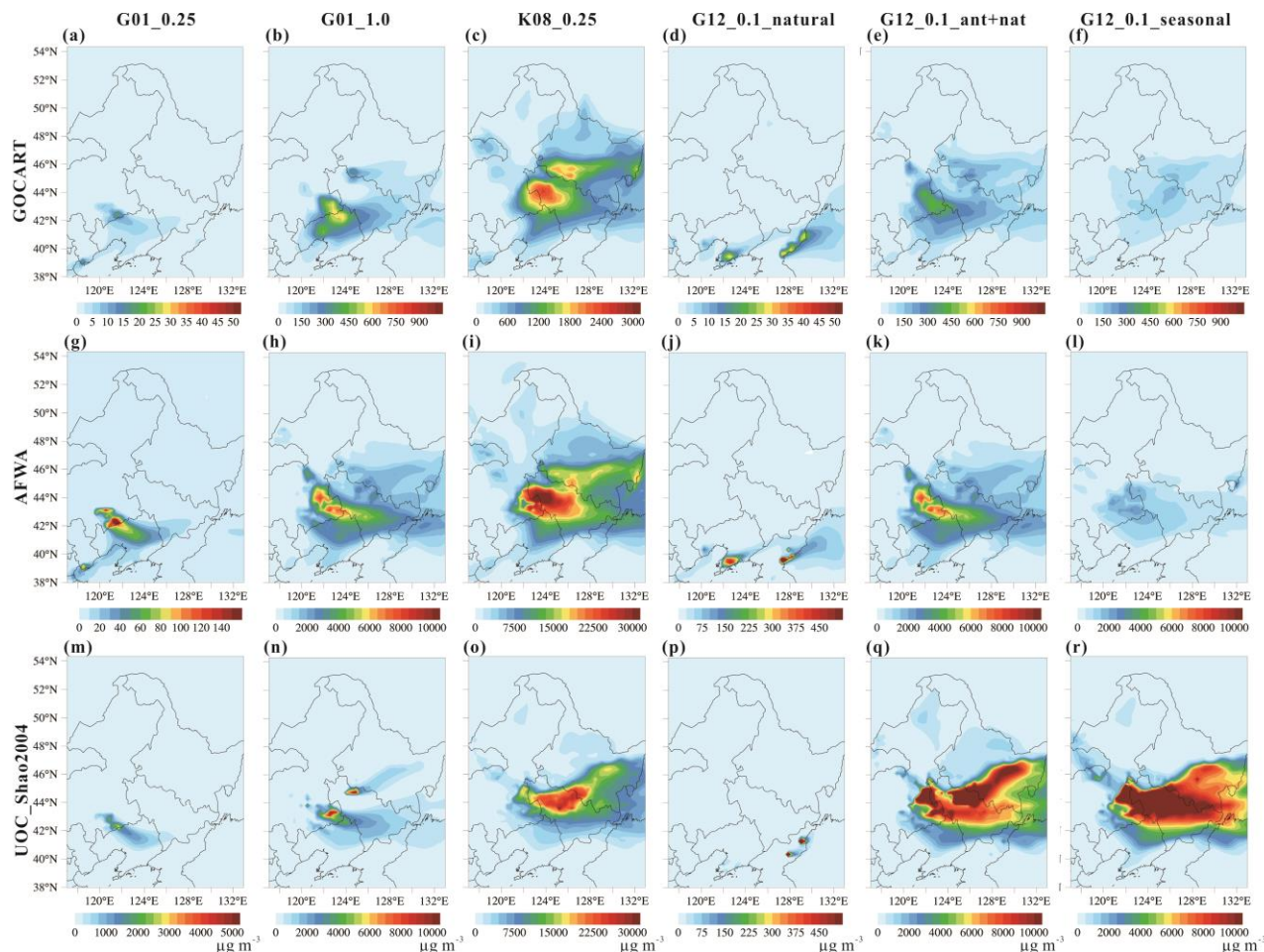
5 Figure 5. Daily mean PM 10 distributions in NEC on May 5th, 2015 using GOCART, AFWA and UOC_Shao2004 with each source map. (a)–(e): GOCART, (g)–(l): AFWA, (m)–(r): UOC_Shao2004.
