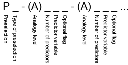
Figure 2. Proposed structure for naming nomenclature to describe the parameterizations of the AM structure.
