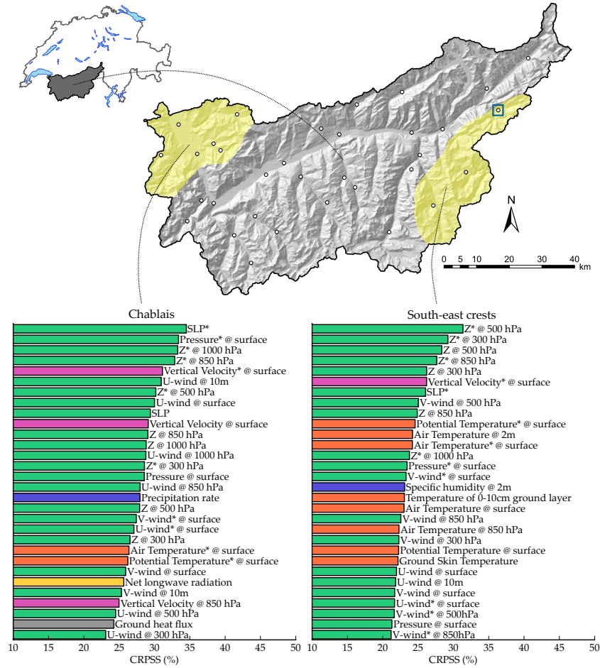
Figure 1. Performance score (CRPSS; Eq. 3; the reference being the climatological precipitation distribution) of the 30 best variables from the NCEP/NCAR reanalysis-NR-1 dataset, when considered separately (no combination), for the Chablais region and the southeast ridges in the upper Rhône catchment in Switzerland. The analogy criterion is S1 when there is an asterisk is present next to the variable name, and RMSE otherwise. Colour illustrates the variable type: green = atmospheric circulation, blue = moisture, orange = temperature, yellow = radiation, purple = vertical velocity, and gray = other. SLP stands for sea level pressure and Z for geopotential height. The blue square indicates the Binn station, which is analyzed in more detail later on.
