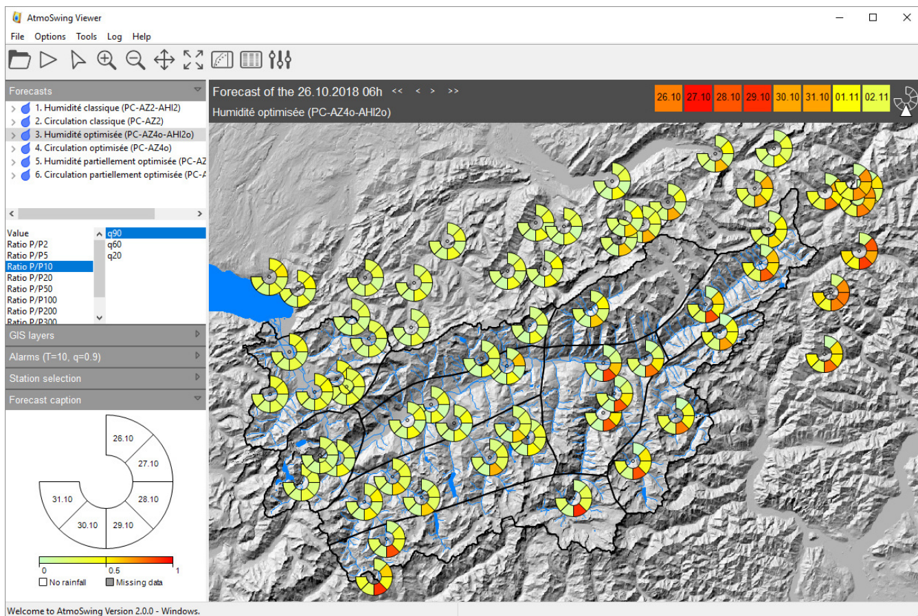
Figure 5. Visualization of Same as Fig. 4 but for multiple lead times on the map (Elevation data from the SRTM, and hydrological network from SwissTopo).
