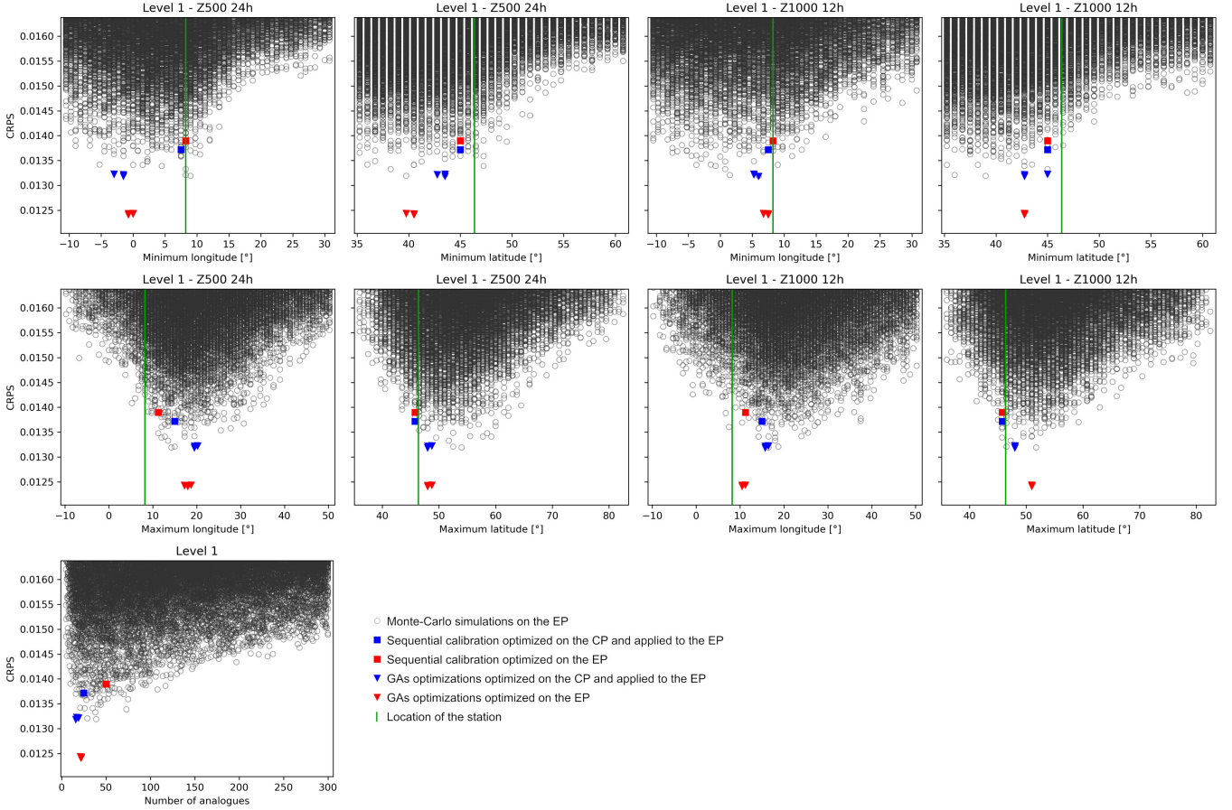
Figure 8. Example of parameter values for 2Z (Table 2) for the precipitation at the Binn station (Fig. 1) on the period-2001–2010 EP . The parameters are the extent (min/max longitude/latitude) of the spatial windows for the geopotential height at 500 and 1000 hPa, and the number of analogs. The green vertical bar in the plots represents the location of the station. The circles represent random parameters from the Monte–Carlo analysis. The plots are truncated at the 25 th best percentiles for 50,000 realizations. Squares are the results of the sequential calibration and triangles result from genetic algorithms. Markers in blue represent parameters optimized for the period-1981–2000 CP and applied to 2001–2010 EP . Markers in red represent parameters optimized directly for the period-2001–2010 EP .
