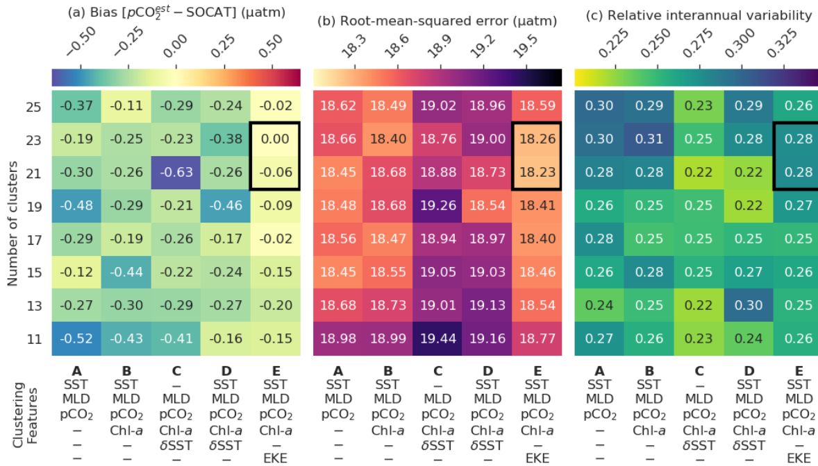
Figure 5: Heatmaps showing the average cluster (a) bias, (b) root-mean-squared error (RMSE) and (c) relative interannual variability ( R_{iav} ) for different cluster configurations, where smaller scores are better for all metrics. The rows show the number of clusters, and the columns show clustering feature-variable configurations. Each cluster contains the average of the scores for four regression methods: support vector regression, extremely randomised trees, gradient boosting machine, and feed-forward neural network. The black box indicates clustering configurations that perform well across all metrics – note that a R_{iav} < 0.3 falls within the best category of performance in Rödenbeck et al. (2015).
