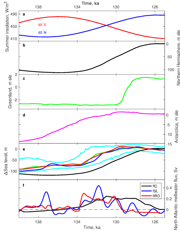
Figure 4. Timeseries of a) Summer solstice insolation at 65°N and 65°S, b-d) global sea level equivalent (m) of changes in b) NH (Abe-Ouchi et al., 2013), c) Greenland (Tarasov et al., 2012) and d) Antarctic ice-sheets (Briggs et al., 2014), e) global sea level (m) change estimated from Red Sea records (Grant et al., 2014) (green) with the 95% probability interval (cyan), sea-level record with an adjusted age scale as described in section 5 (blue), and as estimated from the continental ice-sheets simulations (black). The red line shows the changes in global sea-level that would be obtained by adding the meltwater flux, f_{IRD} , described in f plus an Antarctic contribution of 13 m. f) Possible North Atlantic meltwater flux (Sv) scenarios: estimated from the disintegration of NH ice-sheets as shown in b, c (Tarasov et al., 2012; Abe-Ouchi et al., 2013) (black), estimated from the global sea-level change on the revised age-scale (this study, blue), and scaled from the North Atlantic and Norwegian Sea IRD records (red, shown in Fig. 8b).
