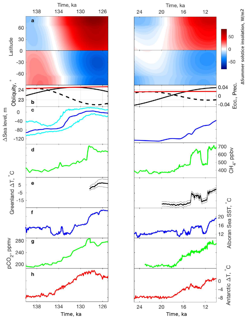
Figure 1. Overview of (left) the penultimate and (right) the last deglaciations climatic and environmental evolutions: a) Hovmöller diagram of summer solstice insolation anomalies ( \text{W/m}^2 ). This corresponds to June 21st in the Northern Hemisphere and December 21st in the Southern Hemisphere; Timeseries of b) eccentricity (red), obliquity (solid black) and precession (dashed black) (Berger, 1978); c) Global mean sea level anomaly probability maximum (m, blue), (left) including its 95% confidence interval (cyan) (Grant et al., 2014), from Grant et al. (2012) on the original age model for the penultimate and (right) from Lambeck et al. (2014) for the last deglaciation. d) Atmospheric methane ( \text{CH}_4 ) concentration as recorded in EDC ice core, Antarctica (Loulergue et al., 2008); e) Precipitation-weighted surface temperature reconstruction based on stable water isotopes from the Greenland NEEM ice core (left), and annual surface temperature composite reconstruction based on air nitrogen isotopes from the Greenland NEEM, NGRIP and GISP2 ice cores (Buizert et al., 2014); f) Alkenone-based ( \text{Uk}'_{37} ) SST reconstruction from ODP976 (Martrat et al., 2014); g) Atmospheric \text{CO}_2 concentration as recorded in Antarctic ice cores (left) EDC (Bereiter et al., 2015) and (right) WAIS divide (Marcott et al., 2014) on the WD2014 chronology (Buizert et al., 2015); h) Antarctic temperature anomalies relative to present day inferred from EDC ice core (Jouzel et al., 2007). Unless specified differently, all records are displayed on the AICC2012 timescale (Bazin et al., 2013; Veres et al., 2013) or a chronology coherent with AICC2012.
