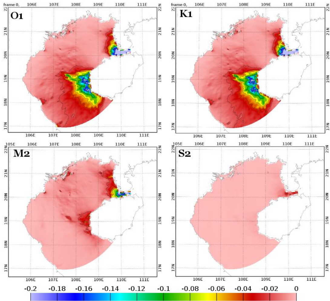
1530 Figure 14: Bottom dissipation flux ( W m^{-2} ) for O1, K1, M2 and S2 computed from model outputs of simulation "TEST 6".
