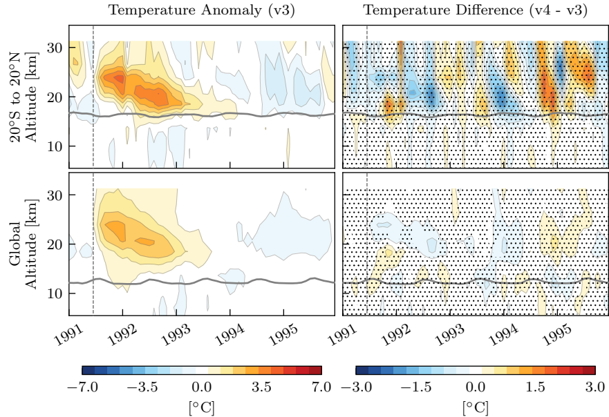
Figure S1: Same as Figure 5, except using data from EAMv1 ran in AMIP mode.
