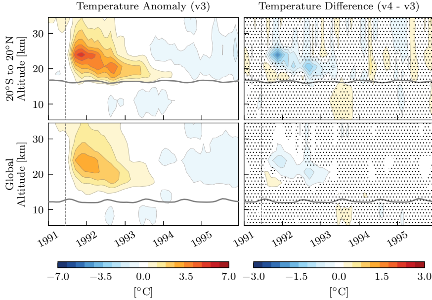
Figure 5. The left column shows the monthly temperature anomalies averaged over all CanESM5 ensemble members with version 3 forcing for 20^{\circ}\text{S} to 20^{\circ}\text{N} (top) and the global average (bottom). The right column shows the difference in temperature when using the version 3 and version 4 datasets. Stippling marks the regions where differences are not significantly different from zero at the 95% confidence level. Anomalies are computed using the simulation period of 1990 through 1999.
