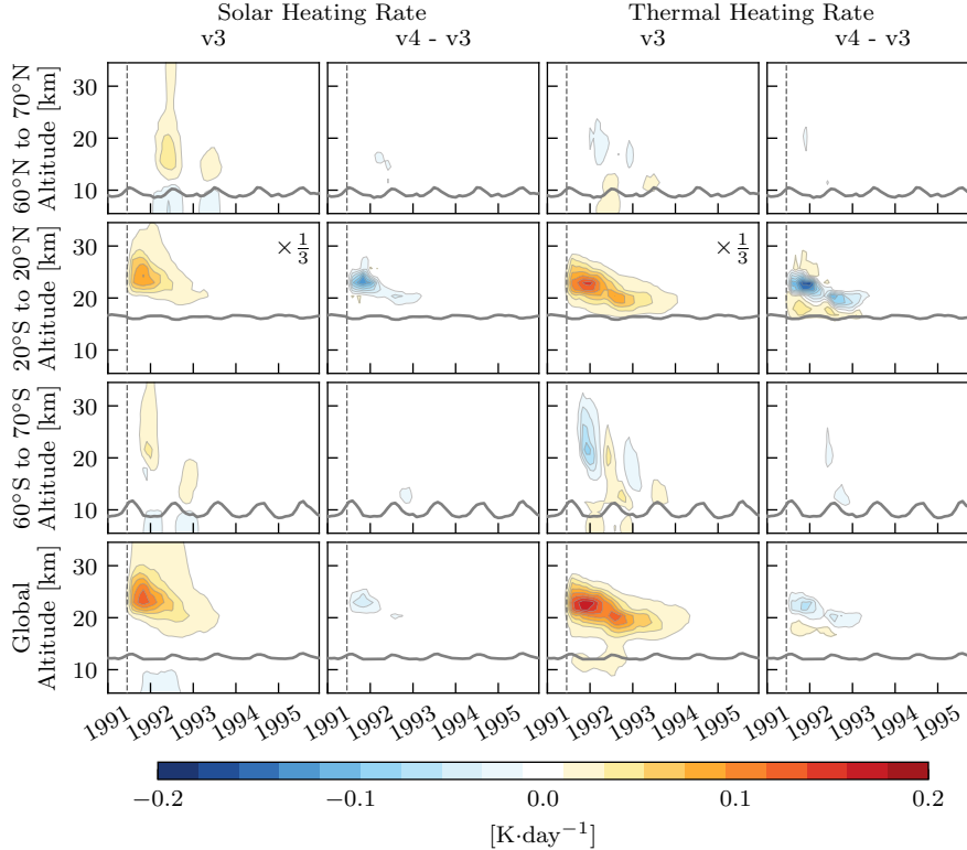
Figure 4. Instantaneous heating rates from CanESM5 model runs. The left column shows the instantaneous solar heating rate due to stratospheric aerosols using the version 3 forcing dataset. The second column shows the change in the instantaneous solar heating rate when version 4 is used instead. The third and fourth columns show the same, except for the instantaneous thermal heating rates. The gray lines denote the tropopause, and dashed lines indicate the date of the Pinatubo eruption. Note that the v3 instantaneous heating rates in the tropics have been multiplied by 1/3 for visual representation.
