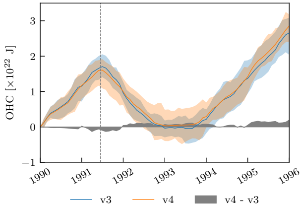
Figure 8. Monthly deseasonalized ocean heat content relative to January 1990. The blue line shows OHC using the version 3 aerosol forcing while the orange line indicates results when using version 4. The shading indicates the 10 th and 90 th percentiles of the data.
