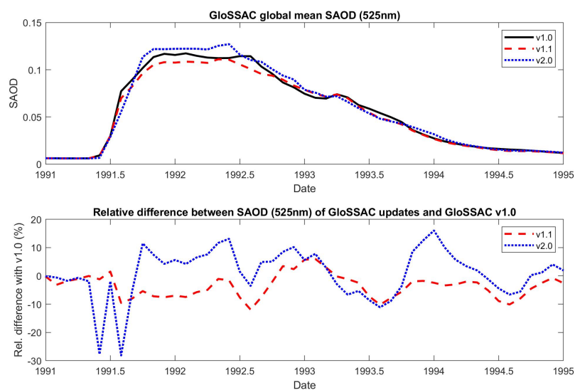
Fig. 1. Post-Pinatubo SAOD in GloSSAC 1.0, 1.1 and 2.0
