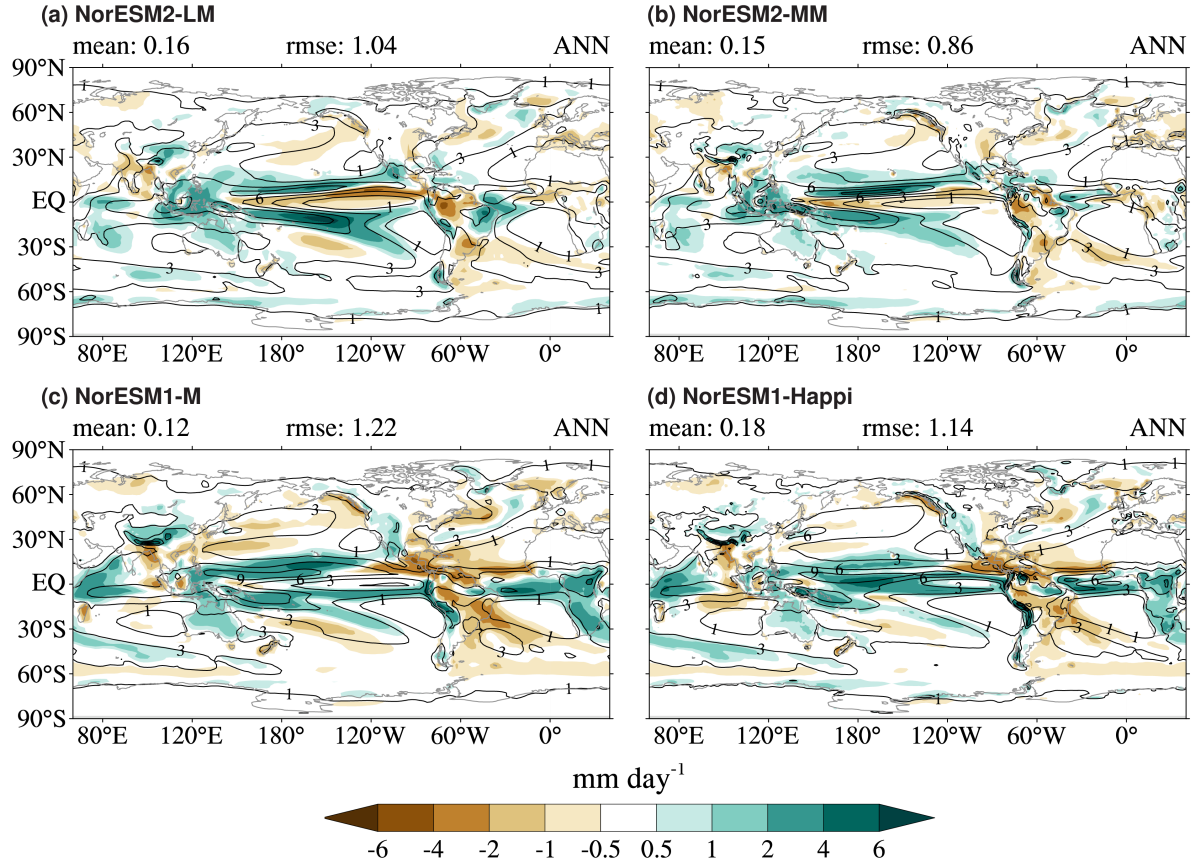
Figure 19. Annual-mean ensemble-mean model bias for total precipitation rate (colors) shown with the present-day model climatology (solid black contours; values from 1 \text{ mm day}^{-1} by 2 \text{ mm day}^{-1} ) from NorESM2-LM (a; years 1980–2009), NorESM2-MM (b; years 1980–2009), NorESM1-M (c; years 1976–2005), and NorESM1-Happi (d; years 1976–2005). Three ensemble members are used for all model versions. The bias is taken with respect to GPCP (years 1979–2008 for NorESM1-M/Happi and 1980–2009 for NorESM2-LM/MM). Units are \text{mm day}^{-1} .
