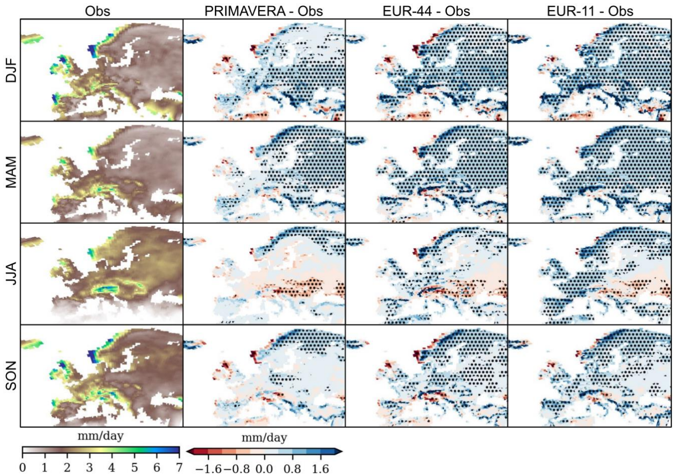
Figure 4: Mean precipitation from the combination of observational datasets (first column), and mean precipitation bias between PRIMAVERA and observations (second column), EUR-44 and observations (third column), and EUR-11 and observations (last column). Results for the different seasons are shown in rows. Dots show regions where mean bias is statistically significant at the 10% level. All datasets are shown on the EUR-44 grid.
