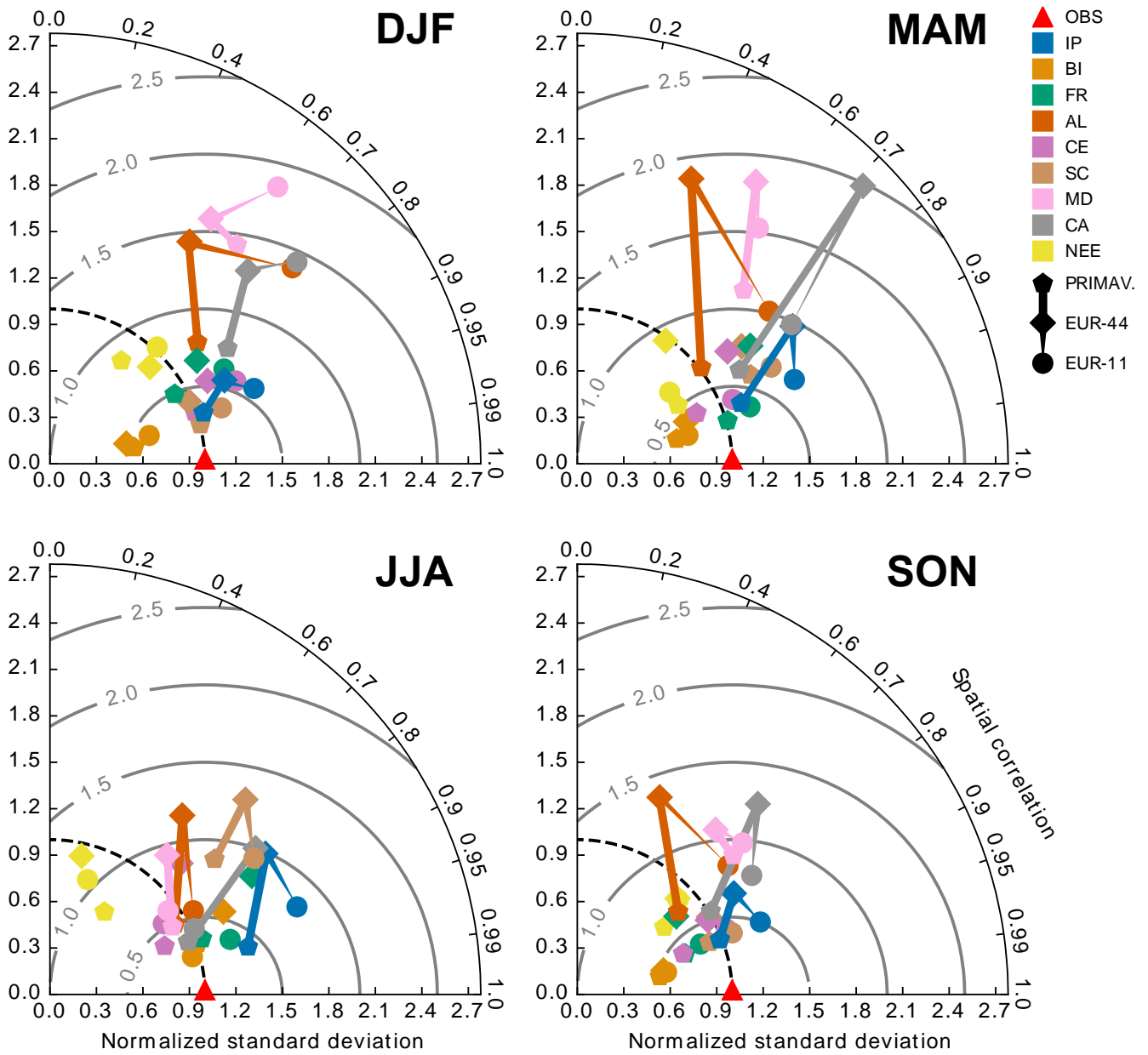
Figure 5: Taylor diagrams performed on the spatial distributions of seasonal mean precipitation for EUR-11 (circles), EUR-44 (diamonds) and PRIMAVERA (pentagons) ensemble means for DJF (top left), MAM (top right), JJA (bottom left), SON (bottom right) over all regions. Symbols are connected (see legend) for complex-orography and coastal regions (AL, CA, IP, MD, SC). Observational references are shown in red triangles.
