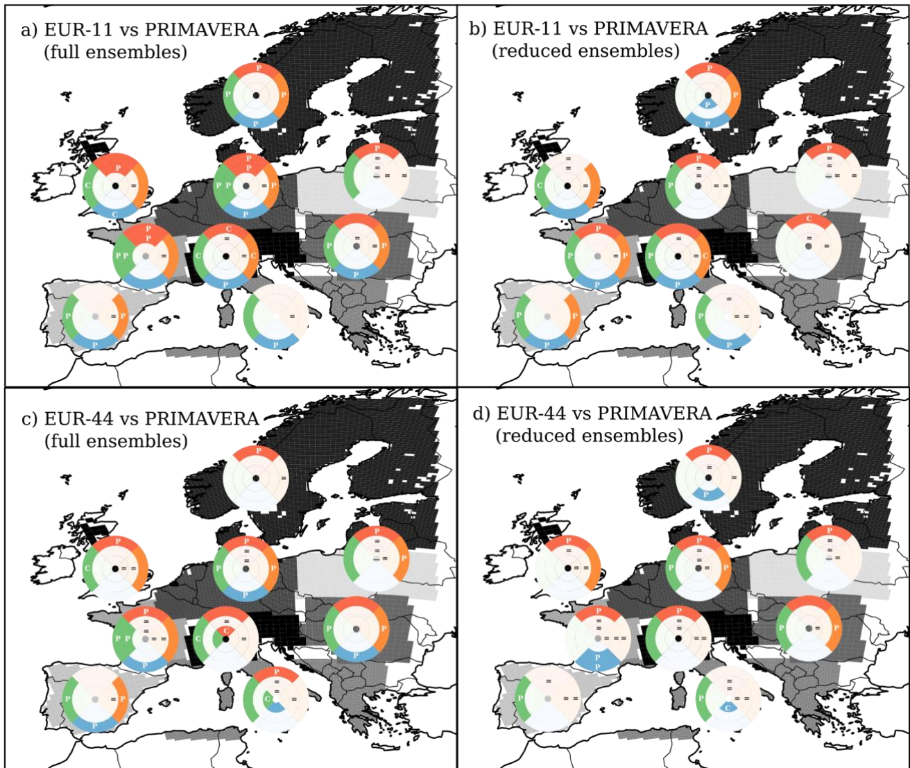
Figure 8: Map using the method described in Fig. 1: for each region, season (clockwise from the top: summer, autumn, winter, spring; see right panel of Fig. 1), and precipitation intensity interval: low precipitation rates (inner part), moderate precipitation rates (middle part), high precipitation rates (outer part), a colour indicates that CORDEX and PRIMAVERA are significantly different, a “P” or “C” letter indicates that PRIMAVERA or CORDEX is closer to observations, respectively, an “=” sign indicates that both ensembles are close to observations. a) Map for the full PRIMAVERA and EUR-11 ensembles (listed in Tables 1 and 2); b) Map with reduced PRIMAVERA and EUR-11 ensembles using GCMs of the same family (coloured in Tables 1 and 2); c) Map for the full PRIMAVERA and EUR-44 ensembles (listed in Tables 1 and 2); d) Map with reduced PRIMAVERA and EUR-44 ensembles using GCMs of the same family (coloured in Tables 1 and 2).
