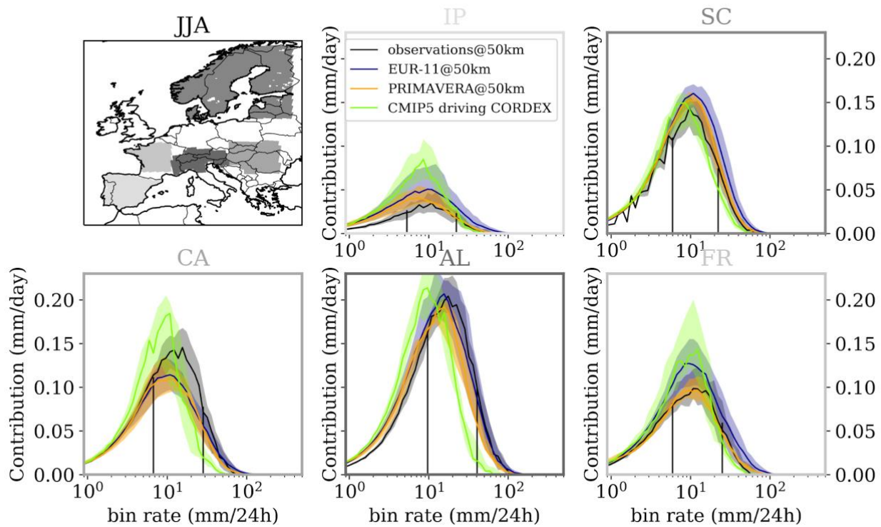
Figure 3: As Fig. 2 for summer (JJA).
