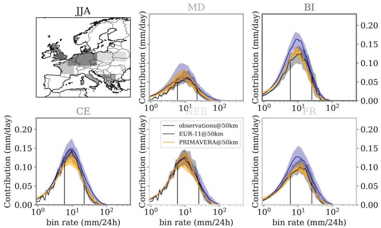
Figure 7: Same as Fig. 6 for JJA.
