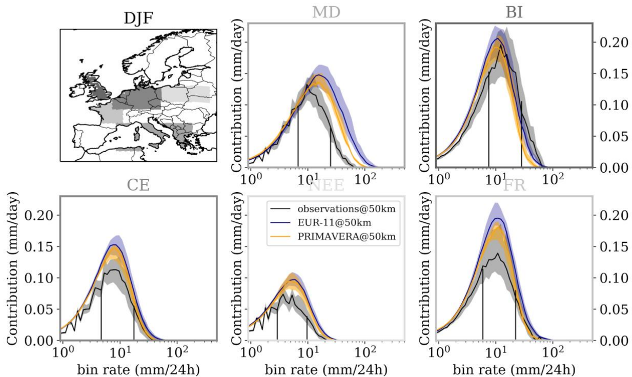
Figure 6: Precipitation contribution (frequency x bin rate) per precipitation rate in DJF over the Mediterranean (MD), British Isles (BI), Central Europe (CE), North East Europe (NEE), France (FR) for EUR-11 (blue), PRIMAVERA (orange), and observations (black) regridded on EUR-44.
