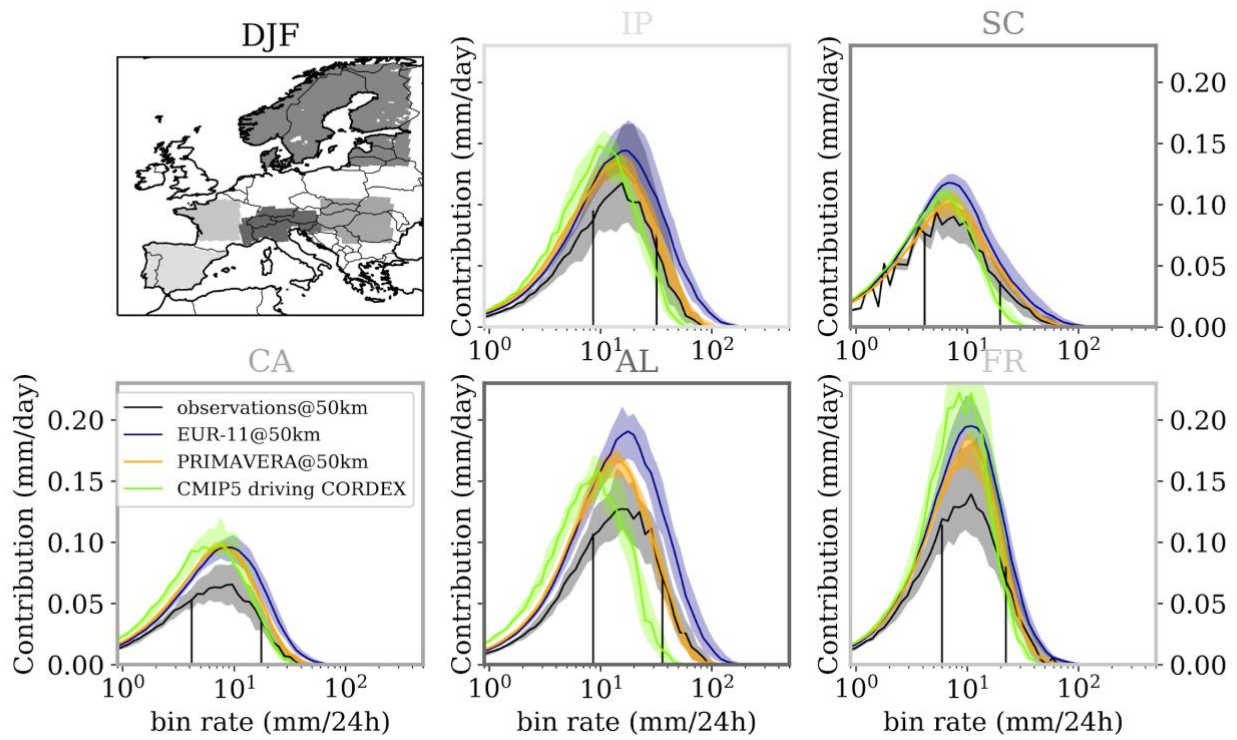
Figure 2: Precipitation contribution (frequency x bin rate) per precipitation rate in DJF over the Iberian Peninsula (IP), Scandinavia (SC), the Carpathian region (CA), the Alps (AL), and France (FR), for a selection of CMIP5 GCMs (green), PRIMAVERA (orange), EUR-11 (blue). CMIP5 data are plotted on the models native grid, the other datasets are regridded on a common EUR-44 grid.
