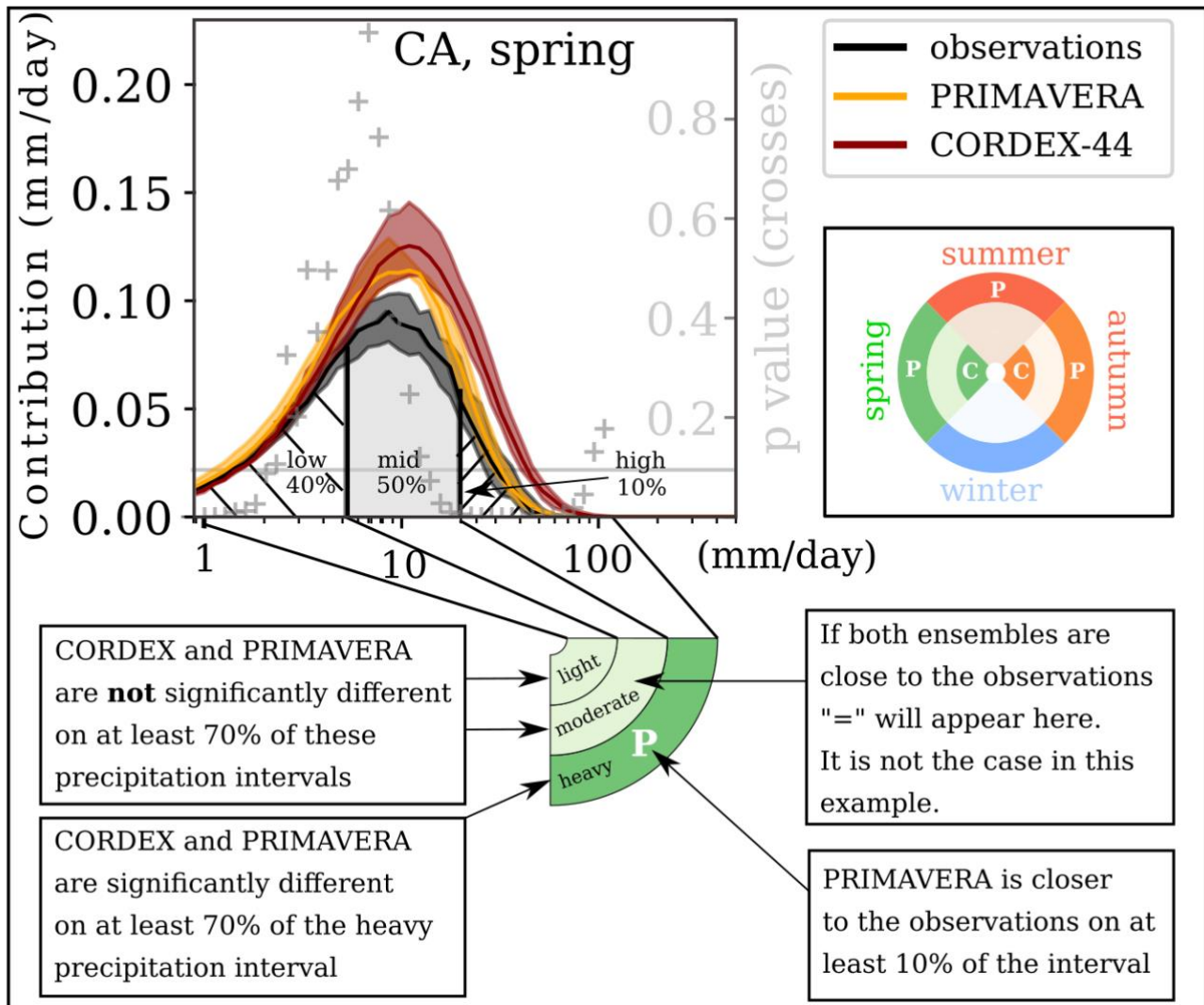
Figure 1: Explanation of the method:(top) Daily precipitation contribution to mean precipitation (precipitation frequency x bin intensity) using exponential bins in the Carpathian region (CA) in spring (MAM) for PRIMAVERA, EUR-44 and observations. The thick lines show the ensemble median, the model spread is calculated on the inter-quartile range of the inter-member spread, and the observation spread is based on inter-annual values. Grey crosses are p -values of the PRIMAVERA versus CORDEX difference using a Student's t -test, the ensembles are significantly different where the crosses are below 0.1. (bottom) For three precipitation intensity intervals (light: accounting for lowest 40% of mean precipitation, moderate: accounting for the next 50% of the mean, heavy: accounting for highest 10% of the mean), a pie is coloured if the ensembles differ on more than 70% of the interval. Letters show which ensemble is closest to observations ('P' for PRIMAVERA, 'C' for CORDEX; no colour indicates that none of the ensembles are close to observations, '=' indicates that both ensembles are close to observations). (right) Resulting pie for each region (here CA) and season.
