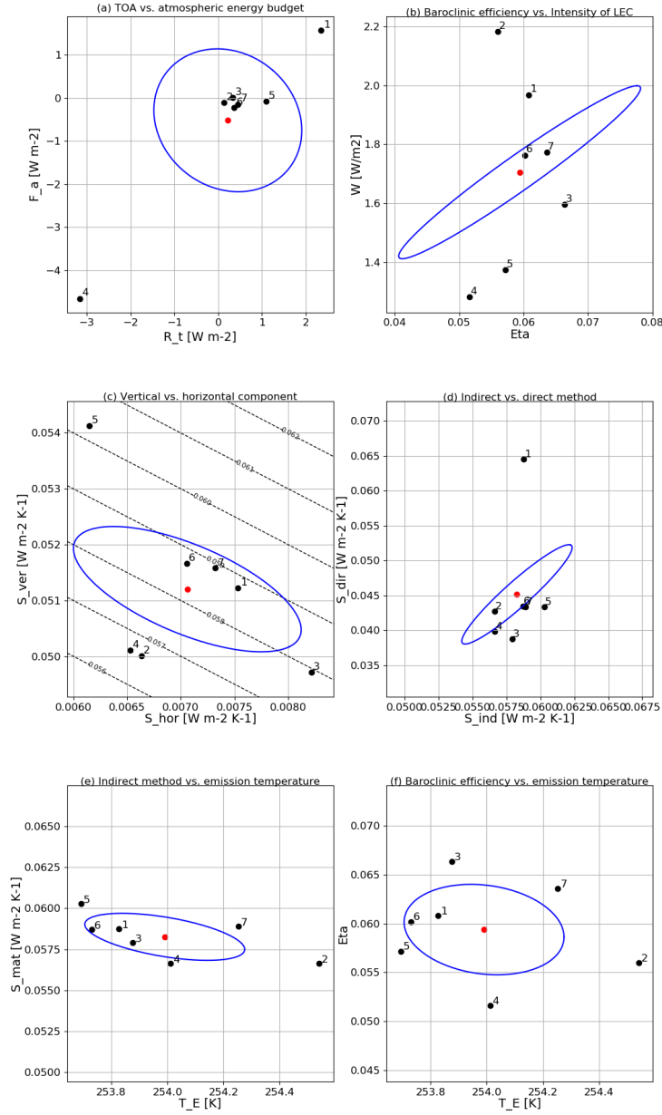
Figure 10. Multi-model ensemble scatter plots from piC scenario for: (a) Atmospheric energy budget vs. TOA energy budget (both in \text{W/m}^2 ), (b) Baroclinic efficiency vs. LEC intensity (in \text{W/m}^2 ), (c) vertical component of the material entropy production vs. vertical component (together with iso-lines of total material entropy production with the indirect method) (in \text{W/m}^2 \cdot \text{K} ), (d) Direct vs. indirect method for material entropy production (in \text{W/m}^2 \cdot \text{K} ). Blue ellipses denote the \sigma standard deviation of the multi-model mean (denoted by the red dot). Model IDs are: 1. BNU, 2. Can2, 3. IPSL-M, 4. MIR5, 5. MIR-C, 6. MPI-LR, 7. MPI-MR.
