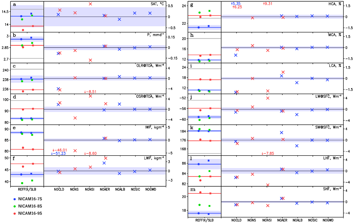
Figure 5: Global annual means of surface air temperature (a), precipitation (b), top-of-atmosphere (TOA) outgoing longwave radiation (OLR) (c), TOA outgoing shortwave radiation (OSR) (d), ice water path (e), liquid water path (f), high cloud amount (g), middle cloud amount (h), low cloud amount (i), surface net downward longwave radiation (j), surface net downward shortwave radiation (k), surface latent heat flux (l), and surface sensible heat flux (m). They are averaged over June 2004–May 2005, and their units are shown at the upper-right corner of each panel. Blue shading shows the interannual variability ( 2\sigma , detrended) estimated from the HighResMIP NICAM16-7S run over 1950–2050 (Table 1). In the left part of each panel contains plots of global annual means simulated by NICAM16-7S (56-km mesh; blue), NICAM16-8S (28-km mesh; green), and NICAM16-9S (14-km mesh; red), which were performed under the fixed SST condition (filled circles; REFFIX run in Table 2) and with the slab ocean condition (filled squares; REFFSLB run in Table 2). Blue and red lines are the reference (REF) runs with 56-km mesh and 14-km mesh, respectively. Observational values taken from the JRA-55 reanalysis (surface air temperature), GPCP (precipitation), CERES (radiation), and ISCCP (cloud amount) are shown as gray lines. The right part of each panel shows differences between the REF run and each sensitivity run (NOCLD, NONS, NONSI, NOAER, NOALB, NOSIC, and NOGWD runs in Table 2). simulated by NICAM16-7S (56-km mesh; blue multiplication sign), and NICAM16-9S (14-km mesh; red multiplication sign). Results outside the scale range are shown with digits.
