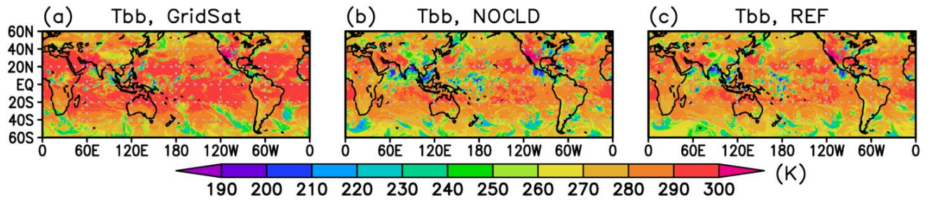
Figure 7: TOA brightness temperature near 11 \mu\text{m} at 00:00 UTC June 6, 2004, from the GridSat product (a) and the NOCLD (b) and REF (c) runs by NICAM16-9S. The display style follows Figure 1 of Roh et al. (2017). Grid interval in (b) and (c) is 0.14°.
