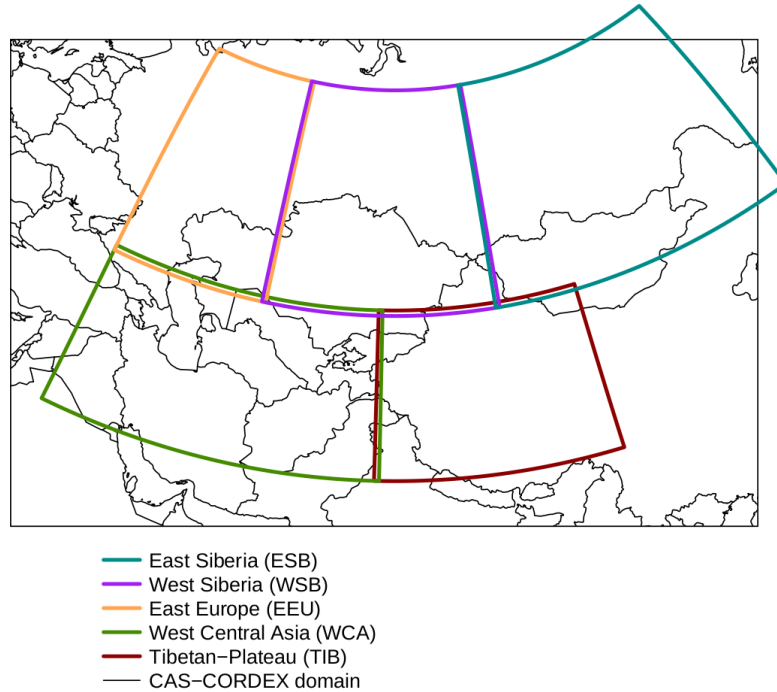
125 Figure 2: IPCC6 subregions projected on the CAS-CORDEX region.
