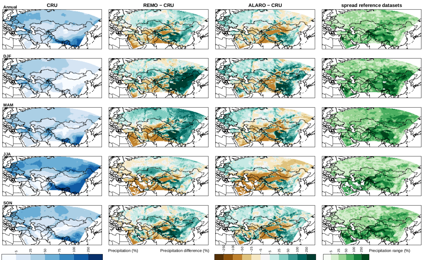
Figure 10: Left column: mean monthly precipitation amounts (mm month -1 ) over the CAS-CORDEX domain based on the observational CRU dataset for the 1980-2017 period on annual level and for winter (DJF), spring (MAM), summer (JJA) and autumn (SON). In the middle columns: relative difference between the average annual and seasonal CRU precipitation and the precipitation simulated by the models (%). Right column: the range in precipitation (%) between the different reference datasets (CRU, MW, GPCP and ERA-Interim).
