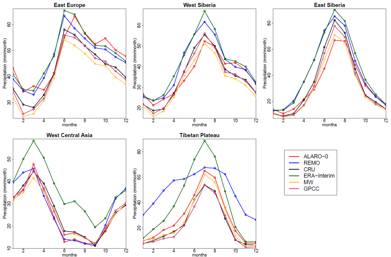
Figure 12: Annual cycles of precipitation (mm/month) for both RCMs (ALARO-0 and REMO) compared to the ERA-Interim reanalysis, MW, GPCC and CRU observational data over five subregions.
