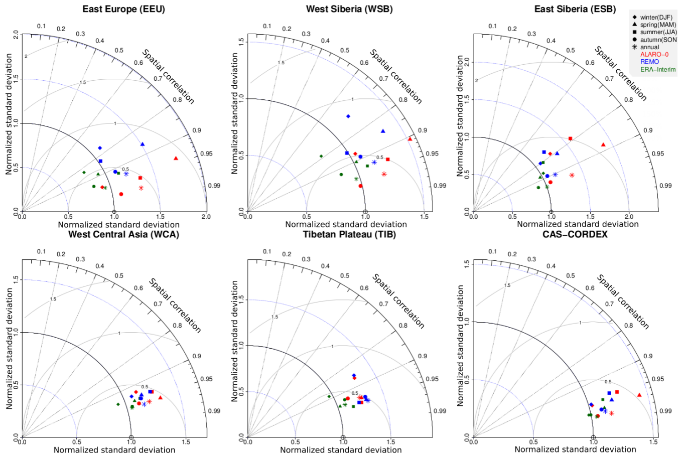
Figure 9: Normalized Taylor diagram expressing the model spatial performance of the maximum temperature for seasonal and annual means for both RCMs (ALARO-0 and REMO) and ERA-Interim reanalysis with respect to CRU for the five subregions and the complete CAS-CORDEX domain.
