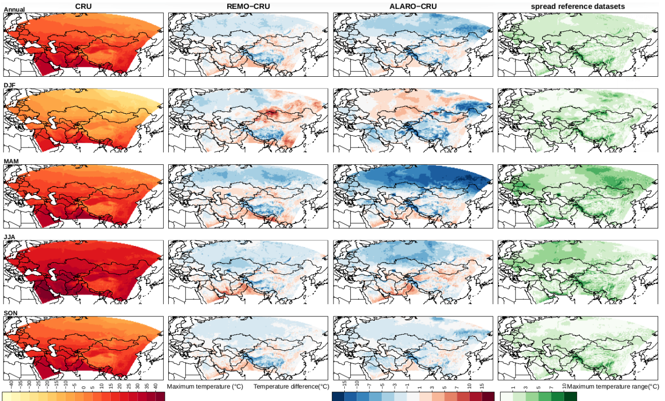
400 Figure 8: Left column: maximum air temperature ( ^{\circ}\text{C} ) at 2 m height over the CAS-CORDEX domain based on the observational CRU dataset for the 1980-2017 period on annual level and for winter (DJF), spring (MAM), summer (JJA) and autumn (SON). In the middle columns: difference in maximum temperature between models and CRU. Right column: the range in maximum temperature ( ^{\circ}\text{C} ) between the different reference datasets (CRU and ERA-Interim).
