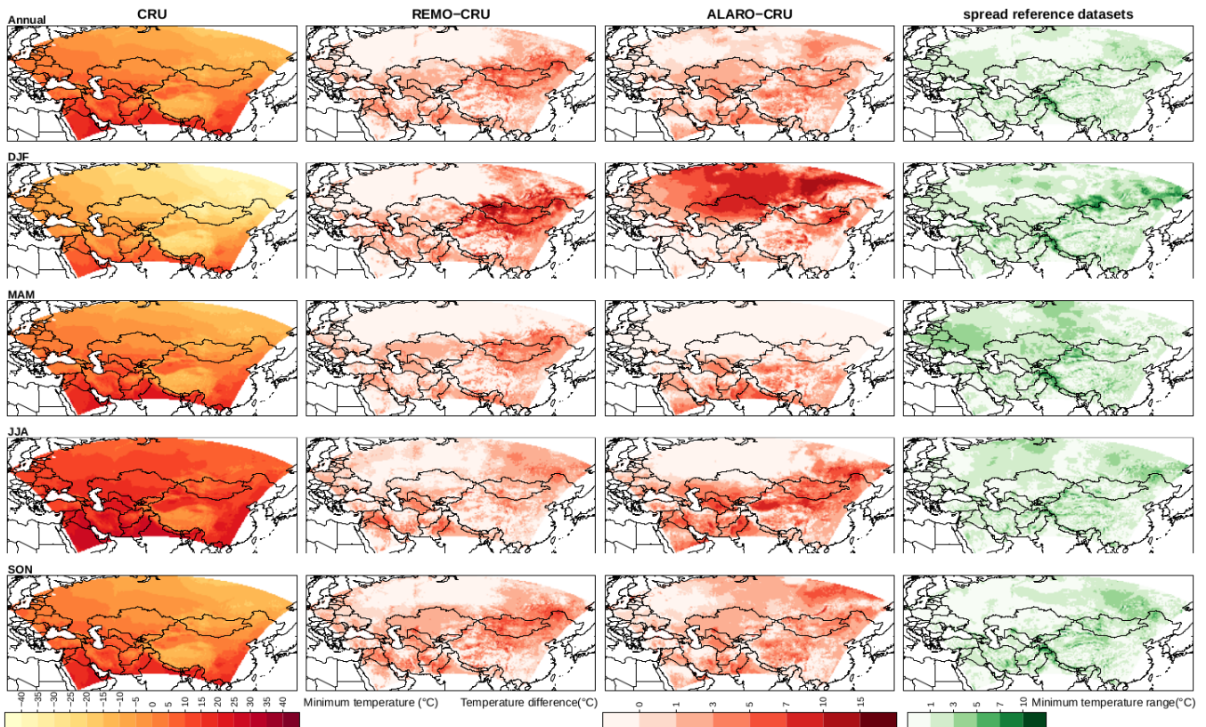
360 Figure 6: Left column: minimum air temperature ( ^{\circ}\text{C} ) at 2 m height over the CAS-CORDEX domain based on the observational CRU dataset for the 1980-2017 period on annual level and for winter (DJF), spring (MAM), summer (JJA) and autumn (SON). In the middle columns: difference in minimum temperature between models and CRU. Right column: the range in minimum temperature ( ^{\circ}\text{C} ) between the different reference datasets (CRU and ERA-Interim).
