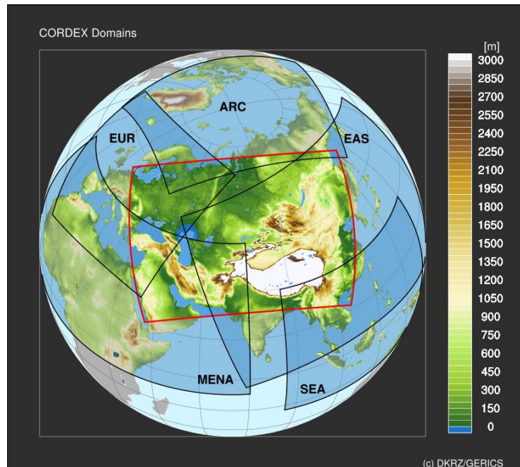
Figure 1: The CAS-CORDEX domain delineated by a red contour and the main overlapping CORDEX domains (black contour lines): Europe (EUR), Arctic (ARC), South East Asia (SEA), East Asia (EAS) and MENA projected upon the topography of Eurasia (geopotential height [m] of the GTOPO30 global digital elevation model (DEM) 3). All points with orography higher than 3000 m are colored white.
