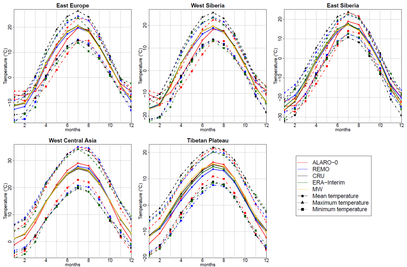
335 Figure 5: Annual cycles of the mean, minimum and maximum temperature for both RCMs (ALARO-0 and REMO) compared to the ERA-Interim reanalysis, MW and CRU observational data over five subregions.
