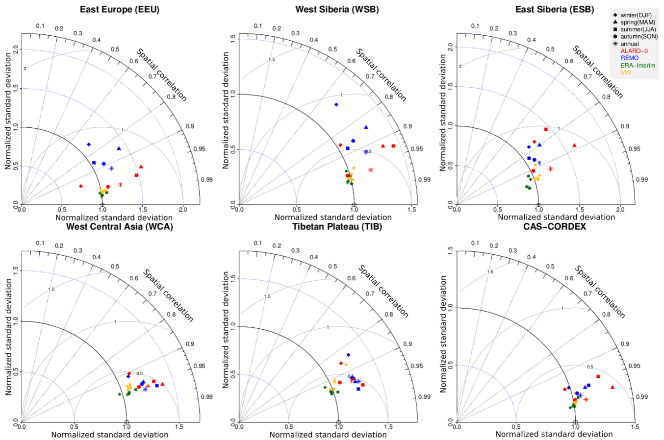
310 Figure 4: Normalized Taylor diagram expressing the spatial performance of mean temperature for seasonal and annual means for both RCMs (ALARO-0 and REMO), the ERA-Interim reanalysis and MW observational data with respect to CRU for the five subregions and the complete CAS-CORDEX domain.
