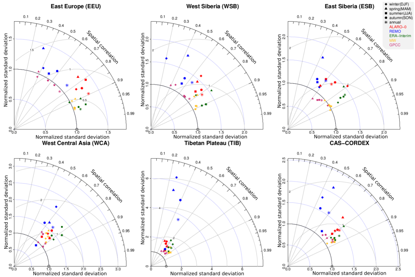
Figure 11: Normalized Taylor diagram expressing the model performance of precipitation for seasonal and annual means for both RCMs (ALARO-0 and REMO), gridded observational datasets (MW, GPCP) and the ERA-Interim reanalysis data with respect to CRU for the five subregions and CAS-CORDEX domain.
