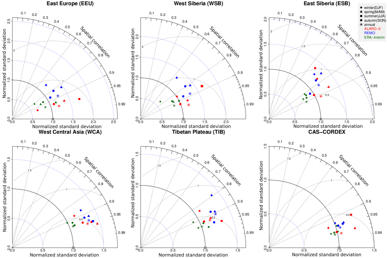
Figure 7: Normalized Taylor diagram expressing the model spatial performance of the minimum temperature for seasonal and annual means for both RCMs (ALARO-0 and REMO) and ERA-Interim reanalysis with respect to CRU for the five subregions and the complete CAS-CORDEX domain.
