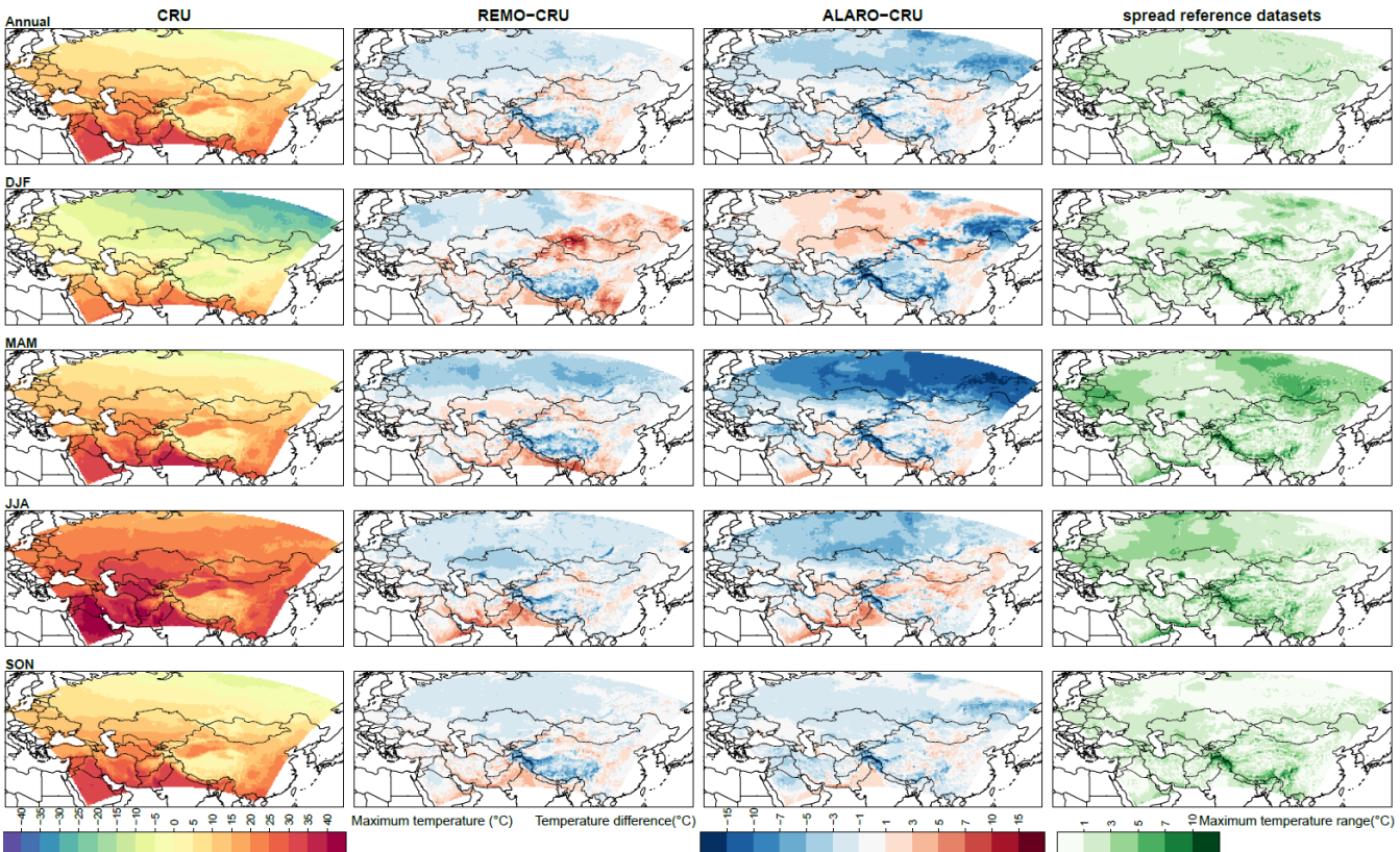
Figure 8: : Left column: maximum air temperature (°C) at 2 m height over the CAS-CORDEX domain based on the observational CRU dataset for the 1980-2017 period on annual level and for winter (DJF), spring (MAM), summer (JJA) and autumn (SON). In the middle columns: difference in maximum temperature between models and CRU. Right column: the range in maximum temperature (°C) between the different reference datasets (CRU and ERA-Interim).
