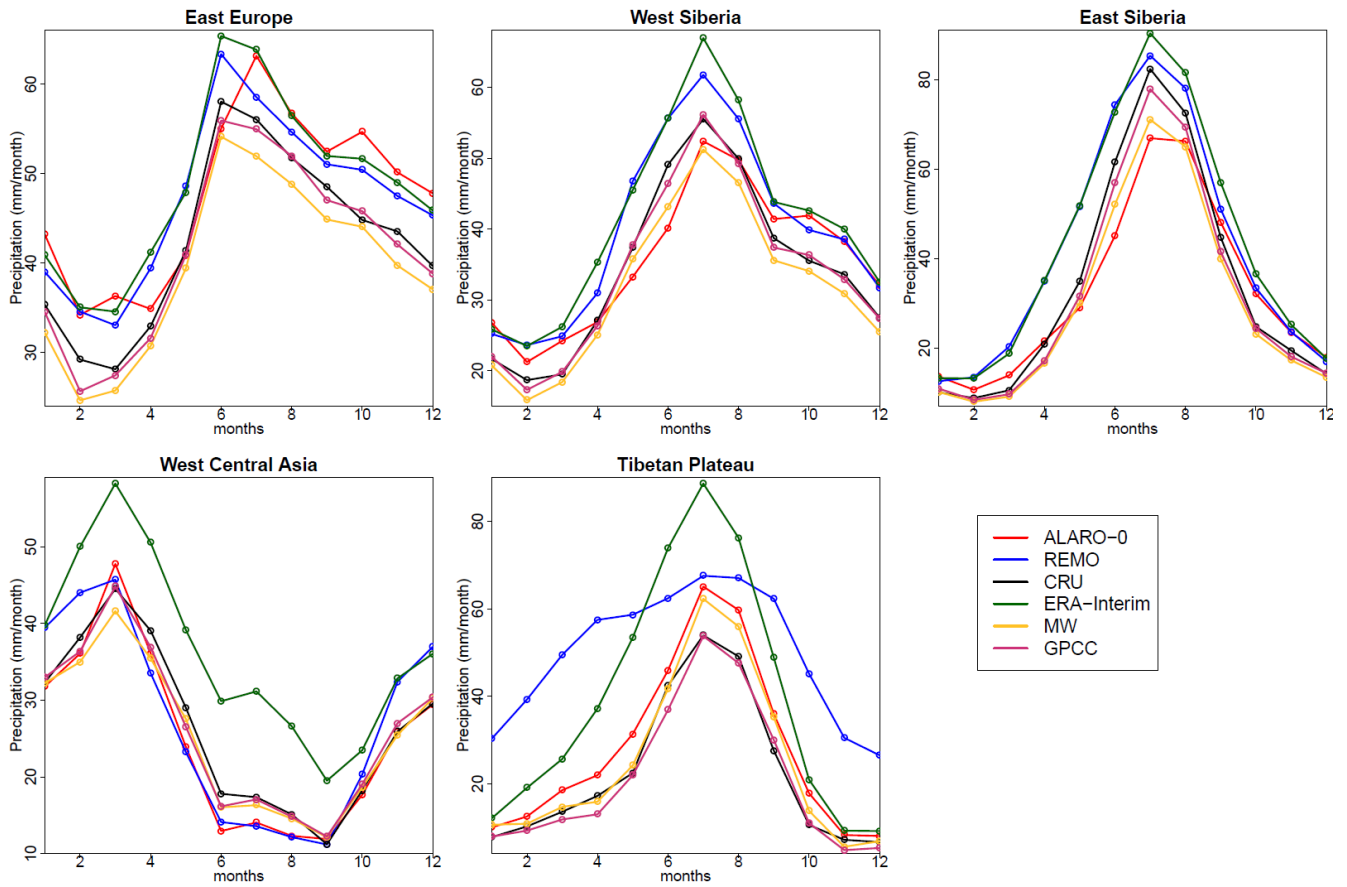
505 Figure 12: Annual cycles of precipitation (mm/month) for both RCMs (ALARO-0 and REMO) compared to the ERA-Interim reanalysis, MW, GPCC and CRU observational data over five subregions.
