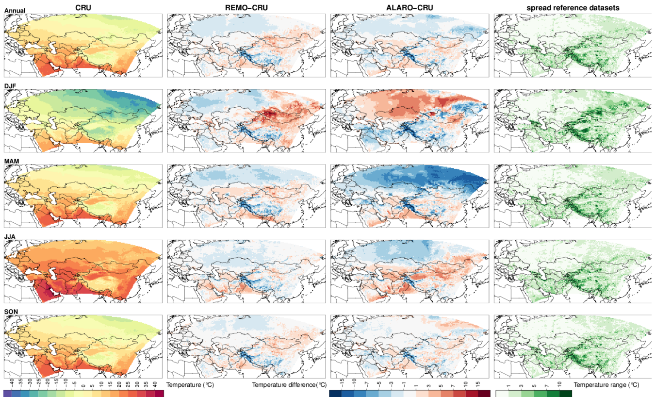
Figure 3: Left column: mean air temperature (°C) at 2 m height over the CAS-CORDEX domain based on the observational CRU dataset for the 1980-2017 period on annual level and for winter (DJF), spring (MAM), summer (JJA) and autumn (SON). In the middle columns: difference in mean temperature between models and CRU. Right column: the range in mean temperature (°C) between the different reference datasets (CRU, MW and ERA-Interim).
