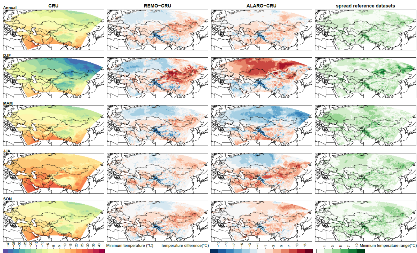
Figure 6: Left column: minimum air temperature (°C) at 2 m height over the CAS-CORDEX domain based on the observational CRU dataset for the 1980-2017 period on annual level and for winter (DJF), spring (MAM), summer (JJA) and autumn (SON). In the middle columns: difference in minimum temperature between models and CRU. Right column: the range in minimum temperature (°C) between the different reference datasets (CRU and ERA-Interim).
