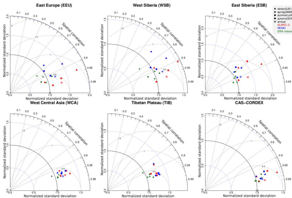
Figure 89: Normalized Taylor diagram expressing the model spatial performance of the maximum temperature for seasonal and annual means for both RCMs (ALARO-0 and REMO) and ERA-Interim reanalysis with respect to CRU for the five subdomains/subregions and the complete CAS-CORDEX domain.
