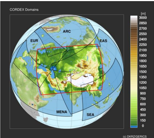
Figure 1: The CAS-CORDEX domain demarcated delineated by a red contour and the main overlapping CORDEX domains (black contour lines): Europe (EUR), Arctic (ARC), South East Asia (SEA), East Asia (EAS) and MENA projected upon the topography of Eurasia (geopotential height [m] of the GTOPO30 global digital elevation model (DEM) 3). All points with orography higher than 3000 m are colored white.
