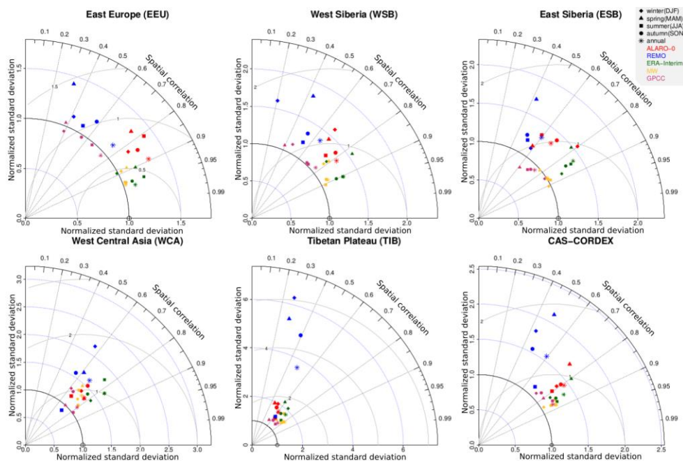
Figure 101: Normalized Taylor diagram expressing the model performance of precipitation for seasonal and annual means for both RCMs (ALARO-0 and REMO), gridded observational datasets (MW, GPCC) and the ERA-Interim reanalysis data with respect to CRU for the five subdomains and CAS-CORDEX domain.
