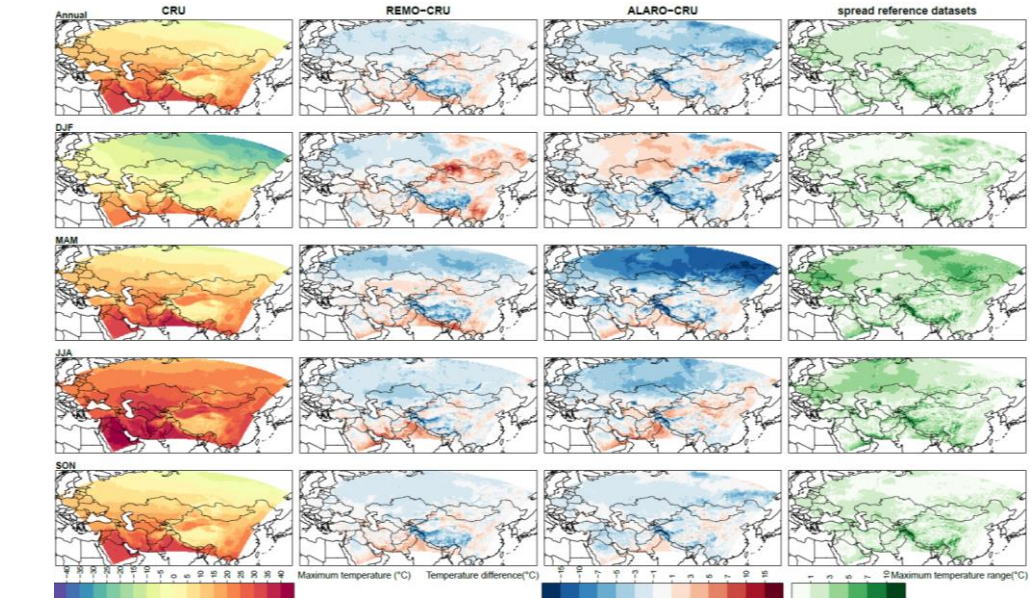
Figure 87: Left column: maximum air temperature ( ^{\circ}\text{C} ) at 2 m height over the CAS-CORDEX domain based on the observational CRU dataset for the 1980-2017 period on annual level and for winter (DJF), spring (MAM), summer (JJA) and autumn (SON). In the middle columns: difference in maximum temperature between models and CRU. Right column: the range in maximum temperature ( ^{\circ}\text{C} ) between the different reference datasets (CRU and ERA-Interim).
