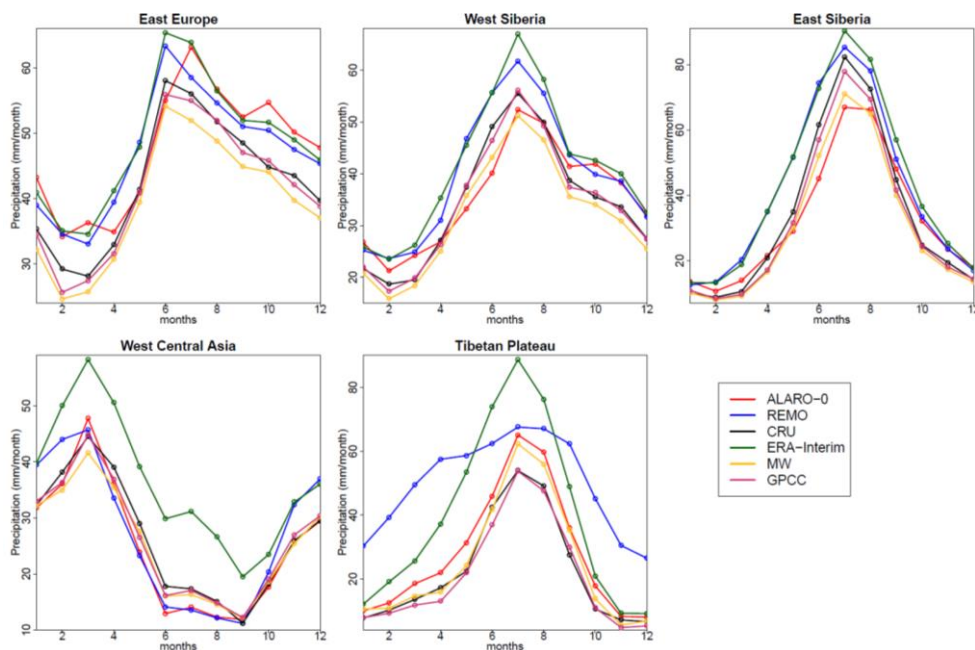
Figure 142: Annual cycles of precipitation (mm/month) for both RCMs (ALARO-0 and REMO) compared to the ERA-Interim reanalysis, MW, GPCC and CRU observational data over five subdomains/subregions.
