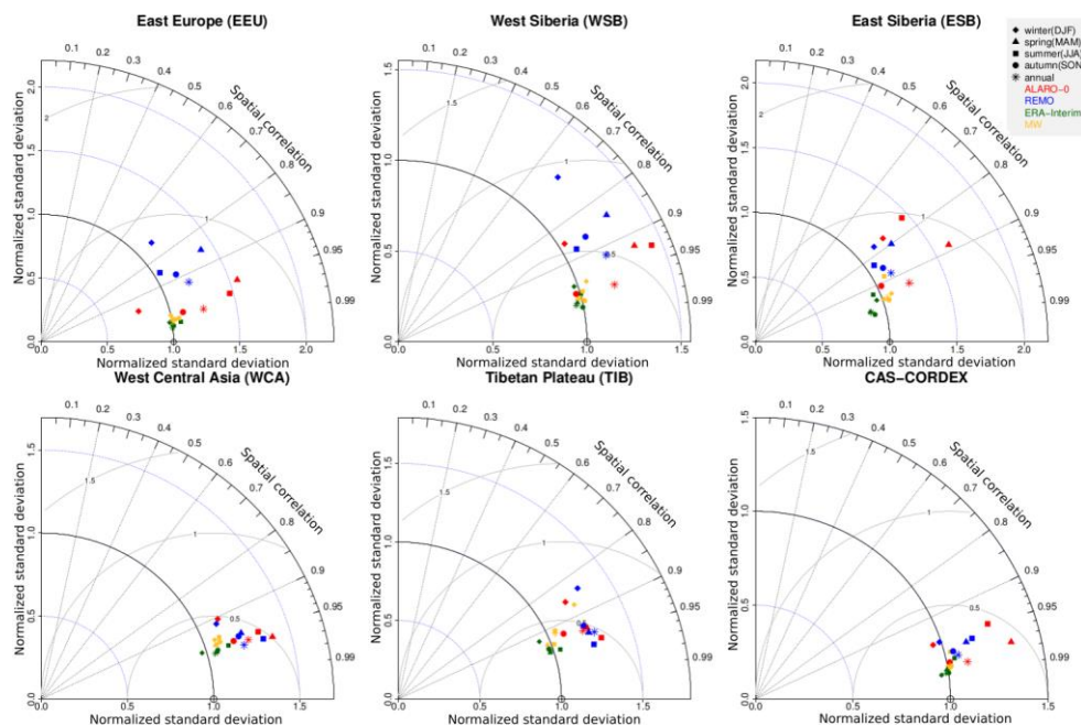
Figure 43: Normalized Taylor diagram, expressing the spatial performance of mean temperature for seasonal and annual means for both RCMs (ALARO-0 and REMO), the ERA-Interim reanalysis and MW observational data with respect to CRU for the five subregions/subdomains and the complete CAS-CORDEX domain.
