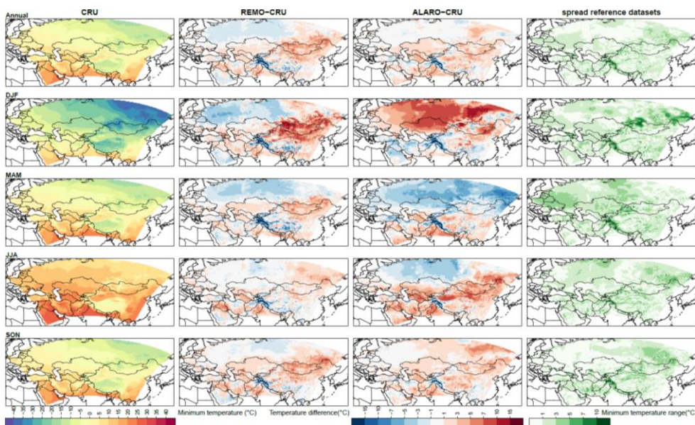
Figure 56: Left column: minimum air temperature (°C) at 2 m height over the CAS-CORDEX domain based on the observational CRU dataset for the 1980-2017 period on annual level and for winter (DJF), spring (MAM), summer (JJA) and autumn (SON). In the middle columns: difference in minimum temperature between models and CRU. Right column: the range in minimum temperature (°C) between the different reference datasets (CRU and ERA-Interim).
