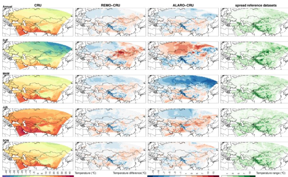
Figure 3: Left column: mean air temperature ( ^{\circ}\text{C} ) at 2 m height over the CAS-CORDEX domain based on the observational CRU dataset for the 1980-2017 period on annual level and for winter (DJF), spring (MAM), summer (JJA) and autumn (SON). In the middle columns: difference in mean temperature between models and CRU. Right column: the range in mean temperature ( ^{\circ}\text{C} ) between the different reference datasets (CRU, MW and ERA-Interim).
