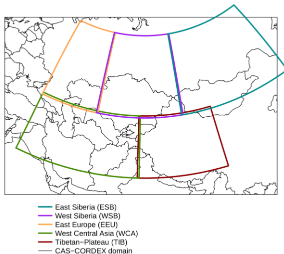
Figure 2: IPCC6 subregions projected on the CAS-CORDEX region.
