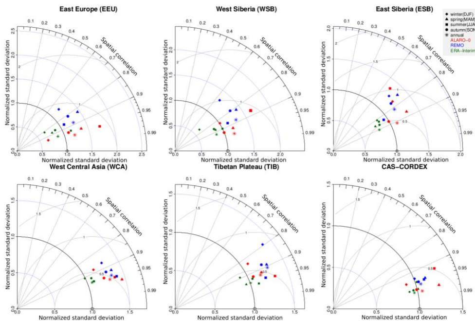
Figure 67: Normalized Taylor diagram expressing the model spatial performance of the minimum temperature for seasonal and annual means for both RCMs (ALARO-0 and REMO) and ERA-Interim reanalysis with respect to CRU for the five subdomains/subregions and the complete CAS-CORDEX domain.
