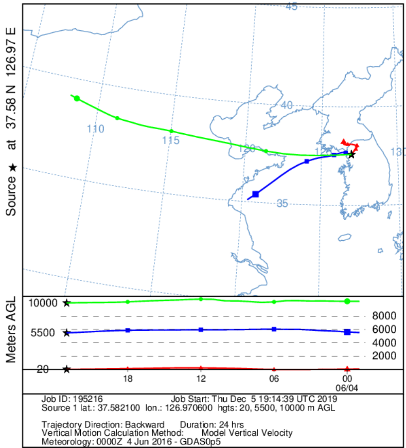
Figure S1: HYSPLIT back-trajectory output for June 4, 2016 from three different heights similar to packets.
