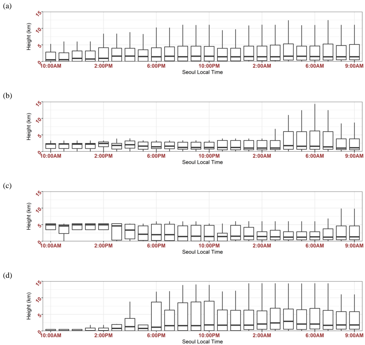
10 Figure S2. Boxplot outputs of Heights of C-TRAIL outputs for different periods of May 2016, (a) the entire month of May 2016 (b) Dynamic weather period (DWP) (c) Stagnant period (SP) (d) Extreme pollution period (EPP)
