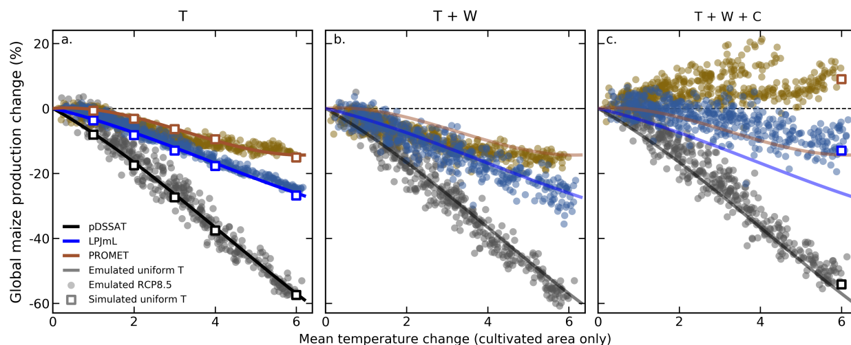
Figure 11. Illustration of the factors affecting yields in more realistic climate scenarios, for three different crop models. Figure shows emulated yield changes (relative to 1981–2010) for maize (both rainfed and irrigated) on currently cultivated land under RCP8.5 climate projections from 5 representative CMIP-5 climate models, using changes to T only (a), to T and W (b), and to T, W, and C (c). X-axis is the mean growing-season temperature change over cultivated land, computed using the historical growing season; note these values will be higher than the corresponding global mean temperature change. Circles are emulated yearly global production changes to 2100 (90 years \times 5 climate timeseries = 450 per crop model), with x-axis the mean historical growing-season T shift over all grid cells where maize is grown (unweighted by within-cell cultivated area). a: Using only temperature changes allows comparing regional simulated and emulated values. Open squares are simulated values for each T level, with CWN at baseline; bold lines are emulated values over uniform T shifts (repeated in each panel). Emulation uncertainty (compare squares to lines) is small relative to differences across climate and crop models, and mean yield changes are similar whether T changes are applied as a uniform shift or in a more realistic spatial pattern (compare lines to circles). b: Adding in precipitation changes increases yield spread across climate projections and depresses yield slightly. c: CO 2 fertilization is small in pDSSAT, moderate in LPJmL, and very large in PROMET. The separation of groups of points in PROMET (gold) results because CMIP-5 climate sensitivities differ by nearly a factor of two; points at far right are under HadGEM2-ES. In RCP8.5, the 30-year-average CO 2 at end of century is 807 ppm (Riahi et al., 2011). For comparison, open squares in c show GGCMII simulated production changes at T+6, W=0, C=810 ppm. (Note that in these climate projections, mean CO 2 levels when T > 5.8 degrees is 912 ppm.) See Supplemental Figures S14–15 for analogous figures for other crops (spring wheat and soybeans).
