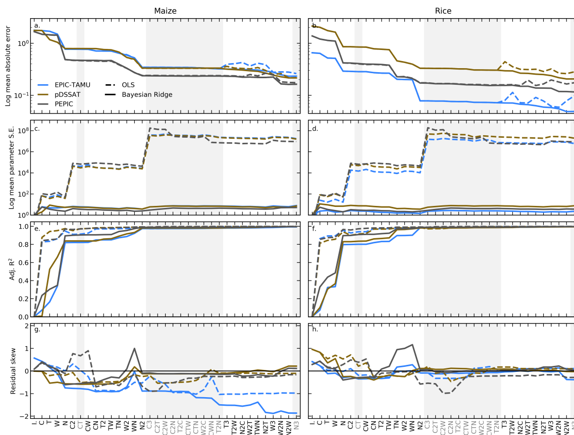
Figure 3. Illustration of results from the polynomial feature selection process for three different crop models (colors), for all grid cells with more than 1000 ha cultivated for maize ( left ) and rice ( right ). Solid lines are Bayesian Ridge regression results and dashed lines those for standard OLS. Rows show four metrics of fit quality and x axes the terms successively tested in the statistical model, sequentially added to the model in order from left to right. Terms that do not reduce the aggregate error are marked in gray and are not included in the final model. a & b: log mean absolute error between emulated yield and simulated values calculated with a three fold cross validation process, where the emulator is trained on two thirds of the data and predicts the remaining third. c & d: log mean standard parameter error. The Bayesian Ridge method strongly reduces parameter error and results in more stable estimates. e & f: adjusted R^2 score for the fit at each model specification. g & h: distribution of the residuals. Skewness is low at the high model specifications tested in all model cases other than EPIC-TAMU maize.
