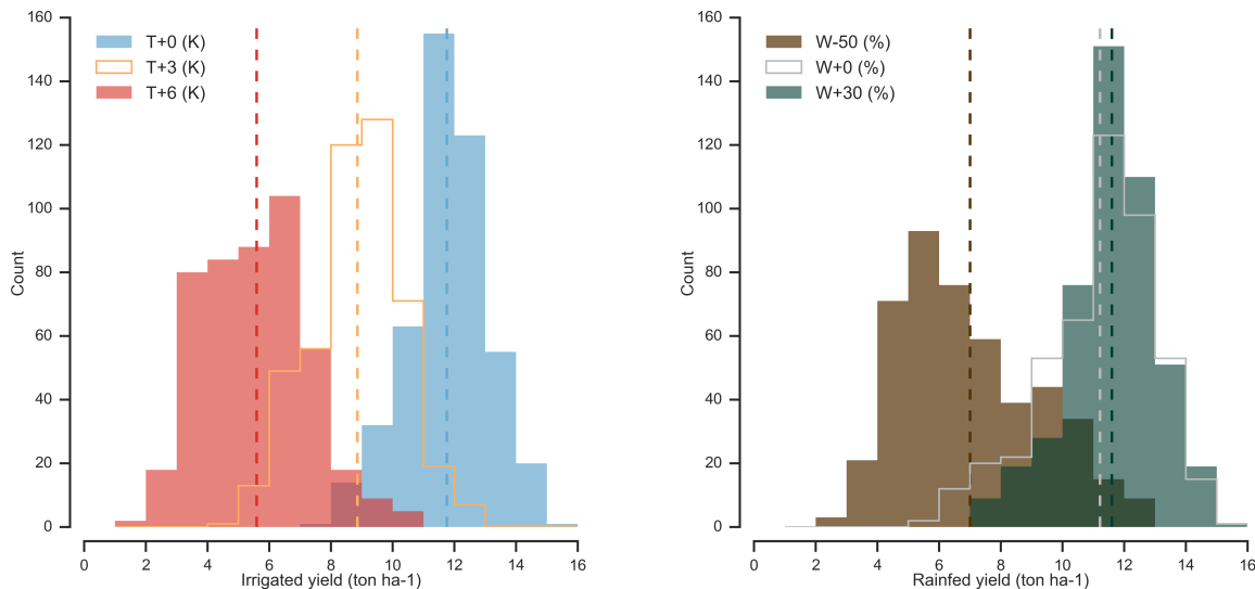
Figure 2. Example showing results of increased crop-yield sensitivity to year-to-year climate variations under climate stress. Yield distributions are from examples of Figure 1, top row, of maize in Iowa, ( left ) for irrigated maize in scenarios of altered temperature and ( right ) for rainfed maize in scenarios of altered precipitation. Because yield sensitivities rise under strong warming or drying, distributions of year-to-year crop yields widen in T+6 and P-50% scenarios relative to present-day simulations, even though all input climate timeseries have identical variance for temperature. Note: precipitation changes have different variance since the perturbations are fractional.
