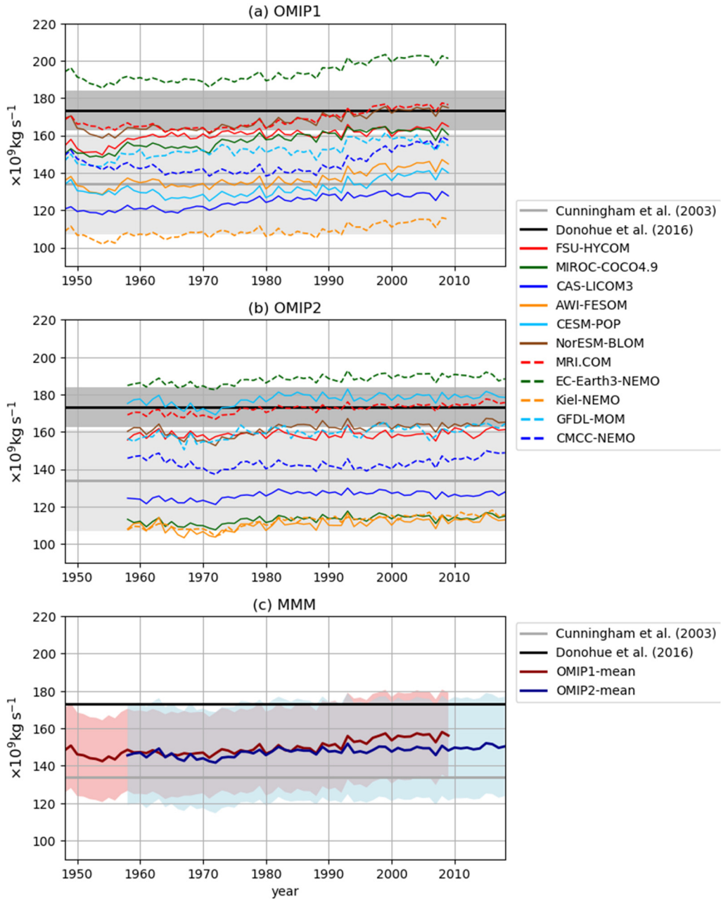
1975 Figure 20: Same as Fig. 19, but for the Drake passage transport (positive eastward), which represents the strength of Antarctic Circumpolar Current. Units are 10^9 \text{ kg s}^{-1} . Observational estimates are due to Cunningham et al. (2003) 134 \pm 27 \text{ Sv} ( 1 \text{ Sv} = 10^9 \text{ kg s}^{-1} ) and Donohue et al. (2016) 173.3 \pm 10.7 \text{ Sv} .
