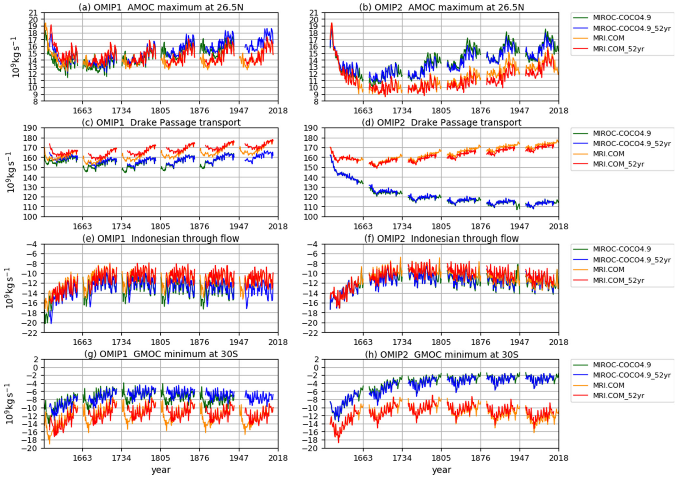
2040 Figure B2: Time series of annual mean ocean circulation metrics of the two sets of OMIP-1 and OMIP-2 simulations differing in the period used for repeating conducted by two models (MIROC-COCO4.9 and MRI.COM). (green) MIROC-COCO4.9 simulations using full period (1948–2009 for OMIP-1 and 1958–2018 for OMIP-2) for repeating. (blue) MIROC-COCO4.9 simulations using common period of OMIP-1 and OMIP-2 forcing (1958–2009) for repeating. (orange) MRI.COM simulations using full period and (red) MRI.COM simulations using 1958–2009. (a, b) Atlantic meridional overturning circulation (AMOC) maximum at 26.5°N. (c, d) Drake passage transport (positive transport eastward). (e, f) Indonesian Throughflow (negative into the Indian Ocean). (g, h) Global meridional overturning circulation (GMOC) minimum between 2000 m – bottom at 30°S. Units are 10 9 kg s -1 . 2045
