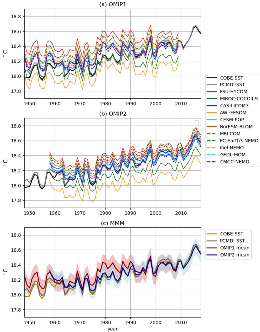
Figure 21: Same as Fig. 19, but for the globally averaged sea surface temperature ( ^{\circ}\text{C} ). Observational estimates by COBE-SST (Ishii et al. 2005) and PCMDI-SST are depicted as references. The model spreads ( \pm 2\sigma ) of both OMIP-1 and OMIP-2 capture the observation for the entire period. The z-value of the difference between OMIP-1 and OMIP-2 for the period from 1980 to 2009 is -0.46 (See also Table 2).
