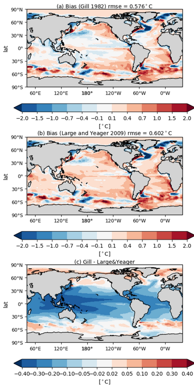
2055 Figure B4: Upper two panels show the bias of 30-year (1980–2009) mean SST relative to PCMDI-SST of two OMIP-2 simulations by MRI.COM differing in the set of formulae for properties of moist air used to compute surface turbulent fluxes. (a) Gill (1982) and (b) Large and Yeager (2004; 2009). (c) (a) minus (b). Units are degrees Celsius (°C).
