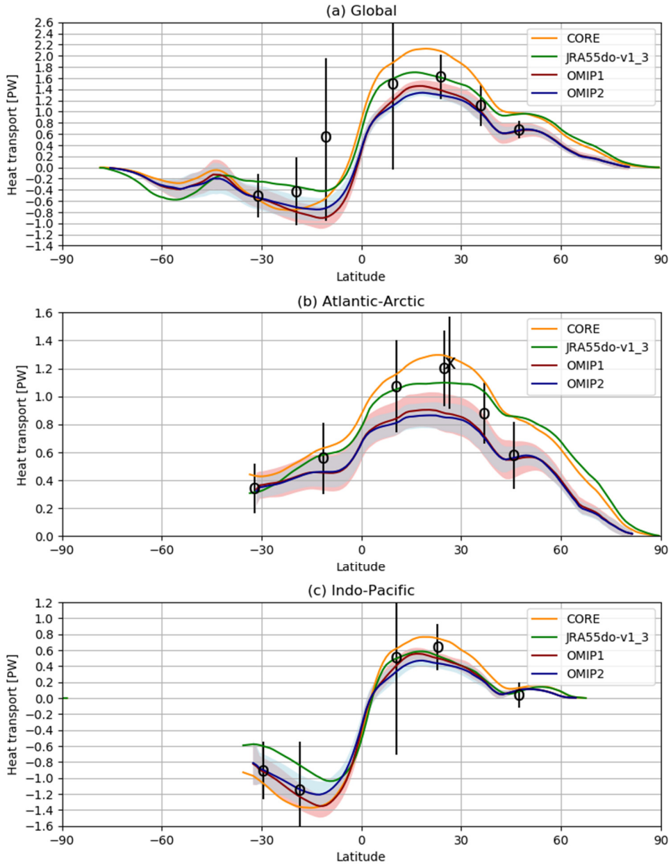
1955 Figure 17: Multi-model mean, 20-year (1988–2007) mean northward heat transport ( PW = 10^{15} \text{ W m}^{-2} ) in three oceanic basins. (a) Global, (b) Atlantic-Arctic, and (c) Indo-Pacific Ocean basins. Multi-model mean (lines) and spread defined as one standard deviation of the ensemble (shades) of OMIP-1 (red) and OMIP-2 (blue). For reference, implied northward heat transports derived from CORE (orange) and JRA55-do (green) dataset using sea surface temperature from COBE-SST (Ishii et al. 2005) as the lower boundary condition are depicted as in Tsujino et al. (2018). The open circles are estimated from observations and assimilations compiled by Macdonald and Baringer (2013). The cross at 26.5°N in the Atlantic (b) is an estimation from RAPID transport array reported by McDonagh et al. (2015). See Figs. S42 and S43 for results of individual models.
