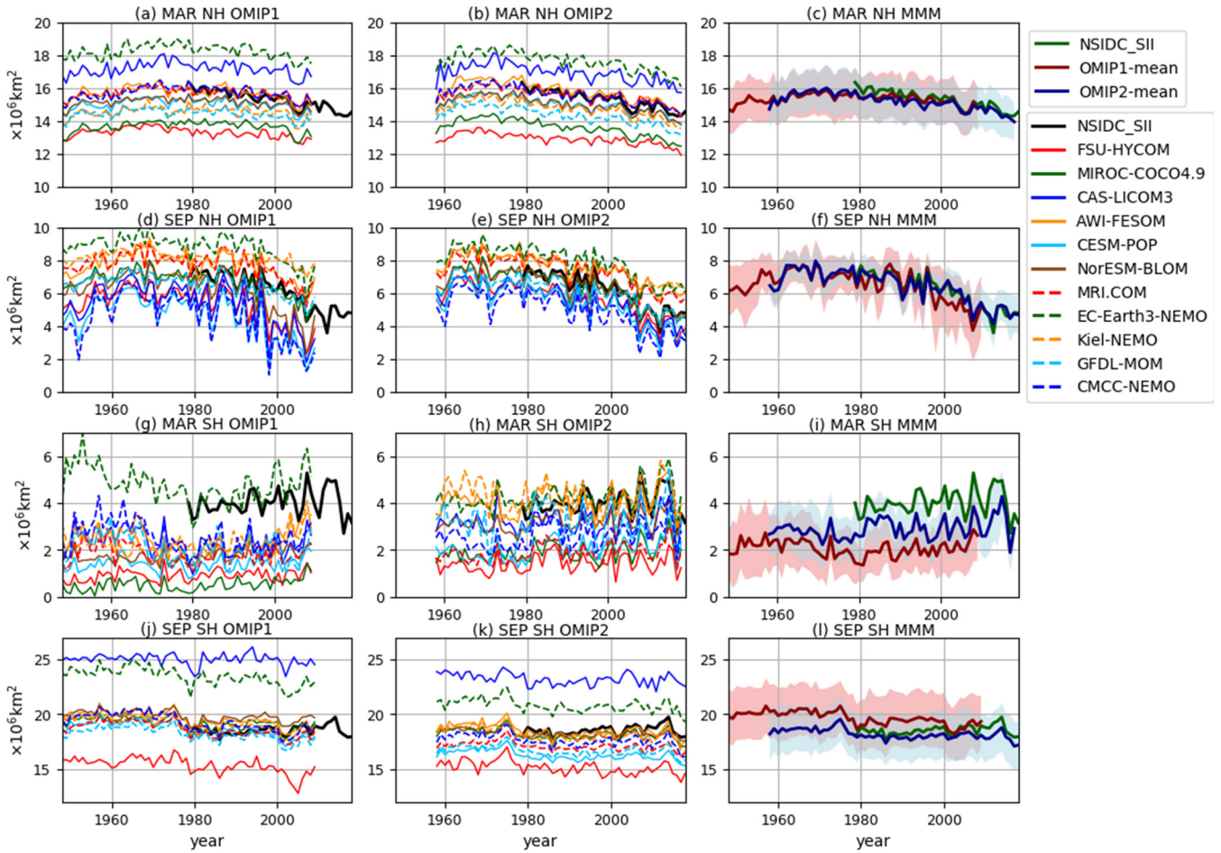
1985 Figure 22: Time series of sea ice extent in both hemispheres of the last cycle of the simulations ( 10^6 \text{ km}^2 ). (a – c) March (winter) sea ice extent in the northern hemisphere. (d – f) September (summer) sea ice extent in the northern hemisphere. (g – i) March (summer) sea ice extent in the southern hemisphere. (j – l) September (winter) sea ice extent in the southern hemisphere. (a,d,g,j) OMIP-1, (b,e,h,k) OMIP-2, (c,f,i,l) Multi model mean (lines) and spread defined as one standard deviation (shades) of OMIP-1 (red) and OMIP-2 (blue). In each panel, National snow and ice data center Sea Ice Index (NSIDC-SII; Fetterer et al. 2017) has been depicted as a reference with bold black lines for the left and middle panels and bold green lines for the right panels. The model spreads ( \pm 2\sigma ) of both OMIP-1 and OMIP-2 capture the observation except for summer in the southern hemisphere of the OMIP-1 simulations (55% of the period from 1979 to 2009). See Table 2 for the z-values of the difference between OMIP-1 and OMIP-2 for the period from 1980 to 2009. 1990
