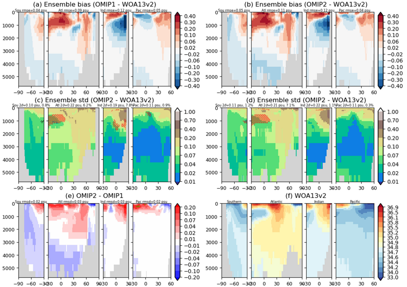
1930 1935 Figure 14: Upper two panels show biases of multi-model mean, 30-year (1980–2009) mean basin-wide zonally averaged salinity of the last cycle relative to WOA13v2 (Zweng et al. 2013) for (a) OMIP-1 and (b) OMIP-2. Middle two panels show the standard deviation of the ensemble, with the regions where the observation is outside the 95% confidence range of the model spread ( \pm 2\sigma ) hatched with red. (c) OMIP-1 and (d) OMIP-2. (e) Difference of 30-year (1980–2009) mean basin-wide zonal mean salinity between OMIP-2 and OMIP-1 (OMIP-2 minus OMIP-1), with the regions where the difference is significant at 95% confidence level hatched with green as in Fig. 6. (f) Basin-wide zonal mean salinity of WOA13v2. Units are psu. On the top of each panel, basin mean values are depicted as in Fig. 13. See Figs. S36 through S38 for results of individual models.
