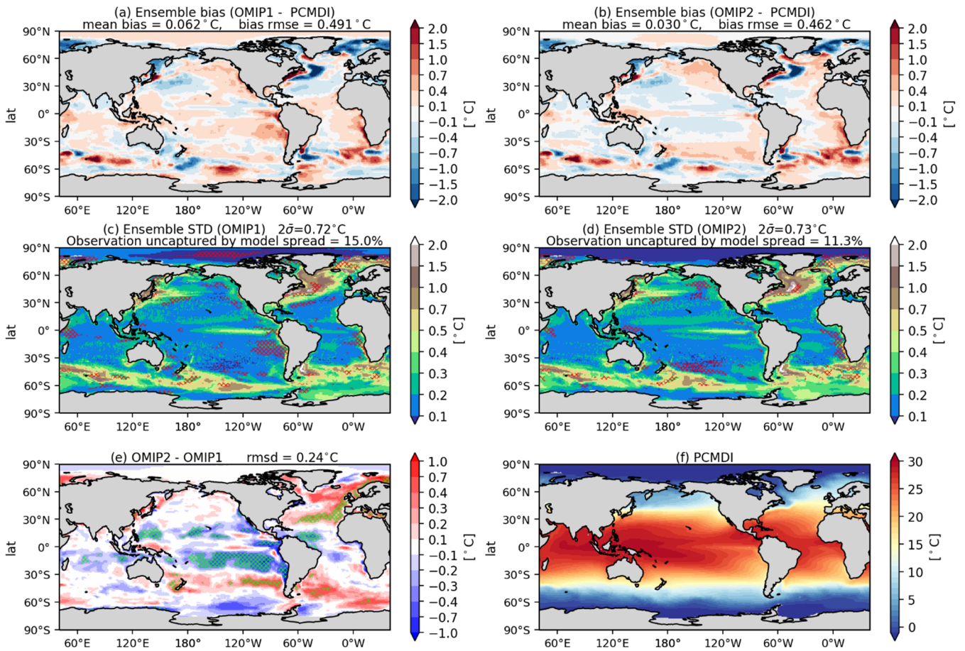
1855 Figure 6: Evaluation of the simulated mean sea surface temperature (SST; units in °C). Upper two panels show the bias of the multi-model mean, 30-year (1980–2009) mean SST relative to an observational estimate provided and updated by Program for Climate Model Diagnosis and Intercomparison (PCMDI) following a procedure described by Hurrell et al. (2008) (hereafter referred to as PCMDI-SST). (a) OMIP-1 and (b) OMIP-2, with global mean bias and global root-mean-square bias depicted on the top. The middle two panels show the standard deviation of the ensemble, with the regions where the observation is outside the 95% confidence range of the model spread ( \pm 2\sigma ) hatched with red. (c) OMIP-1 and (d) OMIP-2, with the global mean confidence range (twice the standard deviation) and the fraction of the region where observation is uncaptured by the model confidence range depicted on the top. (e) Difference between OMIP-1 and OMIP-2 (OMIP-2 minus OMIP-1), with the global root-mean-square difference depicted on the top. The regions where the difference is significant at 95% confidence level are hatched with green, with the uncertainty of multi-model mean difference computed based on the method proposed by Wakamatsu et al. (2017). (f) 30-year (1980–2009) mean SST of PCMDI-SST. In the following figures, all models are used for multi-model mean. See Figs. S10 through 1860 1865
