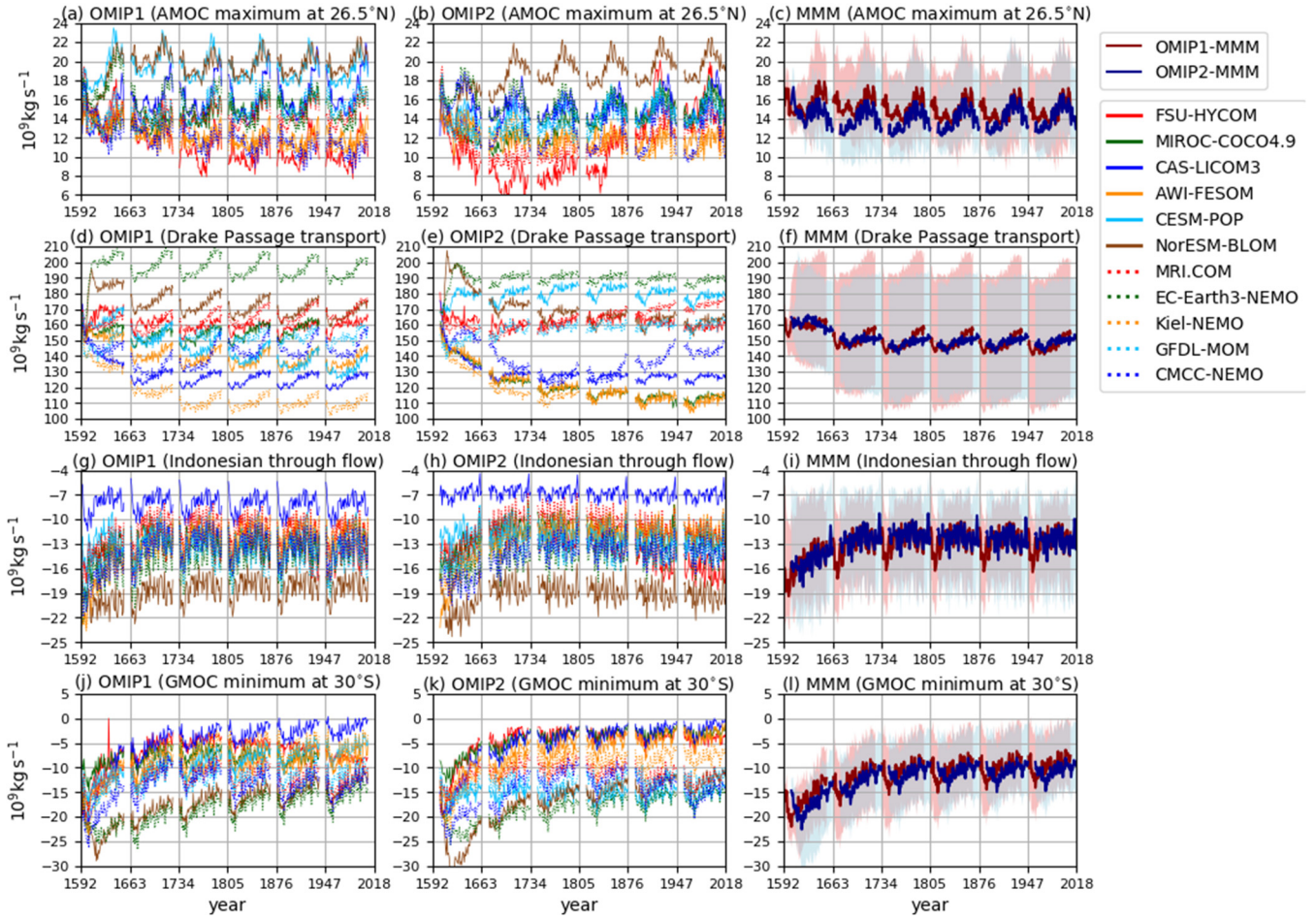
Figure 5: Time series of annual mean ocean circulation metrics. (a-c) Atlantic meridional overturning circulation (AMOC) maximum at 26.5°N, which approximately represents the strength of AMOC associated with the North Atlantic Deep Water formation. (d-f) Drake passage transport (positive eastward), which represents the strength of Antarctic Circumpolar Current. (g-i) Indonesian Throughflow (negative into the Indian Ocean), which represents water exchange between the Pacific and Indian Ocean. (j-l) Global meridional overturning circulation (GMOC) minimum in 2000 m – bottom depths at 30°S, which represents the strength of deep to bottom layer GMOC associated with the Antarctic Bottom Water and Lower Circumpolar Deep Water formation. (a,d,g,j) OMIP-1 and (b,e,h,k) OMIP-2. (c,f,i,l) Multi-model mean (lines) and spread defined as the range between maximum and minimum (shades) of OMIP-1 (red) and OMIP-2 (blue). Units are 10^9 \text{ kg s}^{-1} . See Figs. S8 and S9 for a closer look at individual models.
