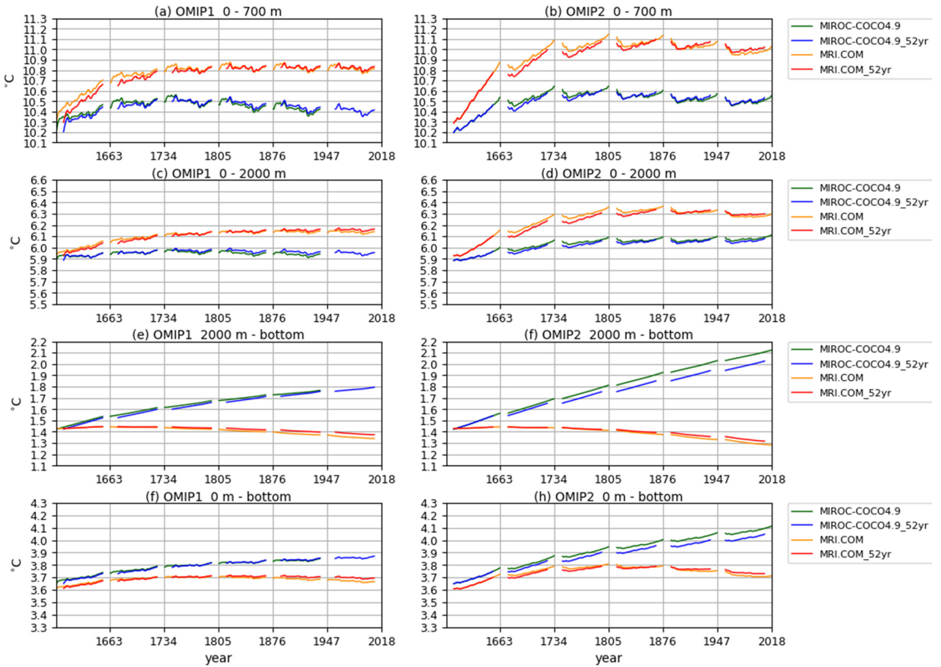
2030 Figure B1: Drift of annual mean, global mean vertically averaged temperatures (°C) for four depth ranges (a, b) 0 – 700m, (c, d) 0 – 2000m, (e, f) 2000m – bottom, (g, h) 0 m – bottom of two sets of OMIP-1 and OMIP-2 simulations differing in the period used for repeating conducted by two models (MIROC-COCO4.9 and MRI.COM). (green) MIROC-COCO4.9 simulations using full period (1948–2009 for OMIP-1 and 1958–2018 for OMIP-2) for repeating. (blue) MIROC-COCO4.9 simulations using common period of OMIP-1 and OMIP-2 forcing (1958–2009). (orange) MRI.COM simulations using full period and (red) MRI.COM simulations using 1958–2009. 2035
