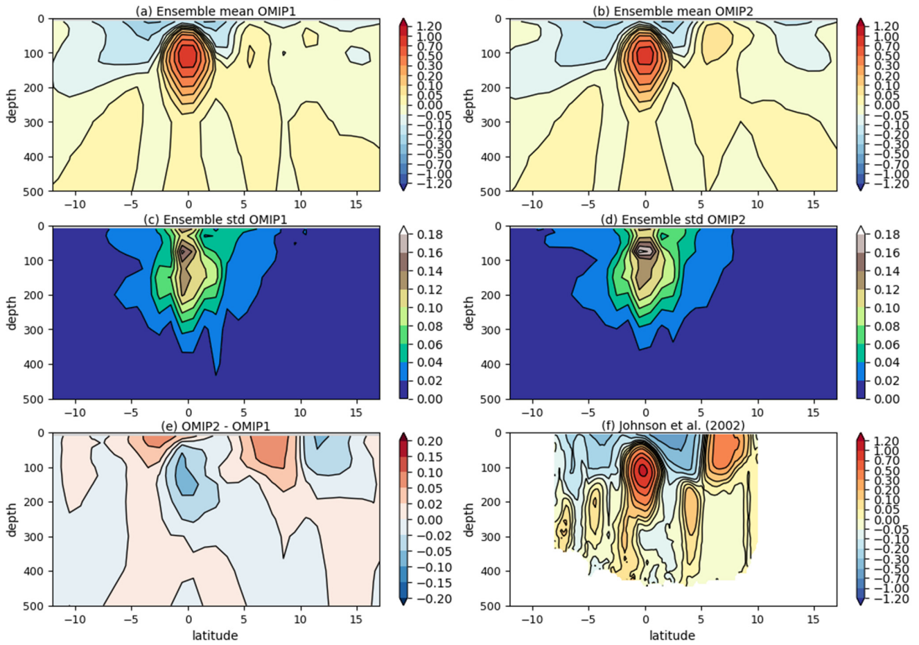
1960 Figure 18: Upper two panels show multi-model mean, 30-year (1980–2009) mean zonal velocity across 140°W in the eastern tropical Pacific. (a) OMIP-1 and (b) OMIP-2. Middle two panels show the standard deviation of the ensemble. (c) OMIP-1 and (d) OMIP-2. (e) OMIP-2 minus OMIP-1. (f) Observational estimates based on Johnson et al. (2002). Units are \text{m s}^{-1} . See Figs. S44 through S46 for results of individual models.
