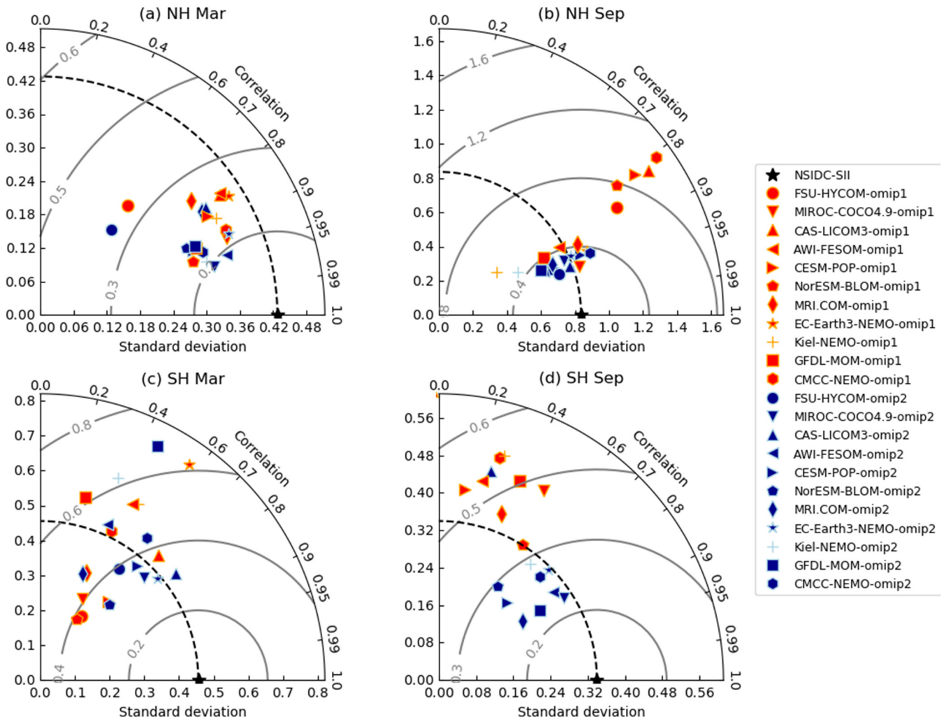
1995 Figure 23: Taylor diagram of the interannual variation of sea ice extent in both hemispheres relative to NSIDC_SII. (a) March (winter) and (b) September (summer) sea ice extent in the northern hemisphere. (c) March (summer) and (d) September (winter) sea ice extent in the southern hemisphere. Standard deviations are expressed in units of 10^6 \text{ km}^2 .
