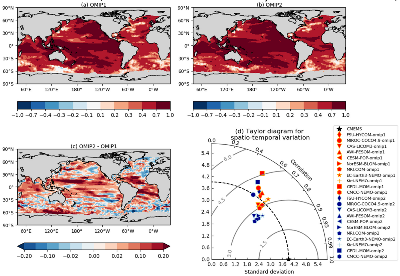
2080 Figure E4: Multi-model mean correlation coefficients of monthly SSH anomaly relative to the monthly climatology for the period 1993–2009 between simulation and CMEMS. (a) OMIP-1, (b) OMIP-2, (c) OMIP-2 – OMIP-1. (d) Taylor diagram of the total space-time pattern variability of monthly SSH anomaly relative to the monthly climatology for OMIP-1 and OMIP-2 simulations relative to CMEMS, with standard deviations expressed in units of centimeters. See Figs. S58 through S60 for results of individual models.
