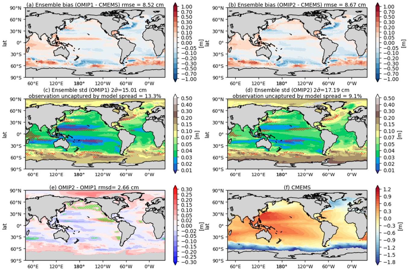
1890 Figure 10: Evaluation of simulated sea surface height (m). Upper two panels show the bias of the multi-model mean, 17-year (1993–2009) mean SSH relative to CMEMS. (a) OMIP-1 and (b) OMIP-2. The middle two panels show the standard deviation of the ensemble, with the regions where the observation is outside the 95% confidence range of the model spread ( \pm 2\sigma ) hatched with red. (c) OMIP-1 and (d) OMIP-2. (e) Difference between OMIP-1 and OMIP-2 (OMIP-2 minus OMIP-1), with the regions where the difference is significant at 95% confidence level hatched with green as in Fig. 6. (f) Annual mean SSH of CMEMS. Note that all SSH fields are offset by subtracting their respective quasi-global mean values before evaluation as described in Appendix C. On 1895 the top of each panel, global mean values are depicted as in Fig. 6. See Figs. S24 through S26 for results of individual models.
