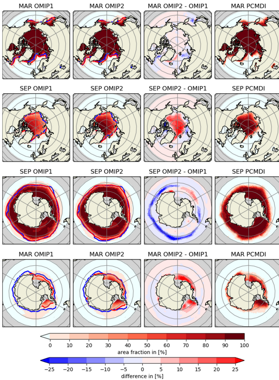
1885 Figure 9: Multi-model mean 30-year (1980–2009) mean sea ice concentration (%). Columns are (from the left) OMIP-1, OMIP-2, OMIP-2 – OMIP-1, and an observational dataset provided by PCMDI-SST. Rows are (from the top) March and September in the Northern hemisphere, and September and March in the Southern hemisphere. Blue lines are contours of 15% concentration of the PCMDI-SST dataset and red lines are those of multi-model mean. See Figs. S16 through S23 for results of individual models.
