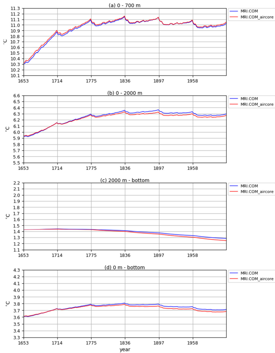
2050 Figure B3: Drift of annual mean, global mean vertically averaged temperatures (°C) for four depth ranges (a) 0 – 700m, (b) 0 – 2000m, (c) 2000m – bottom, (d) 0 m – bottom of two OMIP-2 simulations by MRI.COM differing in the set of formulae for properties of moist air used to compute surface turbulent fluxes. (blue) Gill (1982) and (red) Large and Yeager (2004; 2009).
