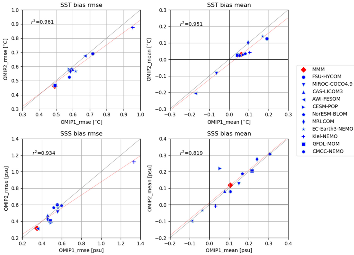
2020 Figure 27: Scatter diagram with linear fitting (red line) and its score ( r^2 ) comparing the 30-year mean (1980–2009) SST bias rmse (upper left), SST bias mean (upper right), SSS bias rmse (lower left), and SSS bias mean (lower right) from OMIP-1 (abscissa) and OMIP-2 (ordinate). See Table D3 for specific values.
