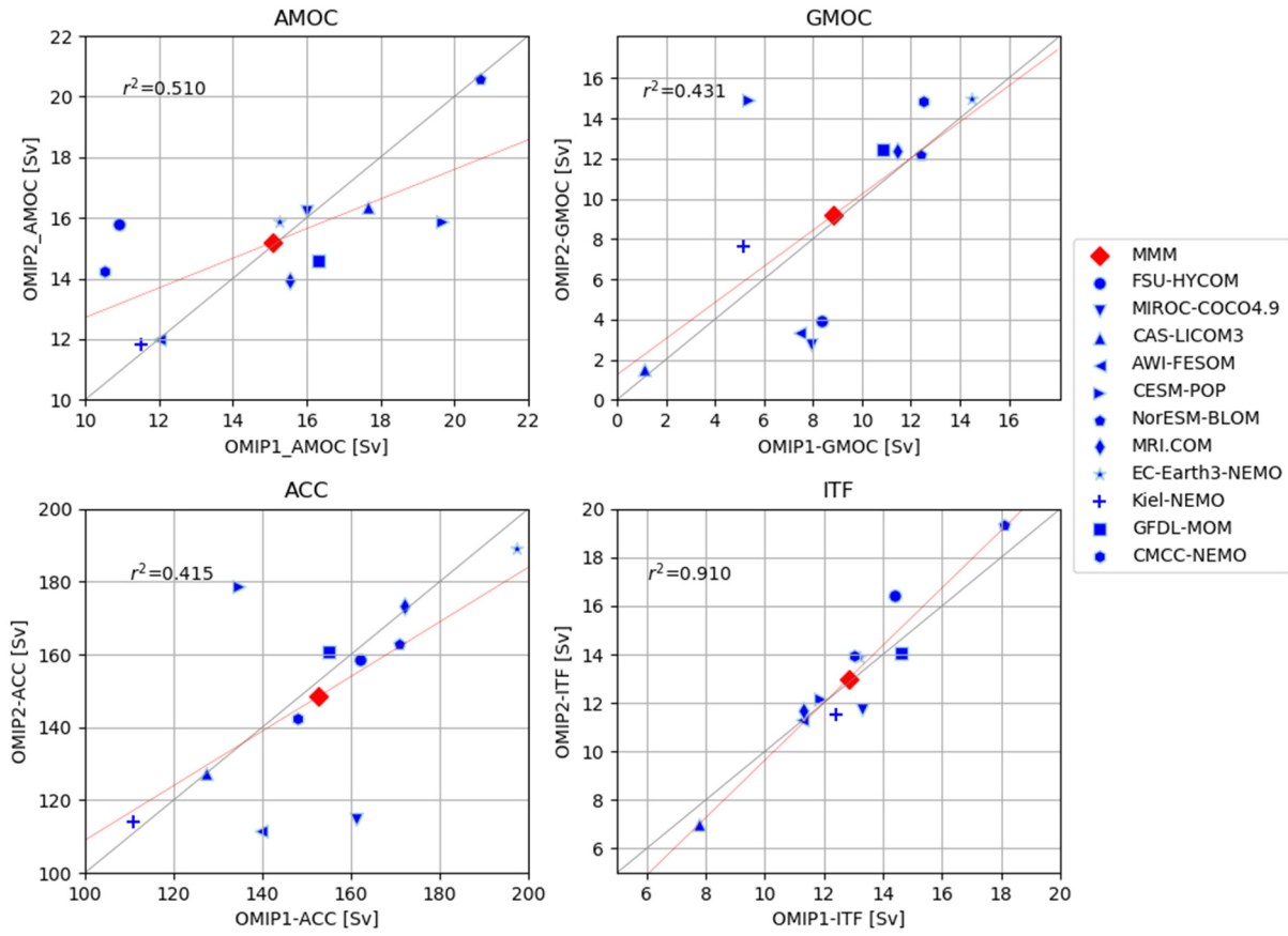
2025 Figure 28: Same as Fig. 27 but for the 30-year mean (1980–2009) AMOC (upper left), Global meridional overturning circulation (GMOC) minimum in 2000 m – bottom depths at 30°S (upper right), Antarctic Circumpolar Current (ACC) (lower left), and Indonesian Throughflow (ITF) (lower right) from OMIP-1 (abscissa) and OMIP-2 (ordinate). See Table D2 for specific values.
