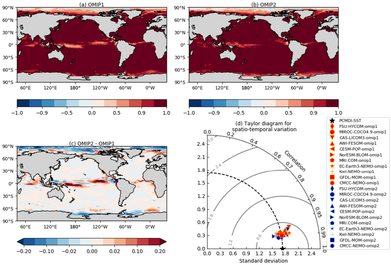
2060 Figure E1: Multi-model mean correlation coefficients of monthly climatology of SST for the period 1980–2009 between simulation and PCMDI-SST. (a) OMIP-1, (b) OMIP-2, (c) OMIP-2 – OMIP-1. (d) Taylor diagram of the total space-time pattern variability of the monthly climatology of SST of OMIP-1 and OMIP-2 simulations relative to PCMDI-SST, with standard deviations expressed in units of °C. For Figs. E1 to E5, all models are used for multi-model mean. See Figs. S49 through S51 for the results of individual models.
