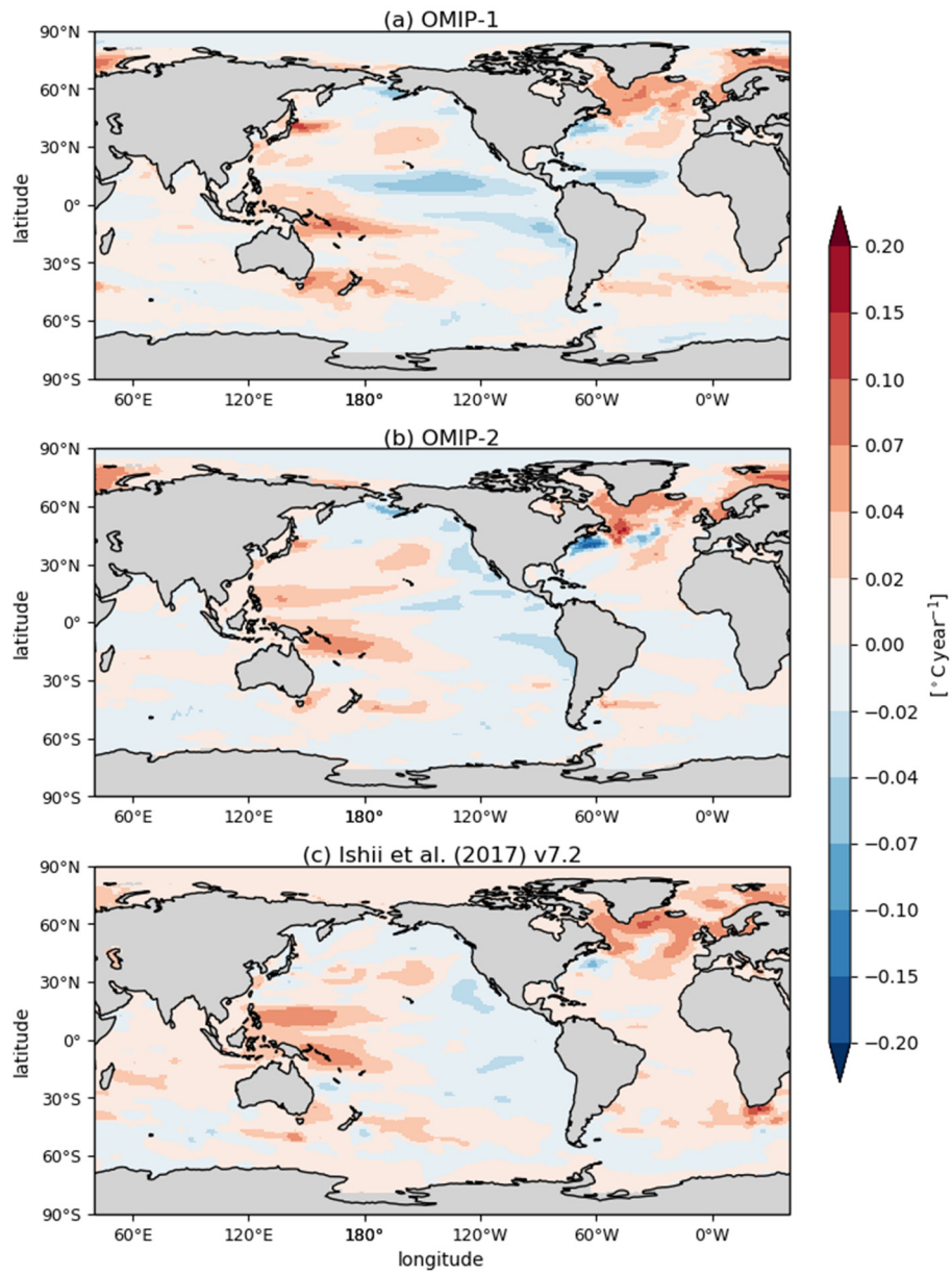
Figure 26: Multi-model mean 17-year (1993–2009) trend of upper 700 m temperature (°C year -1 ). (a) OMIP-1, (b) OMIP-2, (c) Ishii et al. (2017) v7.2. See Figs. S47 and S48 for the behavior of individual models.
