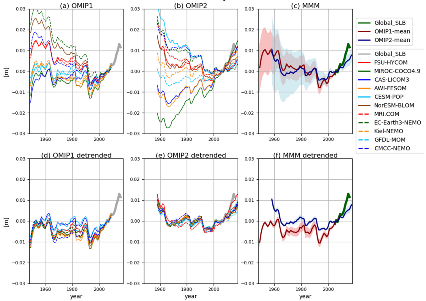
2010 Figure 25: Time series of annual mean thermosteric sea level anomaly relative to 2005 – 2009 mean (m). (a) OMIP-1, (b) OMIP-2, and (c) Multi-model mean (lines) and spread defined as one standard deviation (shades) of OMIP-1 (red) and OMIP-2 (blue). (d-f) Same as (a-c) except that linear trend is subtracted from each model. Grey lines in (a,b,d,e) and green lines in (c,f) are adopted from WCRP Global Sea Level Budget Group (2018).
