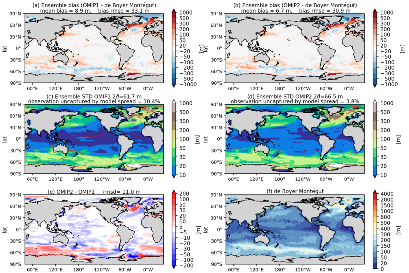
1900 Figure 11: Evaluation of simulated mixed layer depth (m). Upper two panels show the bias of the multi-model mean, 30-year (1980–2009) mean winter mixed layer depth in both hemispheres relative to observationally derived mixed layer depth data from de Boyer Montégut et al. (2004). January–February–March mean for the northern hemisphere and July–August–September mean for the southern hemisphere. (a) OMIP-1 and (b) OMIP-2. The middle two panels show the standard deviation of the ensemble, with the regions where the observation is outside the 95% confidence range of the model spread ( \pm 2\sigma ) hatched with red. (c) OMIP-1 and (d) OMIP-2. (e) Difference between OMIP-1 and OMIP-2 (OMIP-2 minus OMIP-1), which is not statistically significant at 95% confidence level everywhere. (f) Observationally derived mixed layer depth data from de Boyer Montégut et al. (2004). On the top of each panel, global mean values are depicted as in Fig. 6. Note that the regions where mixed layer depths could reach more than 1000 meters in winter, specifically the marginal seas around Antarctica (south of 60^{\circ}\text{S} ) and the high latitude North Atlantic ( 50^{\circ}\text{--}80^{\circ}\text{N} ; 80^{\circ}\text{W}\text{--}30^{\circ}\text{E} ) are excluded from the computation of global means. See Figs. S27 through S29 for results of individual models.
