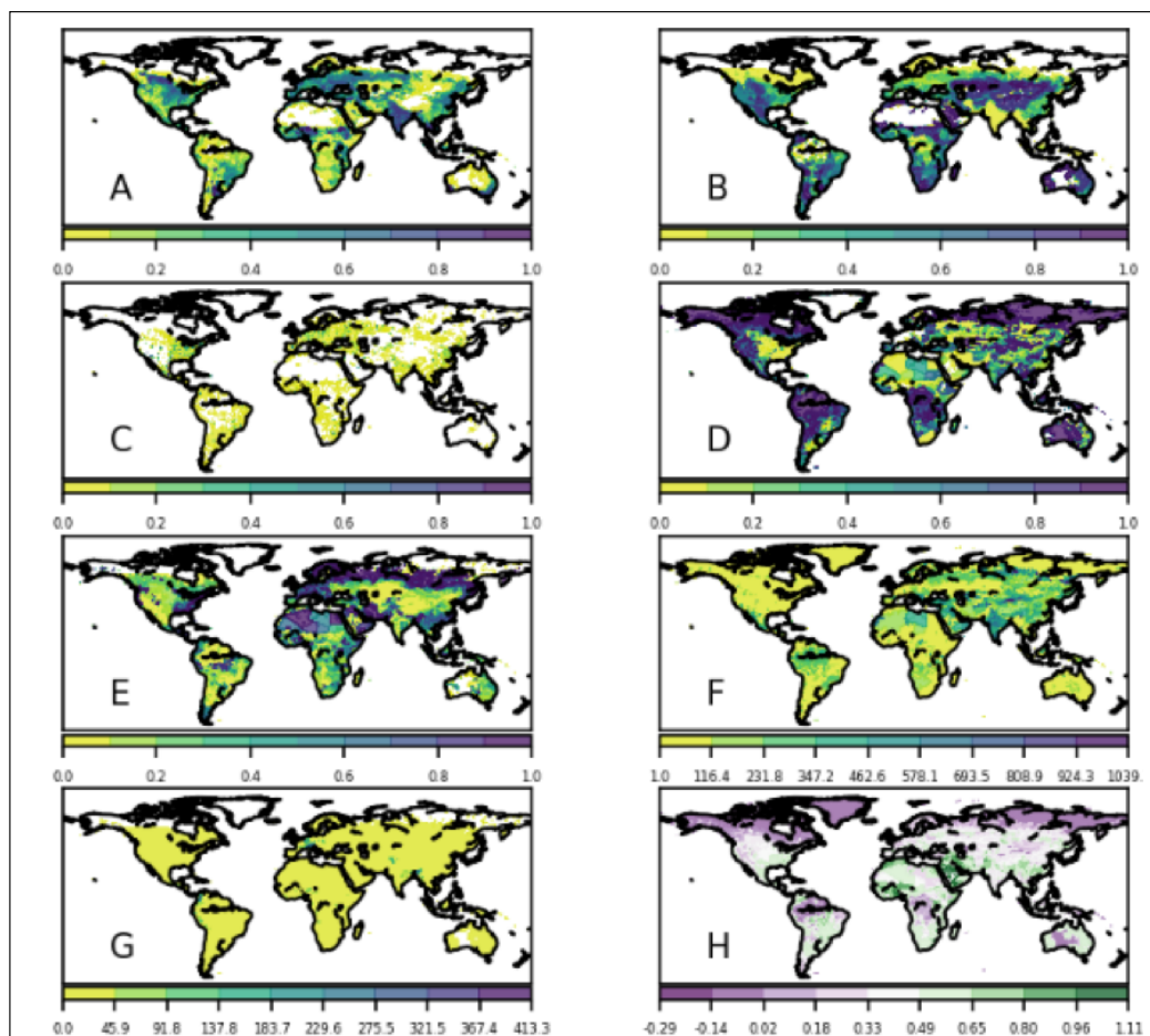
Figure 10. Maps for year 2015 showing a. fraction of each grid cell occupied by cropland b. fraction of each grid cell occupied by pasture, c. fraction of each grid cell occupied by urban land, d. fraction of each grid cell occupied by primary vegetation, e. fraction of each grid cell occupied by secondary vegetation, f. mean age (in years) of secondary lands in each half degree grid cell, g. mean gross transitions ( \text{km}^2 \text{ year}^{-1} ) over 20 year interval for each grid cell, h. mean net transitions ( \text{km}^2 \text{ year}^{-1} ) over 20 year interval for each grid cell.
