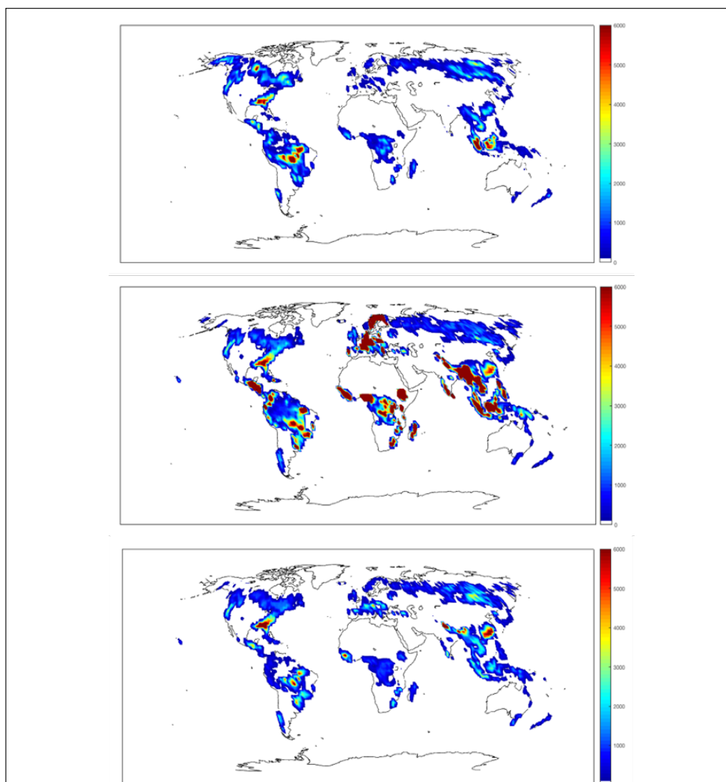
Figure 6. Forest loss 2000-2012 (a) Landsat forest loss (Hansen et al. 2013), (b) LUH2 forest loss without Landsat constraint, (c) LUH2 forest loss with Landsat constraint.
