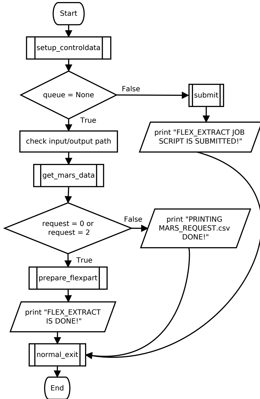
Figure 3. Flow diagram for the local application mode. If queue \neq \text{None} , flex_extract was started in remote or gateway mode and Fig. 2 applies. This is marked by the submit block. In the case of request == 1 , flex_extract skips the retrieval and post-processing steps and just writes the mars_request.csv file. Within the local mode, the retrieval ( get_mars_data ) and post-processing ( prepare_flexpart ) parts are executed. Symbols as in Fig. 2.
