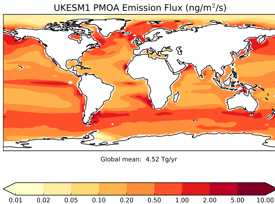
Figure 15. Annual mean emission flux of primary marine organic aerosol from UKESM1-AMIP in \text{ng}/\text{m}^2/\text{s} .
