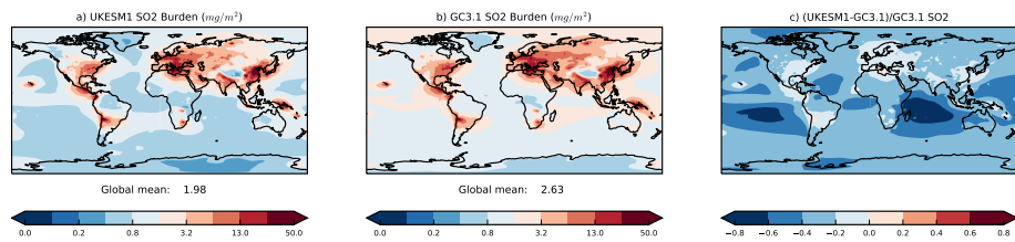
Figure 2. Annual mean SO 2 burden (mg [SO 2 ] m -2 ) in (a) UKESM1, (b) GC3.1 and (c) their relative difference. The annual mean burdens are computed from the 9 and 4 member historical ensemble means from UKESM1 and GC3.1 respectively from years 1980 to 2014 inclusive.
