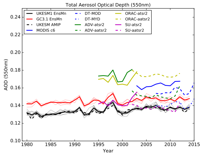
Figure 8. Timeseries of simulated annual mean aerosol optical depth (AOD) at 550nm from the UKESM1 and GC3.1 historical ensemble means with multiple satellite AOD products. Also plotted are the individual ensemble members from each model (light shading) and the UKESM1-AMIP simulation (dashed black line). The satellite products are the collection 6 MODIS merged dataset (MODIS c6), MODIS Dark Target from Terra (DT-MYD) and Aqua (DT-MOD) satellite sensors, the ATSR Dual-View dataset (ADV), the Optimal Retrieval of Aerosol and Cloud dataset (ORAC) and the Swansea University dataset (SU).
