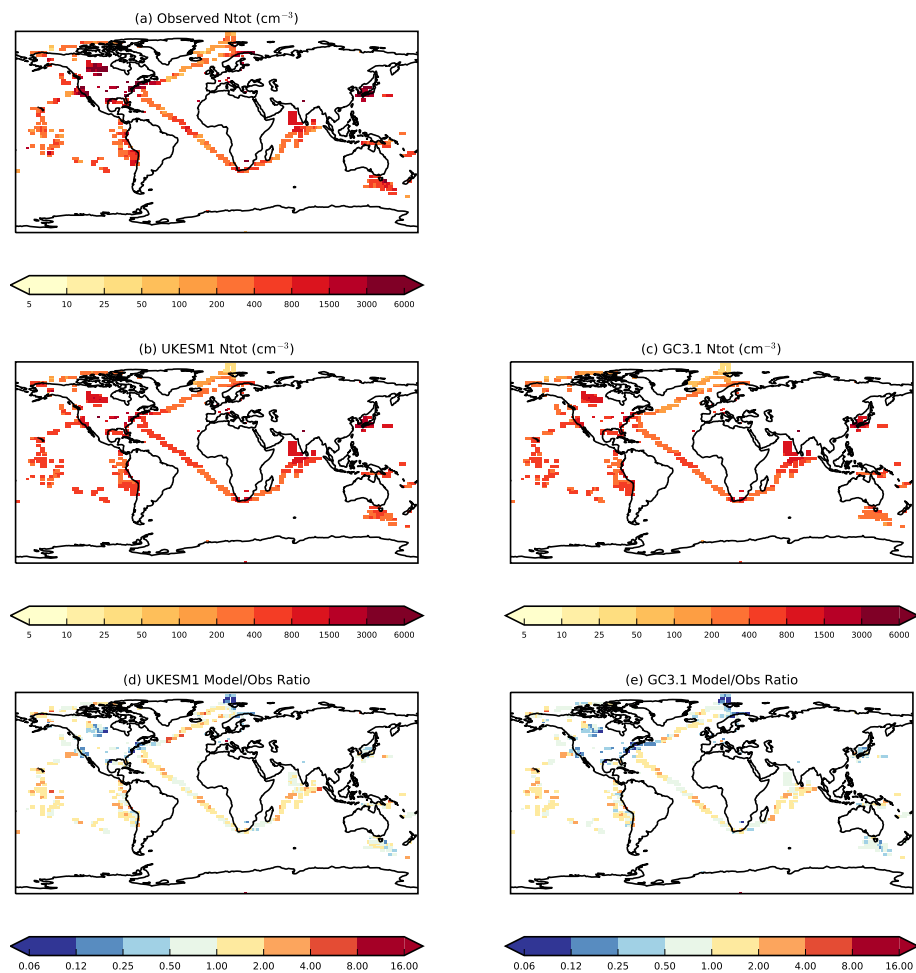
Figure 12. Comparison of simulated N_{tot} (total particle concentration with diameter > 3 nm) ( \text{cm}^{-3} ) from (a) a set of gridded observations from a combination of ground-based, ship and aircraft campaigns against (b) UKESM1 and (c) GC3.1. The ratio of model to observed data for (d) UKESM1 and (e) GC3.1.
