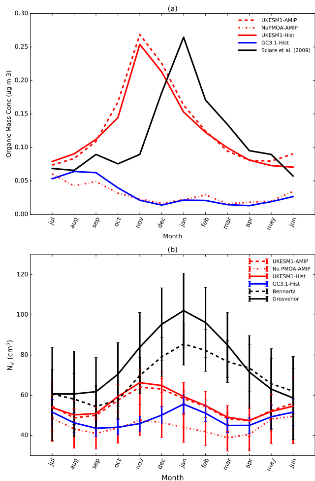
Figure 16. Seasonal evaluation of simulated (a) OM surface mass concentration at Amsterdam Island and (b) N_d averaged averaged over 30^\circ\text{S} - 70^\circ\text{S} from UKESM1-AMIP, a UKESM1-AMIP simulation with no PMOA source and the UKESM1 and GC3.1 historical ensemble means. The OM mass observations in (a) are taken from Sciare et al. (2009). The N_d observations used in (b) are taken from the Grosvenor et al. (2018b) and Bennartz and Rausch (2017) satellite N_d products. The simulated monthly N_d data is taken from the years 2003 to 2014 inclusive to match the satellite temporal coverage. Given the low data coverage of satellite retrievals in the austral winter the model and Bennartz data has been spatially sampled according to the Grosvenor data product
