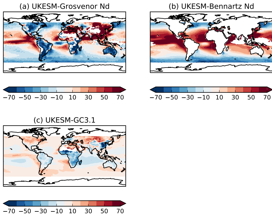
Figure 14. Annual mean bias in UKESM1 N_d from years 2003–2015 compared with (a) Grosvenor et al. (2018b), (b) Bennartz and Rausch (2017) satellite N_d products. (c) UKESM1-GC3.1 N_d .
