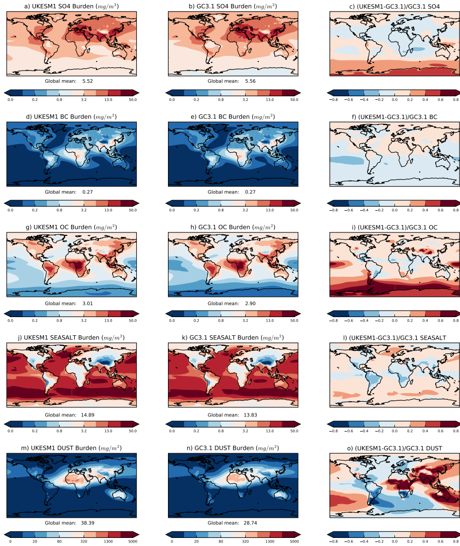
Figure 3. Annual mean burden ( mg\ m^{-2} ) of SO 4 , BC, OC, sea-salt and mineral dust aerosol in (left column) UKESM1, (middle column) GC3.1 and (right column) their fractional difference. The annual mean burdens are computed from the 9 and 4 member historical ensemble means from UKESM1 and GC3.1 respectively from years 1980 to 2014 inclusive. Note the different contour levels in panels m and n.
