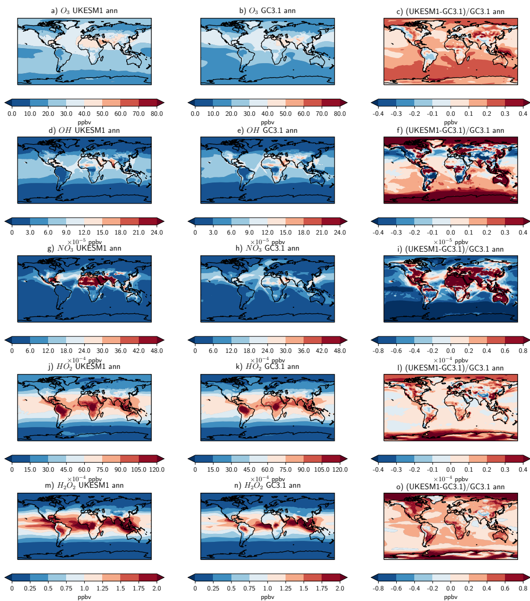
Figure 1. Annual mean surface concentrations (ppbv) of O_3 , OH , NO_3 , HO_2 and H_2O_2 from (left column) UKESM1, (middle column) GC3.1 and (right column) their fractional difference.
