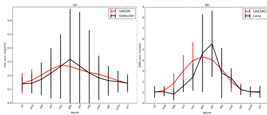
Figure 17. Seasonal comparison averaged over 30^{\circ}\text{S} - 70^{\circ}\text{S} of (a) ocean surface Chl-a concentration and (b) seawater DMS concentration simulated interactively from UKESM1 and observation-based datasets used in GC3.1. The surface Chl-a plotted in (a) and used in Eqn 2 is 0.5 \times Chl-a simulated by the MEDUSA ocean biogeochemistry model, see main text for details.
