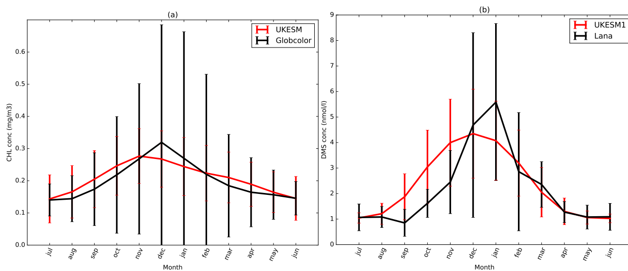
Figure 17. Seasonal comparison averaged over 30^{\circ}\text{S} – 70^{\circ}\text{S} of (a) ocean surface Chl-a concentration and (b) seawater DMS concentration simulated interactively from UKESM1 across 30^{\circ}\text{S} – 70^{\circ}\text{S} . Simulations here are from UKESM1-AMIP and a parallel run with PMOA emissions excluded. Given the low data coverage of satellite retrievals observation-based datasets used in the austral winter the UKESM1 and Bennartz has been spatially sampled according to the Grosvenor product GC3.1. The surface Chl-a plotted in (a) and used in Eqn 2 is 0.5 \times Chl-a simulated by the MEDUSA ocean biogeochemistry model, see main text for details.
