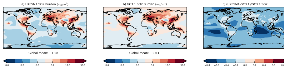
Figure 2. Annual mean \text{SO}_2 burden ( \text{mg}[\text{SO}_2] \text{m}^{-2} ) in (a) UKESM1 and (b) GC3.1 and (c) their relative difference. The annual mean burdens are computed from the 9 and 4 member historical ensemble means from UKESM1 and GC3.1 respectively from years 1980 to 2014 inclusive.
