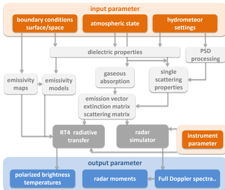
Figure 1. Flowchart of the various steps performed during a PAMTRA simulation. Orange areas describe input parameters given by the user with the Python interface or text files. Gray boxes are the FORTRAN model parts where the various interaction parameters are generated and the radiative transfer or the radar simulator get processed. Blue boxes describe the model output.
