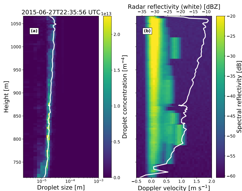
Figure 6. (a) Observed drop size distribution and (b) forward modelled radar Doppler spectrum of the sample cloud of the ACME-V campaign. The white line denote (a) the effective diameter and (b) the radar reflectivity Z_e .
