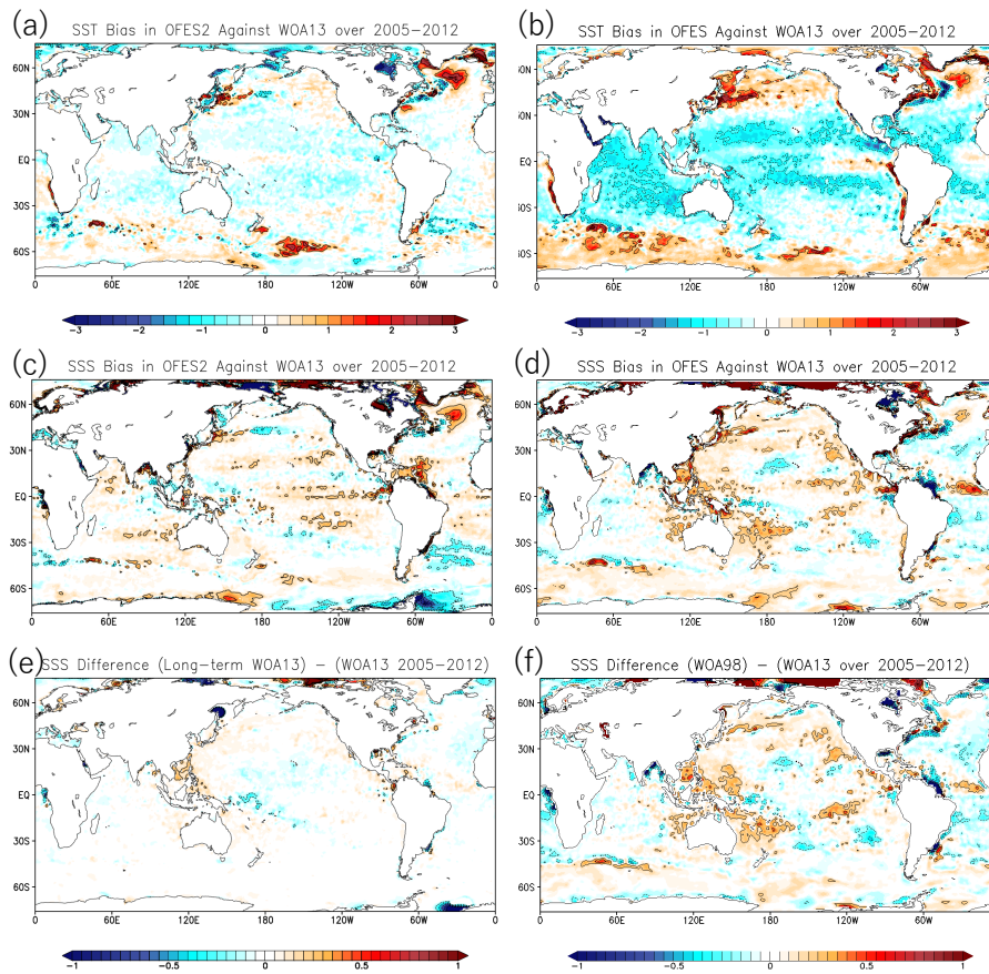
Figure 4: SST bias (°C) in (a) OFES2 and (b) OFES averaged over 2005-2012 against WOA13. (c) and (d) are the same as in (a) and (b), respectively, but the SSS bias is shown instead (psu). SSS differences in (e) long-term WOA13 and (f) WOA98 from WOA13 averaged over 2005-2012. The contour lines are superimposed at an interval of 1 °C for SST and 0.2 psu for SSS, but zero contour lines are omitted.
