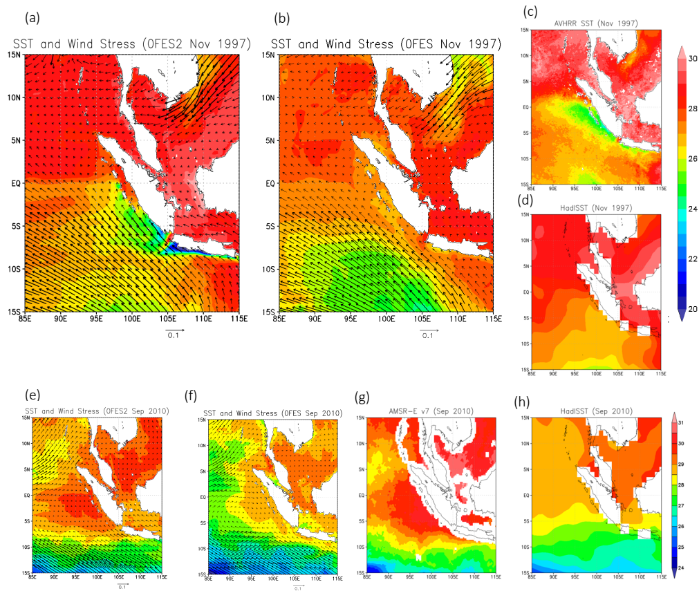
665 Figure 11: SST ( ^{\circ}\text{C} ) in a region including the IOD eastern pole ( 90^{\circ}\text{-}110^{\circ}\text{ E} and 10^{\circ}\text{ S-}0^{\circ} ) in the mature month of (a-d) the 1997 positive IOD event (November 1997) and (e-h) the 2010 negative IOD event (September 2010). (a, e) OFES2, (b, f) OFES, (c, g) satellite observations of AVHRR version 4.1 (Casey et al. 2010) and AMSR-E version 7 (Wentz & Meissner 2007), and (d, h) HadISST ver.1 (Rayner et al. 2003). The vectors in (a, b, e, f) are the surface wind stress ( \text{N m}^{-2} ) in the models, which are plotted at a 1^{\circ}\times 1^{\circ} resolution. The thick vectors denote wind stress magnitudes stronger than 0.05 \text{ N m}^{-2} .
