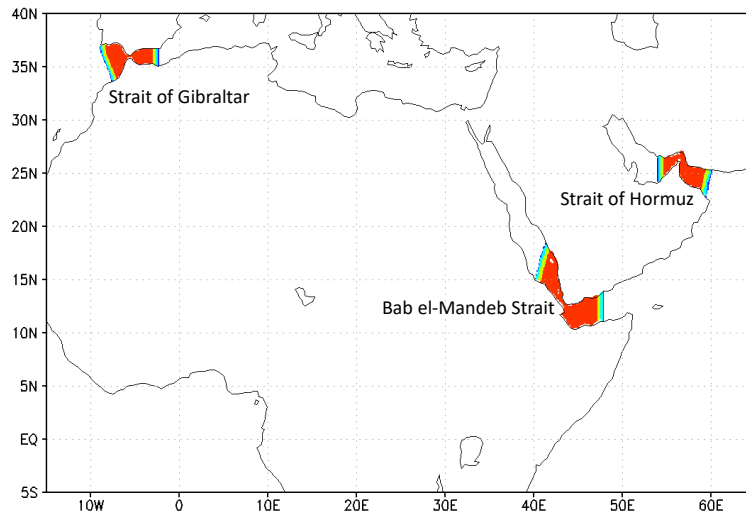
Figure 3: Timescales for restoring the temperature and salinity in and near the Straits of Gibraltar, Hormuz, and Bab el-Mandeb.
