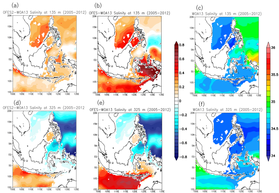
645 Figure 6: Salinity biases (a, b, d, e) against WOA13 (c, f) in OFES2 (a, d), OFES (b, e) at 135 m (a, b, c) and at 325 m (d, e, f). All fields are averaged over 2005-2012, and the units are psu.
