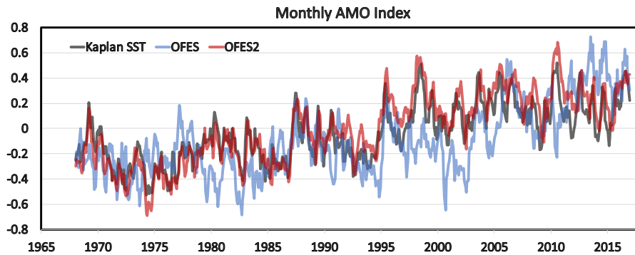
Figure 12: Monthly AMO index defined as SSTAs ( ^{\circ}\text{C} ) in 0^{\circ}\text{S} - 70^{\circ}\text{N} in the eastern tropical Pacific in the Kaplan SST (black curve, Kaplan et al. 1998, https://psl.noaa.gov/data/timeseries/AMO/ ), OFES2 (red curve), and OFES (blue curve).
