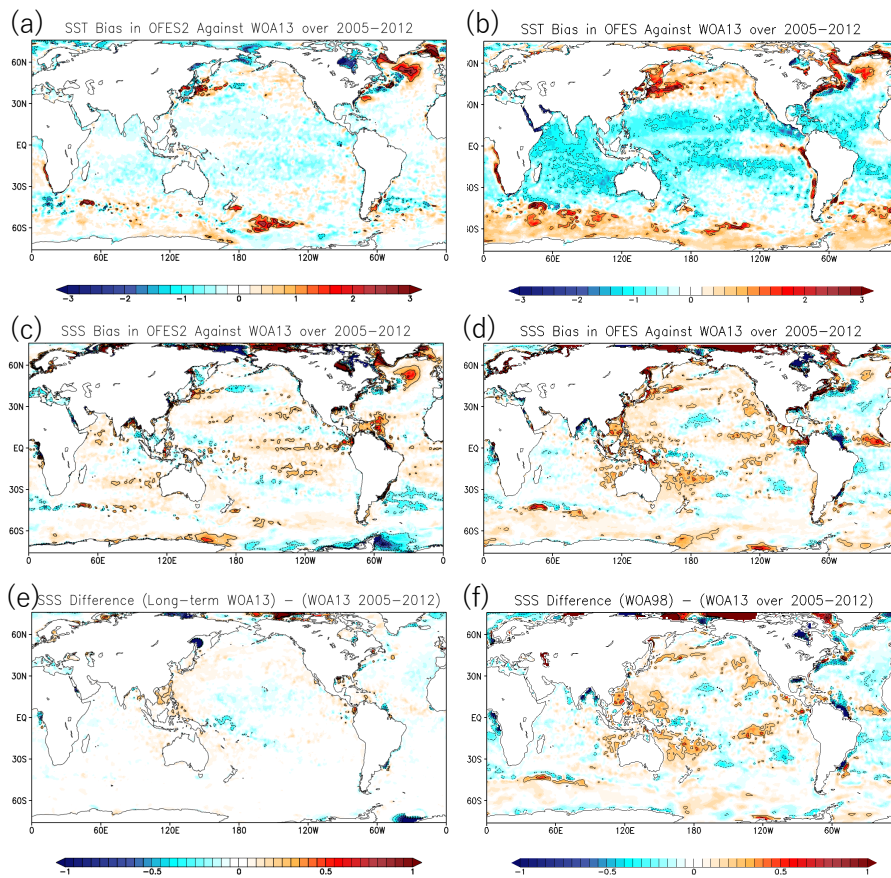
675 Figure 4: SST bias (°C) in (a) OFES2 and (b) OFES averaged over 2005-2012 against WOA13. (c) and (d) are the same as in (a) and (b), respectively, but the SSS bias is shown instead (psu). SSS differences in (e) long-term WOA13 and (f) WOA98 from WOA13 averaged over 2005-2012. The contour lines are superimposed at an interval of 1 °C for SST and 0.2 psu for SSS, but zero contour lines are omitted.
