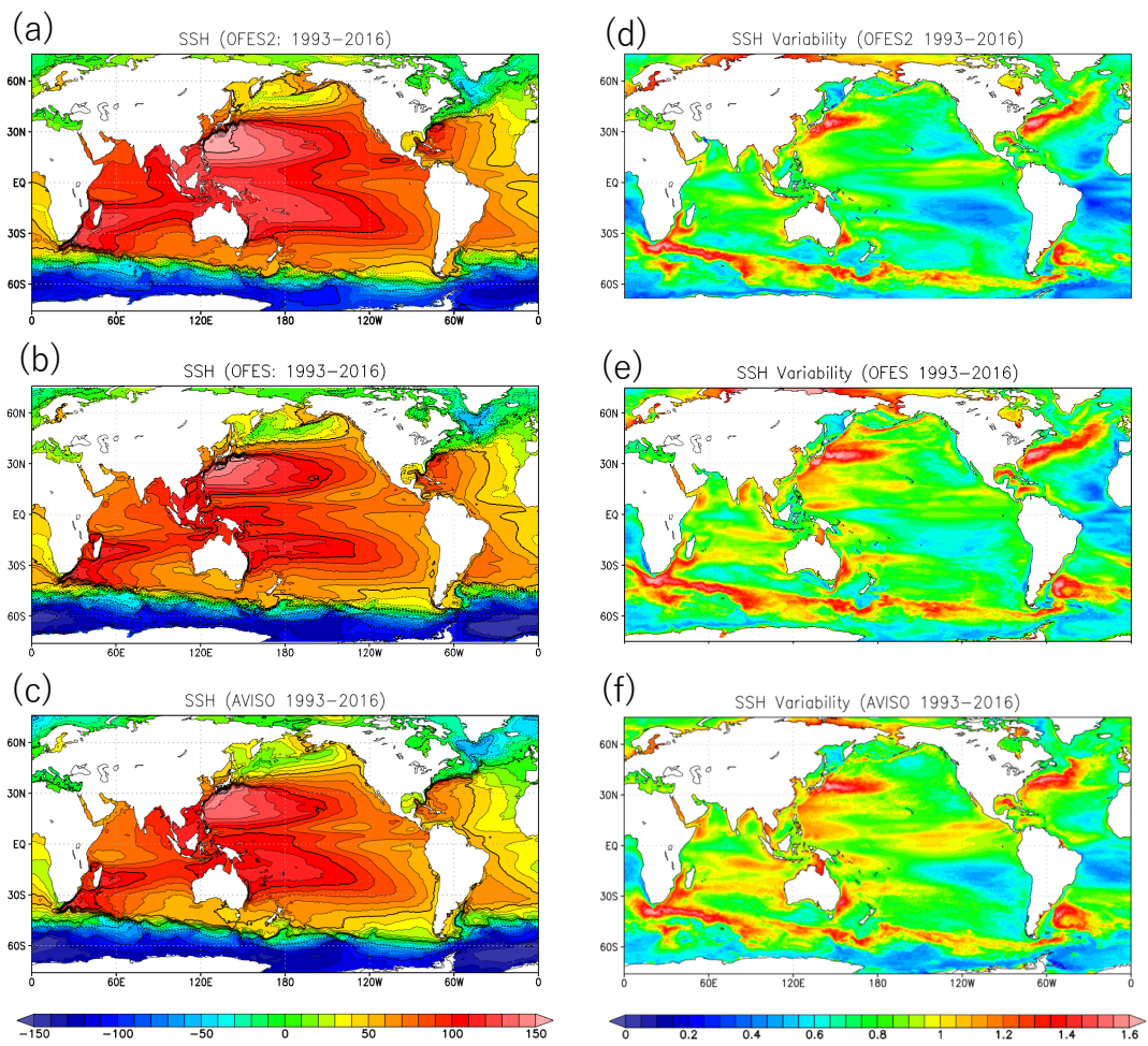
680 Figure 5: Mean (a, b, c) SSH (cm) and (d, e, f) its standard deviation (log10 cm) averaged over 1993-2016 from (a, d) OFES2, (b, e) OFES, and (c, f) AVISO observations. The SSH in OFES2 and OFES was offset by adding 50 cm.
