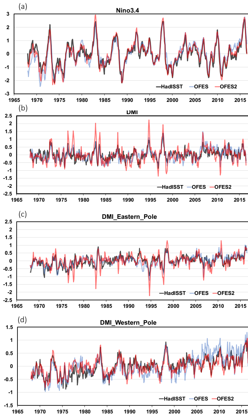
Figure 10: (a) Monthly Niño3.4 index defined as SSTAs ( ^{\circ}\text{C} ) in 165^{\circ}\text{--}145^{\circ}\text{W} and 5^{\circ}\text{S--}5^{\circ}\text{N} in the eastern tropical Pacific and (b) the monthly DMI ( ^{\circ}\text{C} ) defined as difference between the SSTAs ( ^{\circ}\text{C} ) in the (c) eastern ( 90^{\circ}\text{E--}110^{\circ}\text{E} , 10^{\circ}\text{S--}0^{\circ} ) and (d) the western ( 50^{\circ}\text{--}70^{\circ}\text{E} and 10^{\circ}\text{S--}10^{\circ}\text{N} ) poles (Saji et al. 1999) from OFES2 (red curve), OFES (blue curve), and HadISST version 1 (black curve, http://www.cpc.ncep.noaa.gov/data/indices/ and http://www.jamstec.go.jp/frcgc/research/d1/iod/iod/dipole_mode_index.html ).
