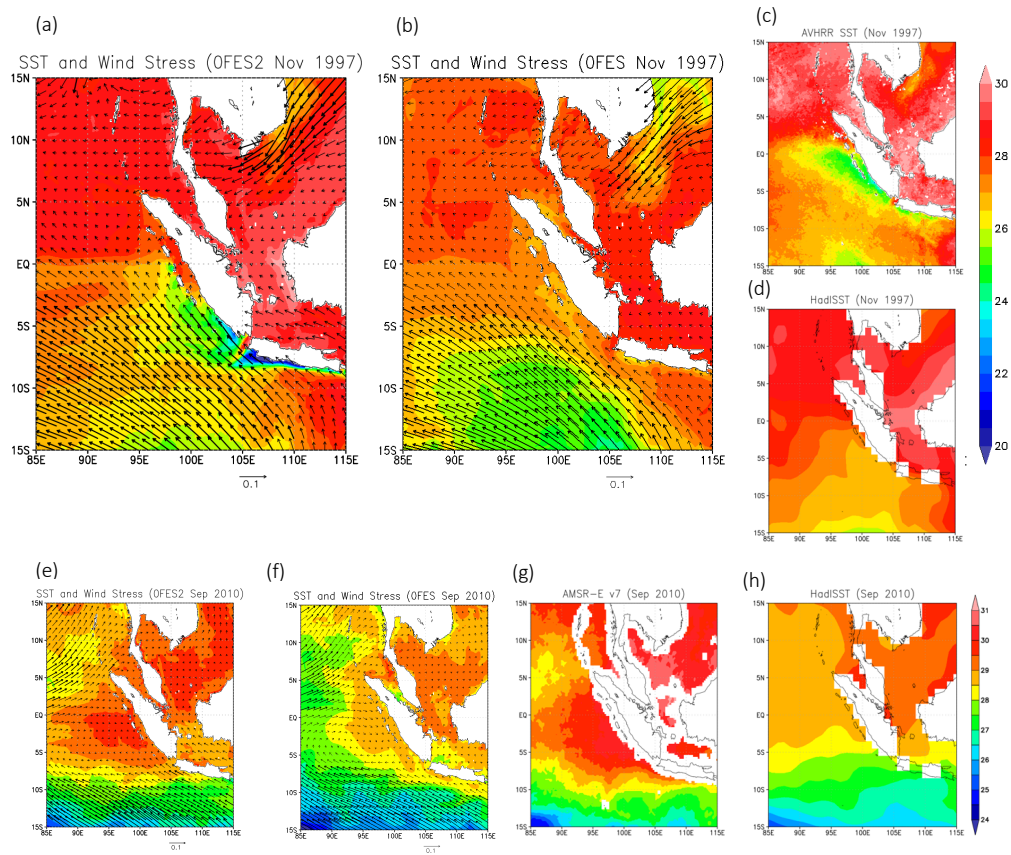
705 Figure 11: SST ( ^{\circ}\text{C} ) in a region including the IOD eastern pole ( 90^{\circ}\text{-}110^{\circ}\text{ E} and 10^{\circ}\text{ S-}0^{\circ} ) in the mature month of (a-d) the 1997 positive IOD event (November 1997) and (e-h) the 2010 negative IOD event (September 2010). (a, e) OFES2, (b, f) OFES, (c, g) satellite observations of AVHRR version 4.1 (Casey et al. 2010) and AMSR-E version 7 (Wentz & Meissner 2007), and (d, h) HadISST ver.1 (Rayner et al. 2003). The vectors in (a, b, e, f) are the surface wind stress ( \text{N m}^{-2} ) in the models, which are plotted at a 1^{\circ}\times 1^{\circ} resolution. The thick vectors denote wind stress magnitudes stronger than 0.05 \text{ N m}^{-2} .
