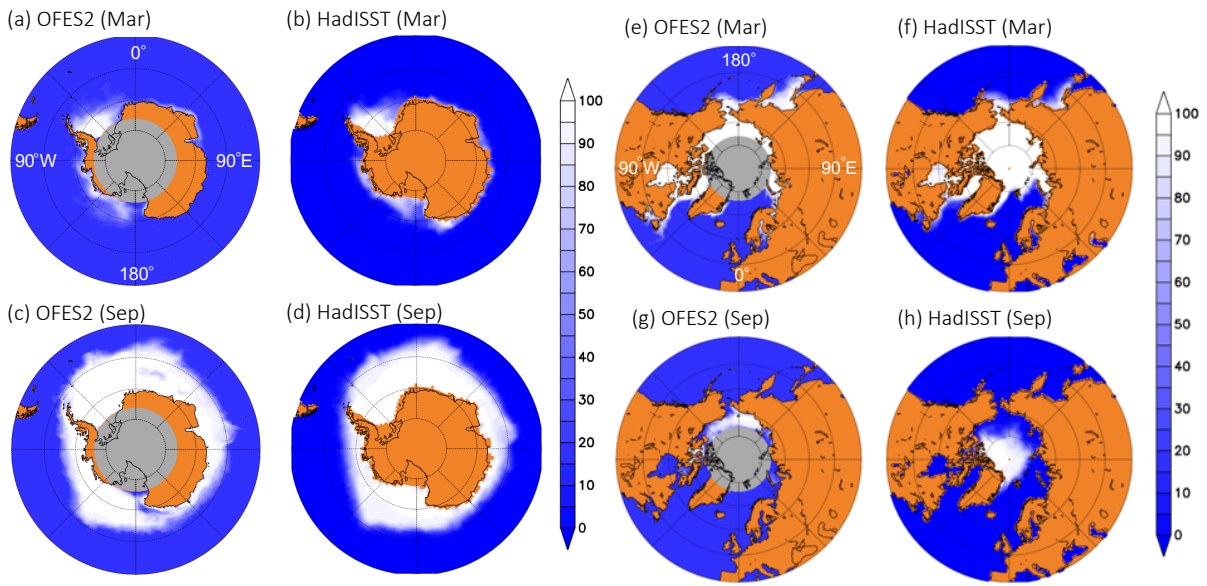
695 Figure 9: Sea-ice concentrations (%) in the Antarctic Ocean in (a, b) March and (c, d) September in (a, c) OFES2 and (b, d) HadISST averaged over 2005-2012. Similarly, the sea-ice concentrations in Arctic Ocean in (e, f) March and (g, h) September in (e, g) OFES2 and (f, h) HadISST. The gray areas are out of the model domain in OFES2 (a, c, e, g).
