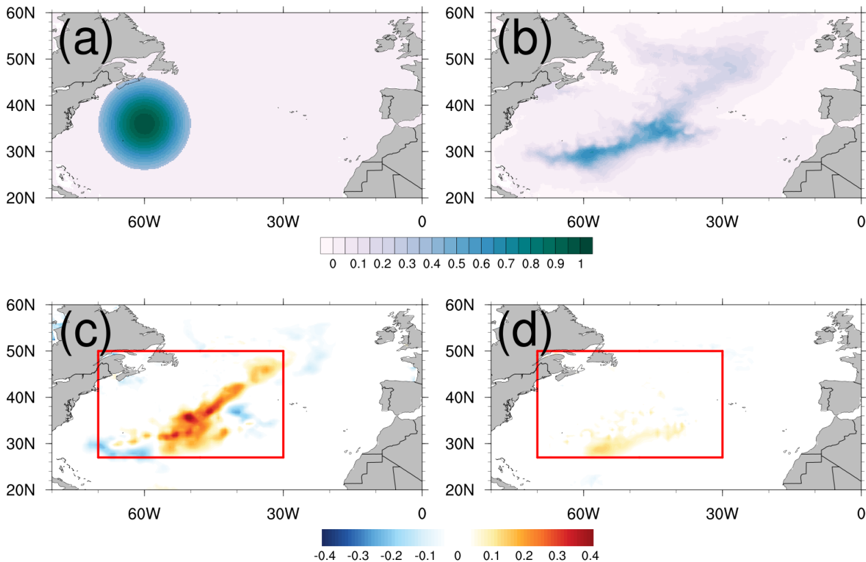
Figure 6. Passive tracer Initial condition for PATCH experiment (a), tracer concentration at 16 m depth after one year for HR configuration (b) and difference with respectively LR (c) and HRCRS configurations (d).
