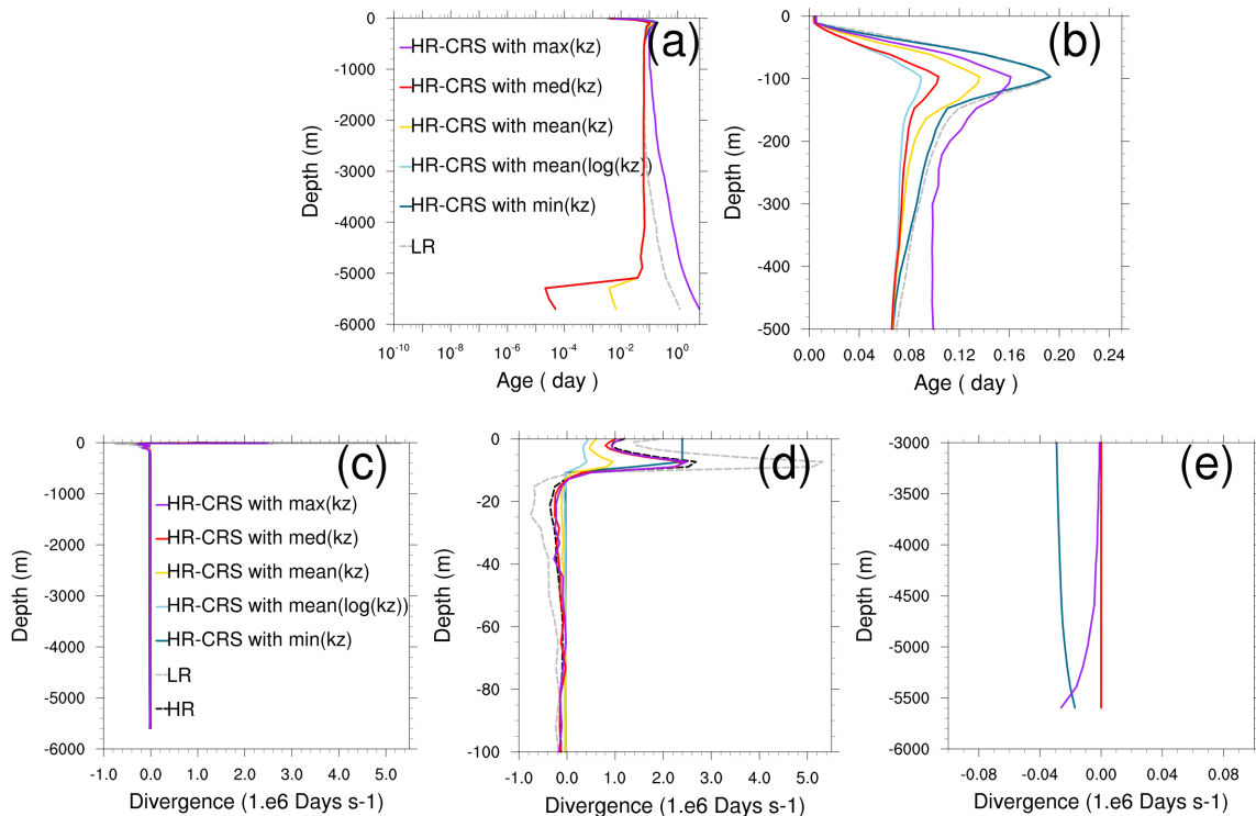
Figure 8. Top: RMS differences to HR Age tracer for HRCRS & LR runs for the whole water column (a) and for the first 500 meters (b). Age Tracer values are instantaneous outputs after one years. Bottom: Horizontal mean of divergence of Age tracer vertical diffusive fluxes mean over the first year for the whole water column (c), the top ocean (d) and the bottom ocean (e).
