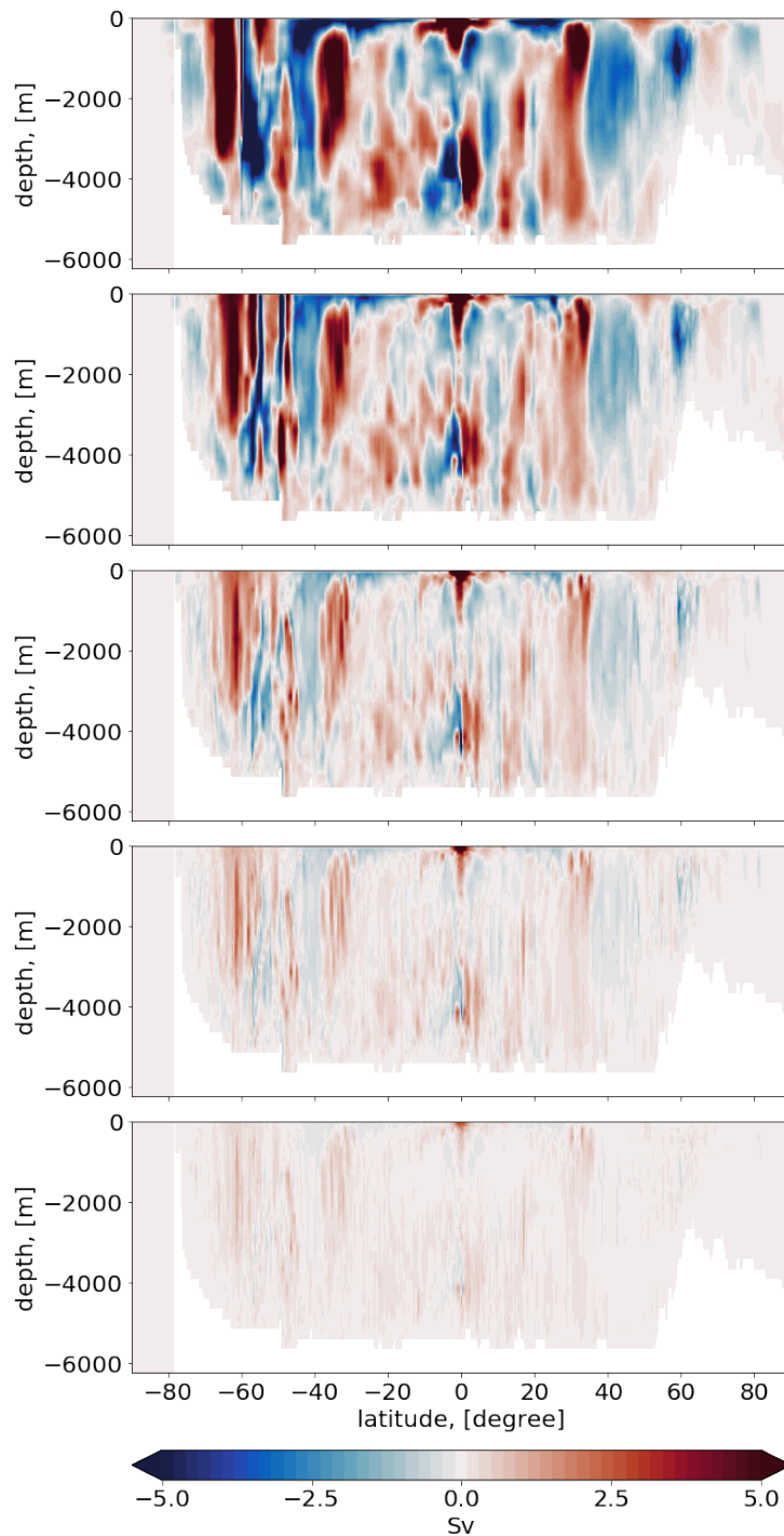
Figure 4. Differences in MOC computed with bins \Delta\theta = 4^\circ, 2^\circ, 1^\circ, 0.5^\circ, 0.25^\circ (from top to the bottom) relative the MOC computed with \Delta\theta = 0.125^\circ . Evidently there is a convergence with decreasing bin size.
