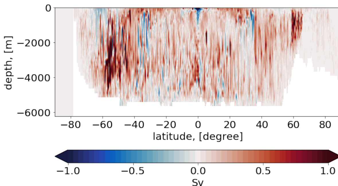
Figure 7. Differences between computations of MOC using meridional or vertical velocities. The discrepancy between techniques may result in differences of more than 1 Sv.
