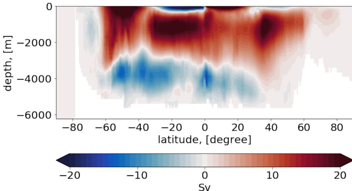
Figure 3. Global Meridional Overturning Circulation (MOC) streamfunctions including the eddy induced transports. The streamfunctions depicts a canonical pattern as known from the literature with a maximum of 20Sv at 45°N.
