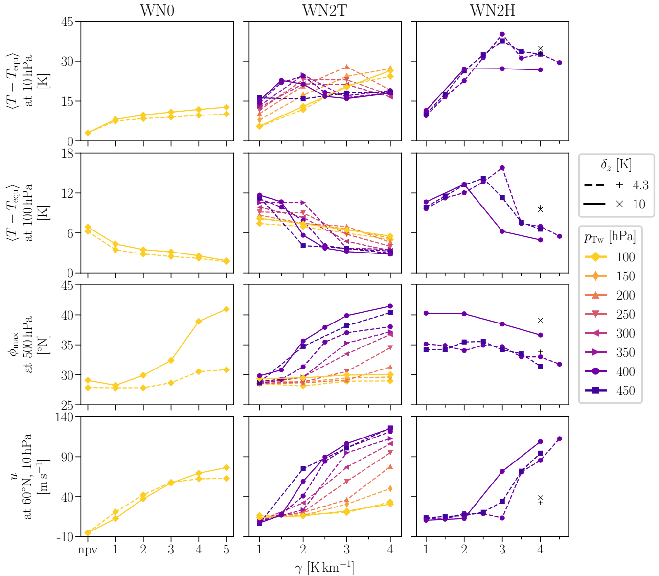
Figure 8. Top row: Difference of temperature and equilibrium temperature T - T_{\text{eq}} averaged from 40^{\circ}\text{N} to 90^{\circ}\text{N} at 10 hPa. Second row: same, but at 100 hPa. Third row: Latitude \phi_{\text{max}} of the zonal mean zonal wind speed maximum of the tropospheric jet. Fourth row: zonal mean zonal wind u at 60^{\circ}\text{N} and 10 hPa. The left column shows results from model simulations without planetary wave forcing, the middle column with WN2 topography of height h = 3 km and the right column with WN2 tropospheric heating of amplitude q_0 = 6 \text{ K day}^{-1} . Solid lines represent simulations with standard \delta_z = 10 \text{ K} , dashed lines with reduced \delta_z = 4.3 \text{ K} .
