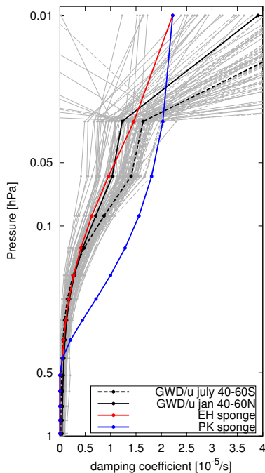
Figure 6. Damping coefficient [ s^{-1} ] of the sponge layer in the “EH” (red) and in the PK02 set-up (blue) together with the effective damping time scale of the zonal winds by gravity wave drag (i.e., -\text{GWD}/u ) from an ECHAM simulation with a non-orographic and orographic GW scheme, averaged over 40\text{-}60^\circ\text{S} in July 1960 to 2010 (gray dashed, average over all years shown as black dashed) and averaged over 40\text{-}60^\circ\text{N} in January 1960 to 2010 (gray solid, average over all years shown as black solid).
