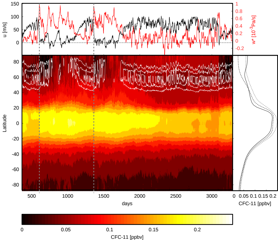
Figure 12. Top: time series of zonal mean zonal wind \bar{u} at 60°N and 10 hPa (black) and mean \bar{w}^* at 50 hPa and 60°-90°N (red). Middle panel: zonal-mean CFC-11 mixing ratios (color, in ppbv) at 50 hPa as function of simulated day and latitude, and zonal mean zonal wind at 50 hPa (white contours, interval 15 \text{ms}^{-1} ). Vertical gray lines mark dates of SSW (centered here at the dates of the strongest wind decelerations). Right: time-mean CFC-11 mixing ratios as function of latitude over days with strong vortex (days 400-600; 1200-1350; 2000-3000, black solid), over days following SSW with strong downwelling (day 600-780; 1380-1500; 3100-3280, dashed) and over days with eroded polar vortex (day 800-1000 and 1580-1700, dotted).
