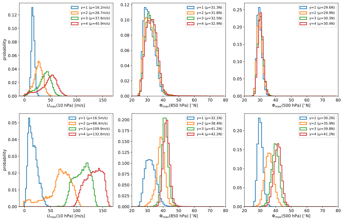
Figure C2. As Fig. C1, but for simulations with standard PK set-up and WN2 topography (top) for p_{\Gamma W} = 100 hPa, and (bottom) for p_{\Gamma W} = 400 hPa.
