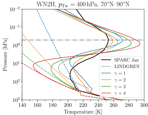
Figure 10. Same as Fig. 9, but for model simulations with WN2 tropospheric heating of amplitude q_0 = 6 \text{ K day}^{-1} and different polar vortex lapse rates \gamma for p_{T_w} = 400 \text{ hPa} . The temperature profiles obtained from a simulation with the original Lindgren set-up (black dotted line) are added for comparison.
