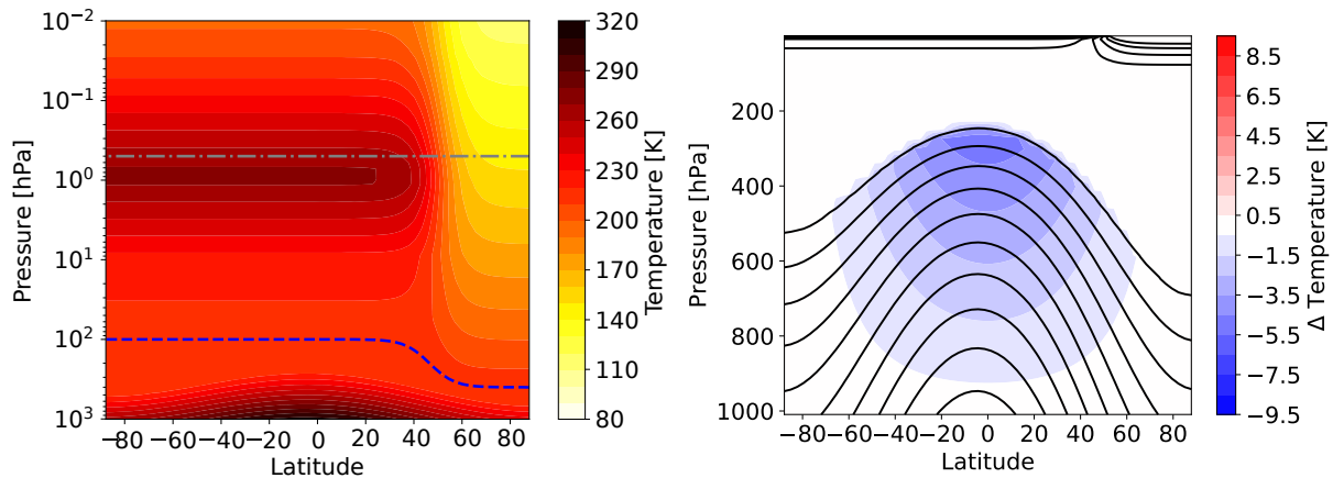
Figure 2. Left: Equilibrium temperature (in K) for p_{\Gamma w} = 400 hPa and \gamma = 2 K km ^{-1} together with the transition pressure p_{\Gamma}(\phi) (blue dashed line) and the pressure above which damping sets in (gray dashed-dotted line). Right: T_{\text{eq}} as given by the original PK02 implementation (black contours) and difference in T_{\text{eq}} between simulations with reduced \delta_z = 4.3 K and with standard \delta_z = 10 K (colors).
