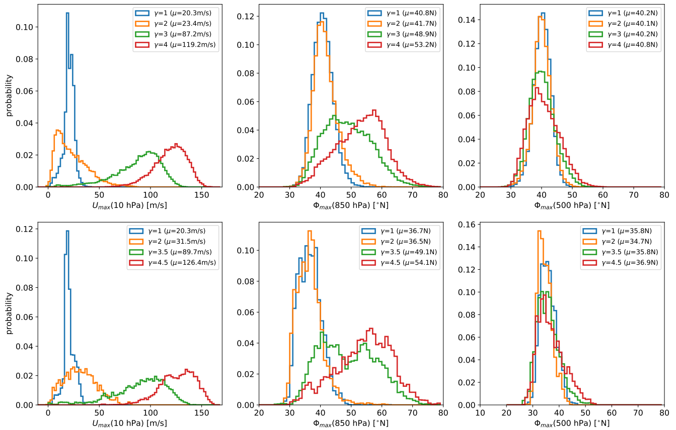
Figure C3. As Fig. C1, but for simulations with WN2 heating and p_{T_w} = 400 \text{ hPa} for (top) the standard set-up and (bottom) the modified set-up with reduced \delta_z .
