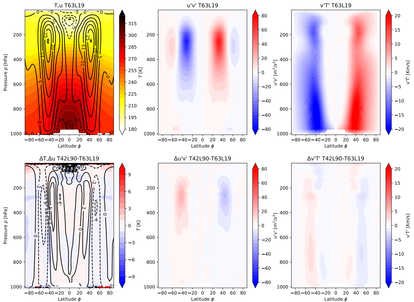
Figure 3. Top: Results from a HS simulation at T63L19 resolution, showing mean temperature [K] and zonal mean zonal wind [ \text{m s}^{-1} , contour interval 5 \text{ m s}^{-1} ] (left), mean eddy momentum fluxes [ \text{m}^2 \text{ s}^{-2} ] (middle) and mean eddy heat fluxes [ \text{K m s}^{-1} ] (right) averaged over 1500 days (after spin-up of 325 days). Bottom: As above, but difference of a simulation at T42L90MA resolution minus the T63L19 simulation (with wind contour interval 2 \text{ m s}^{-1} ).
