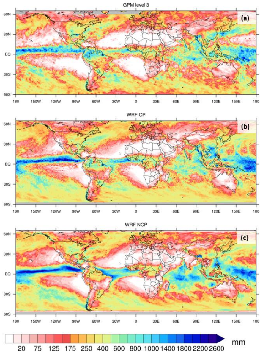
Fig. 6: Accumulated precipitation [mm] from April to June 2015: (a) Global Precipitation Mission (GPM) level 3 data set, (b) CP simulation, (c) NCP simulation. Grey shaded areas indicate lacking coverage in the GPM data or the simulations. The model data are interpolated to the GPM mesh.
