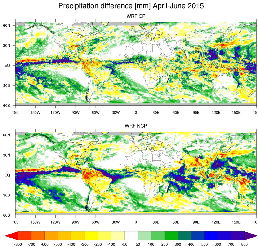
Fig. 7: Precipitation difference [mm] between CP and GPM (upper panel) and difference between NCP and GPM (lower panel).
