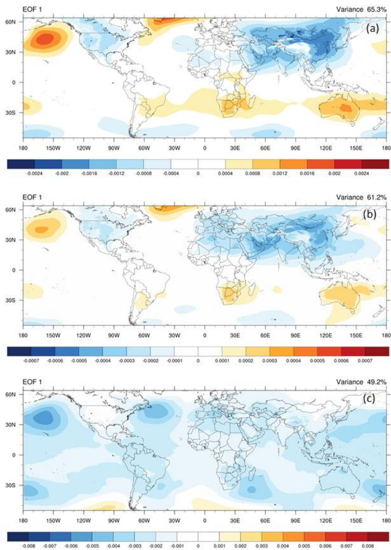
Fig. 8: 1 st EOF analyses of the monthly mean sea level pressure for the ECMWF operational analysis (a), the CP simulation (b) and the NCP simulation (c) over the whole forecast period. Normalized values are shown and the averaging time steps are 00 UTC, 06 UTC, 12 UTC, and 18 UTC to match the ECMWF analysis time steps.
