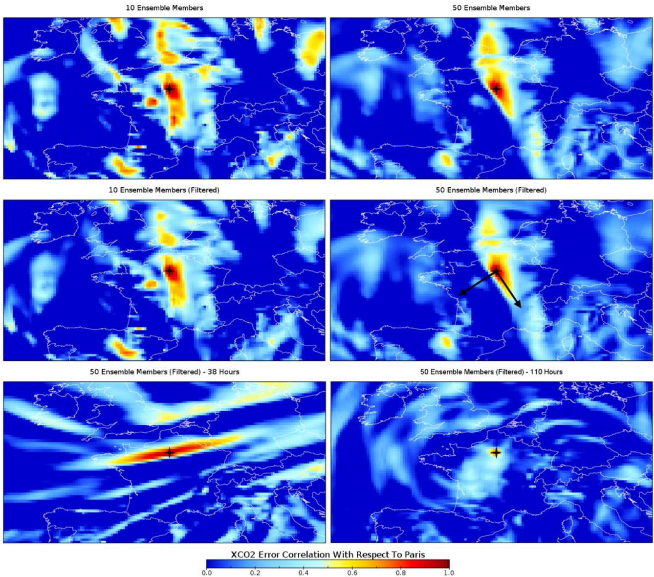
Figure 7. A snapshot of regional XCO 2 error correlation structure with respect to Paris XCO 2 from 10 (top left) and 50 (top right) member IFS model ensemble after 4 days, where the ensemble consists of perturbed initial meteorology and model physics (transport error). The middle-row shows the same as the top-row but includes the preceding and subsequent model time steps ( \pm 1 hour), artificially increasing the correlation sample to 30 and 150 members. The bottom row shows the same correlation calculations as the middle-right panel (150-member consisting of \pm 1 hour) but for two different times; highlighting the flow-dependence in error correlation structure. The star denotes the column over Paris and the black arrows denote the down- and across-wind directions used to calculate the further and shortest correlation lengths for a given time (see Figure 8).
