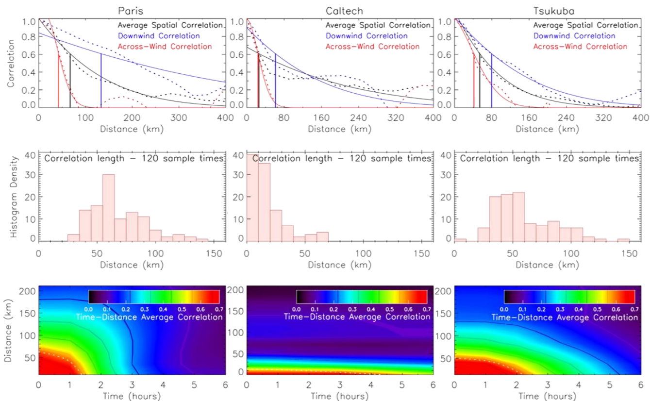
630 Figure 8. A snapshot of XCO 2 error correlation with respect to Paris (left), Caltech (middle) and Tsukuba (right) as a function of distance for a 50-member IFS model ensemble after 4 days (top row). These panels show the directionally averaged (black dashed line), downwind (blue dashed line) and across-wind (red dashed line) correlation values are shown with a gaussian fit (solid lines) in addition to the derived correlation length where R = e^{-0.5} (vertical solid lines). The directionally averaged derived correlation lengths for 120 sample times for January 2015 are placed in 10km bins for all three sites (middle row). The directionally and time averaged error correlation values for the same 120 sample sizes as a function of both time and distance (bottom row).
