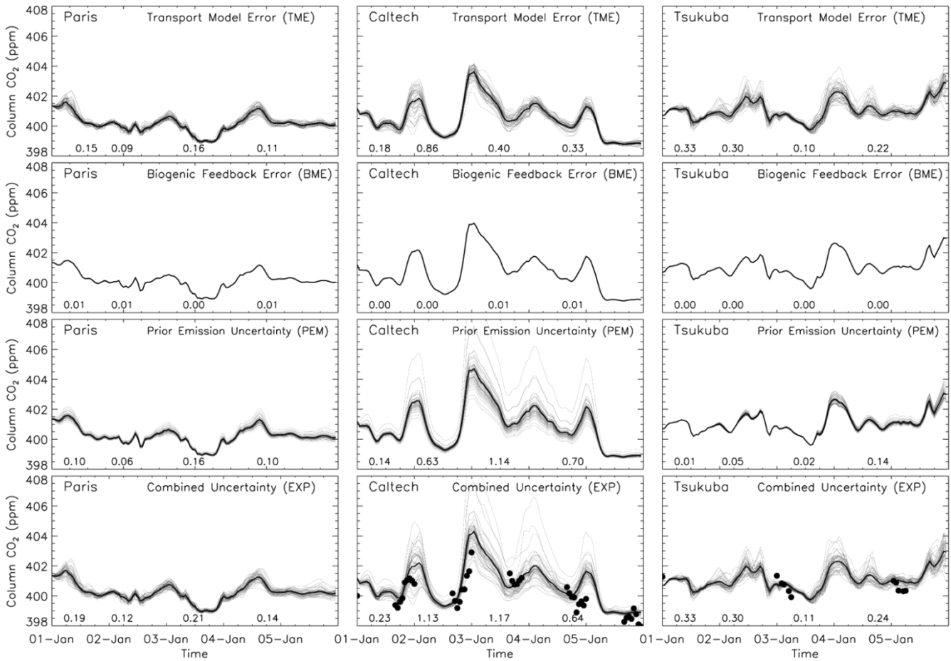
585 Figure 1. IFS model XCO 2 (ppm) variability over three TCCON sites for 50-member ensemble for 1-5 th January 2015 from uncertainties in model transport (first row), biogenic feedback from meteorological uncertainty (second row), monthly uncertainties in anthropogenic emissions (third row) and a combination of all uncertainties (fourth row). Individual ensemble members are shown with grey lines and the ensemble mean is the black line. TCCON observations, when available, are shown for the 5 days (black circles). Values denote standard error after 12, 24, 48 and 96 hours.
