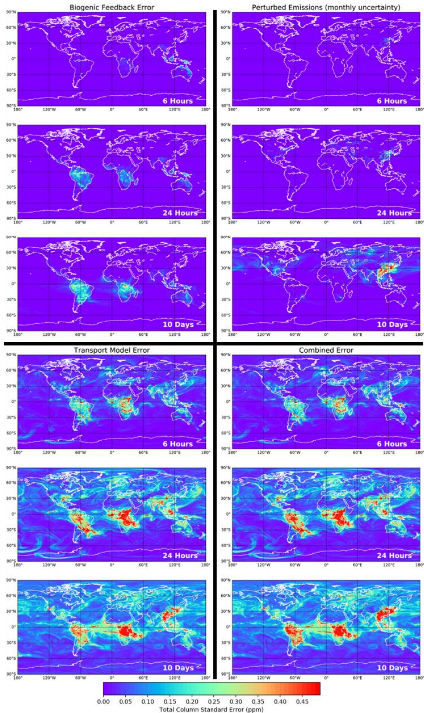
605 Figure 4. Global standard error of IFS model XCO 2 (ppm) across 50-member ensemble after 6 hours, 24 hours and 10 days. Errors shown are from uncertainties in biogenic emissions caused by meteorological uncertainty (top left), monthly anthropogenic emission uncertainties per sector and country (top right), model transport uncertainty (bottom left) and a combination of all uncertainties (bottom right).
