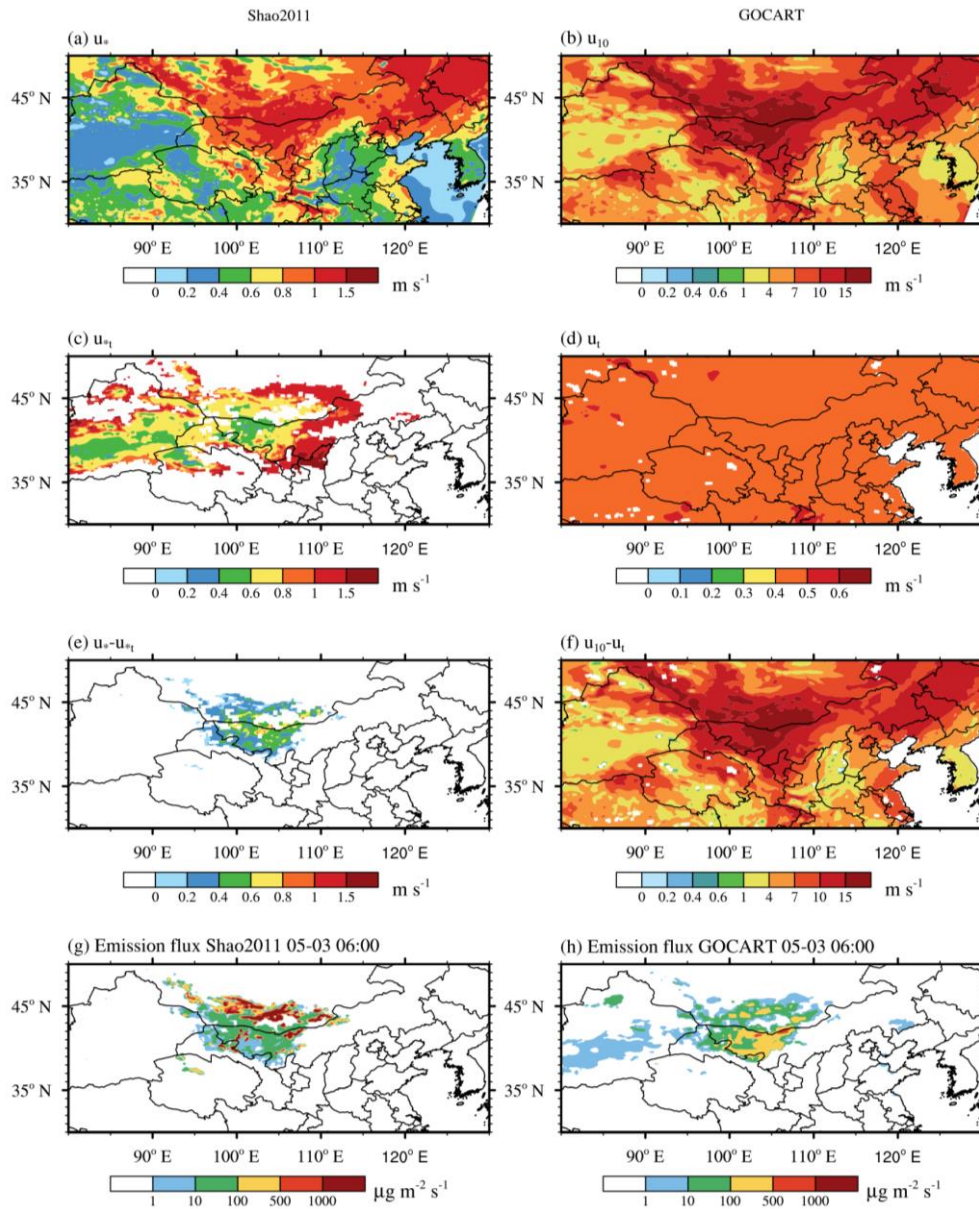
945 Figure 5. Spatial distribution of (a) friction velocity ( u_* ), (c) threshold friction velocity ( u_{*t} ) and (e) the difference between u_* and u_{*t} ( u_* - u_{*t} ) from Shao2011 dust emission scheme at 06:00 UTC on 3 May, 2017; (b) wind speed at 10 meters ( u_{10} ), (d) threshold velocity ( u_t ) and the difference between u_{10} and u_t ( u_{10} - u_t ) from GOCART dust emission scheme at 06:00 UTC on 3 May, 2017. Spatial distribution of (g) dust emission flux from Shao2011, (h) dust emission flux from GOCART at 06:00 UTC on 3 May, 2017.
