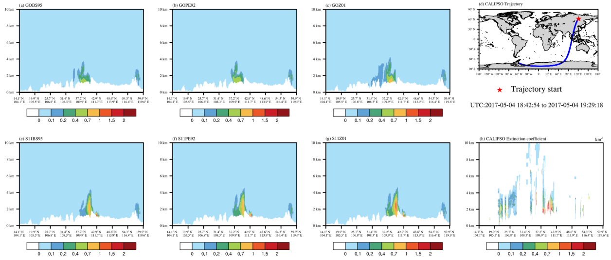
Figure 10. Simulated and observed aerosol extinction profiles at 532 nm at 18:00 UTC 4 May. Panel (d) show the CALIPSO trajectory. Panel (h) show the CALIPSO observed extinction coefficient. Panels (a)(b)(c)(e)(f)(g) show the WRF-Chem simulated extinction coefficient from six experiments.
