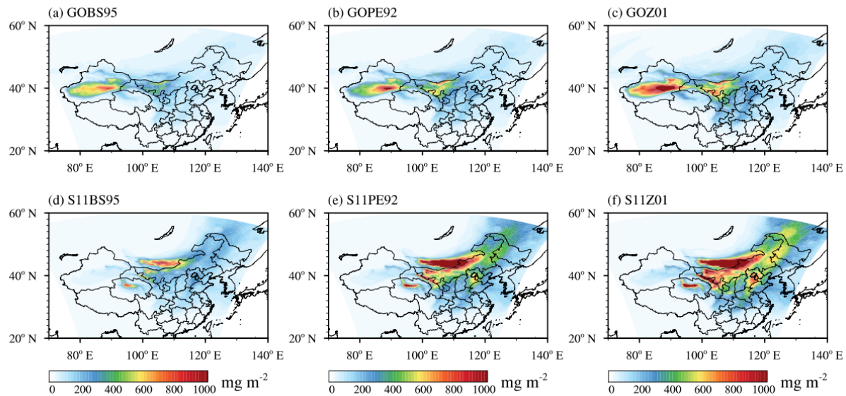
Figure 3. Spatial distribution of simulated mean dust loading for six experiments (a)GOBS95, (b)GOPE92, (c)GOZ01, 925 (d)S11BS95, (e)S11PE92, (f)S11Z01 over the 7-day simulation period from 00:00 UTC on 1 May to 23:00 UTC on 7 May, 2017 (unit: \text{mg m}^{-2} ).
