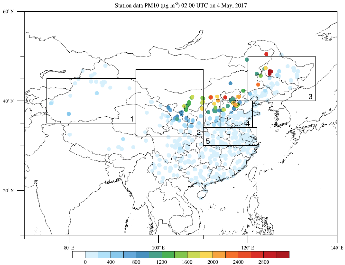
960 Figure 7. Five sub regions and observed PM 10 concentrations. “1” represents the Taklimakan Desert (TD), “2” represents the Gobi Desert (GD), “3” represents the Northeastern plain (NEP), “4” represents the North China Plain (NCP), “5” represents the Middle and lower reaches of Yangtze River Plain (YR). The colored dots represent observed PM 10 concentrations over observational sites at 02:00 UTC on 4 May, 2017 (10:00 Beijing Time (BJT) on 4 May, 2017).
