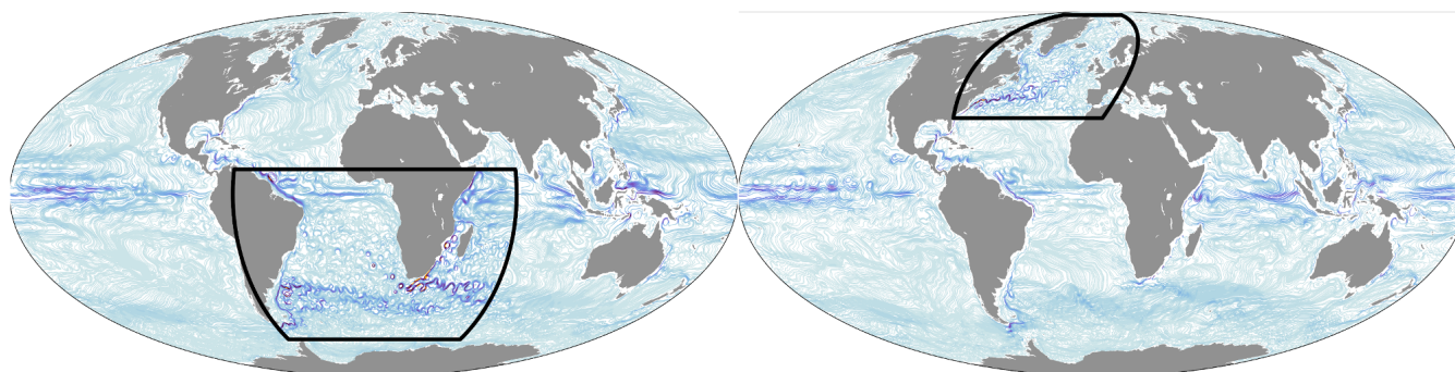
Figure 2. Snapshots of upper ocean current speed (upper 100m averaged) for two separate ocean nest configurations, where ocean resolution refines from 1/2° to 1/10° in the highlighted regions. Left: INALT10X, South Atlantic nest between 9°N - 63°S, 70°W - 70°E, Right: VIKING10, North Atlantic nest between 30°N - 85°N.
