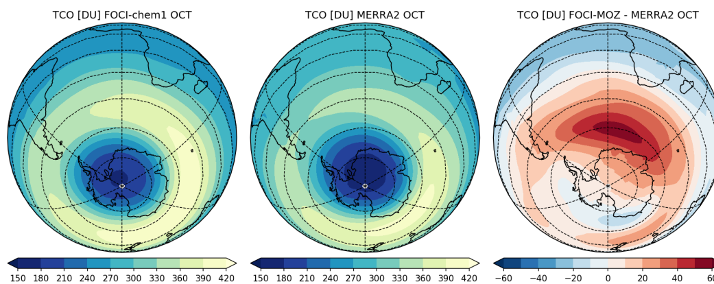
Figure A4. Mean TCO distribution in the SH in October in (a) the FOCI-chem1 simulation, (b) the MERRA2 reanalysis, and (c) the differences between (a) and (b) from 1980 to 2013.
