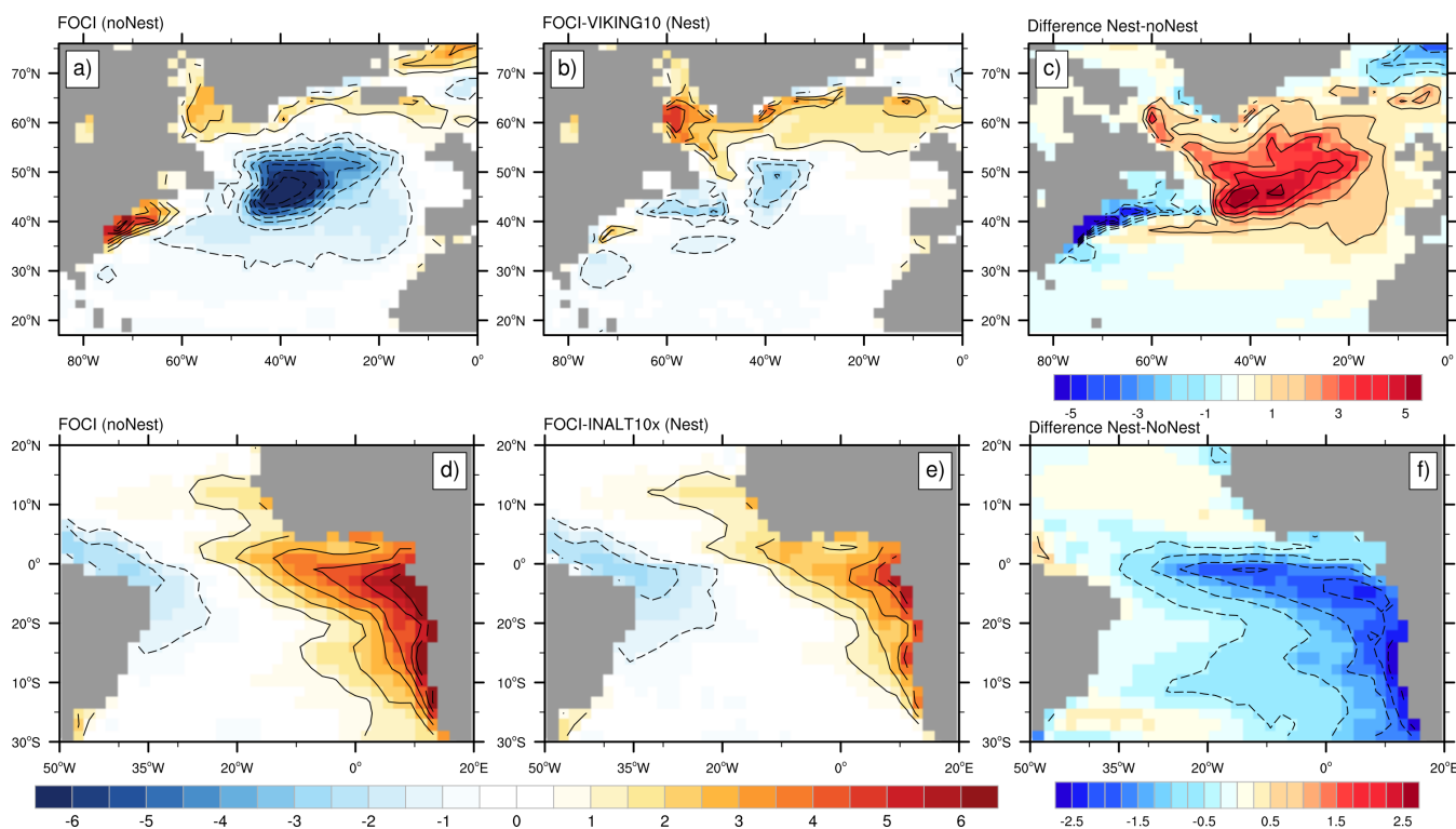
Figure 16. FOCI SST anomalies with respect to observed SSTs (HadISST, 1870-1900) in Kelvin: (a) annual mean FOCI unnested and (b) FOCI_VIKING10-piCTL nested configuration in the North Atlantic; boreal summer (July–Sept.). (d) FOCI-piCTL unnested and (e) FOCI_INALT10X-piCTL nested configuration in the tropical Atlantic. Shared color scale for (a-b),(d-e), contour interval of 1 K for (a-e) and 0.5 K for (f). The global mean SST has been removed from FOCI as well as HadISST data prior to anomaly calculations to eliminate the influence of different mean states.
