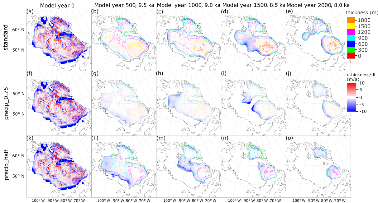
Figure 10. Laurentide Ice Sheet thickness evolution in the three simulations with varying precipitation fields in 500 -year intervals. (a)–(e) 'standard', (f)–(j) 'precip_0.75' (P field in 'standard' multiplied by 0.75), and (k)–(o) 'precip_half' (P field in 'standard' halved).
