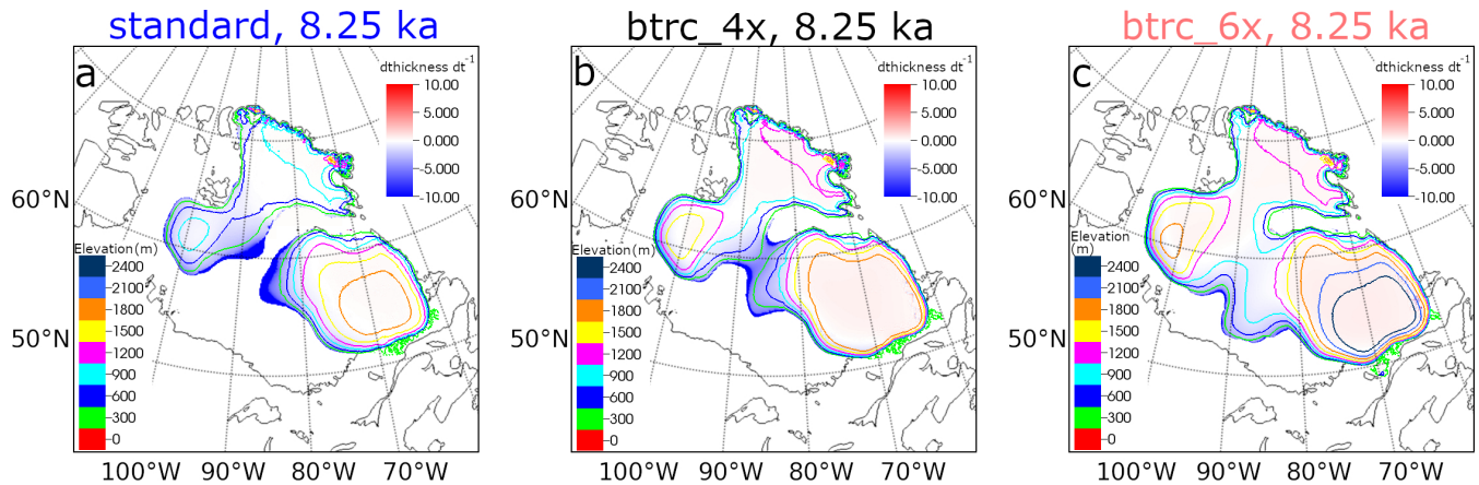
Figure 8. Modelled ice thickness and rate of change of thickness (m a -1 ) at 8.25 ka in (a) the 'standard' simulation, (b) the 'btrc_4x' simulation in which the standard basal traction coefficient field is quadruple, and (c) 'btrc_6x' in which the standard basal traction coefficient field is multiplied by 6.
