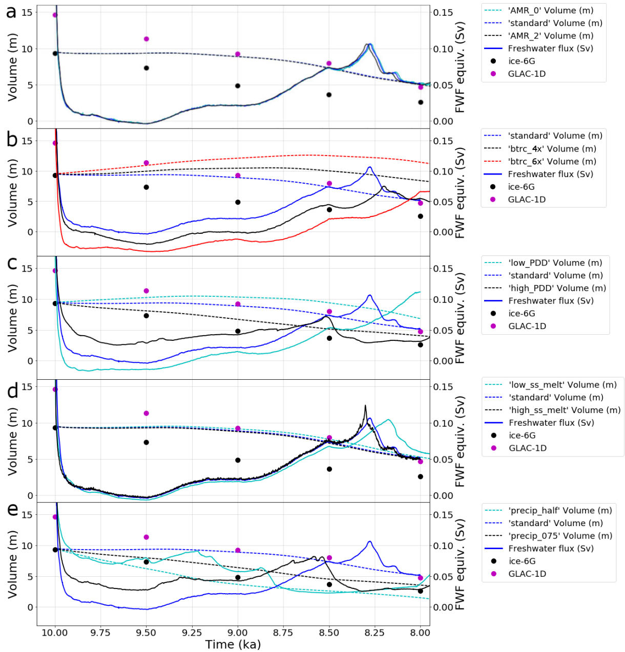
Figure 6. Effects of varying (a) adaptive mesh resolution, (b) basal traction coefficient C, (c) PDD (positive-degree-day coefficients), (d) sub-shelf melting rate and (e) precipitation on simulated ice sheet volume in meters of sea level rise equivalent, and freshwater flux equivalent in Sverdrups. The black and magenta markers show the volume in metres of equivalent sea level rise (SLR) in the ICE-6G_c (VM5a; Peltier et al., 2015), and the GLAC-1D (Tarasov et al., 2012) reconstructions.
