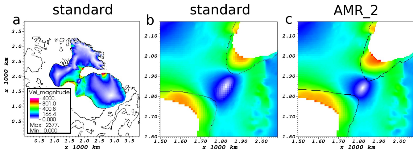
Figure 7. Magnitude of vertically integrated ice velocity ( \text{m a}^{-1} ) at model year 1700 with the grounding line and coastlines shown in black. The three panels follow the scale shown in panel a . (a) The velocity over the whole domain in the 'standard' simulation. (b) A zoomed-in view of the ice saddle in 'standard', and (c) in 'AMR_2' simulations.
