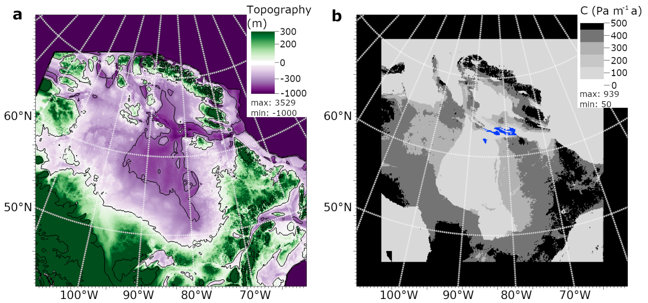
Figure 1. (a) The ‘ETOPO 10 ka’ topography map centred at Hudson Bay on a 10 km grid. The basal topography in the northern part of the grid (Greenland and Canadian archipelago) is set to -1000 m to avoid ice sheet formation in these regions. The black lines show contours every 400 m. (b) Basal traction coefficient map used in the ‘standard’ simulation. The basal traction coefficient ( C ) values are calculated based on bedrock elevation and sediment coverage. The domain was divided into three different types of sediment coverage: bare bedrock, sediment-covered and submerged bare bedrock in the Hudson Strait (highlighted in blue, C = 80 \text{ Pa m}^{-1} \text{ a} ). The outermost 35 grid cells along both axes are initialised with a high basal traction coefficient ( C = 450 \text{ Pa m}^{-1} \text{ a} ) to avoid ice flow reaching the edges of the domain.
