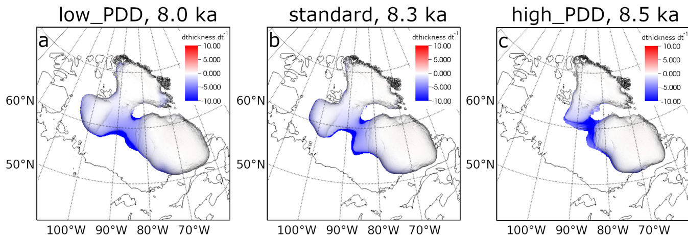
Figure 9. Laurentide Ice Sheet at the approximate time of the peak freshwater flux in the (a) 'low_PDD' simulation, (b) 'standard' simulation, (c) 'high_PDD' simulation. The separation of the Keewatin and Labrador domes in the 'standard' and 'high_PDD' simulations is at a more advanced stage at the time of peak freshwater flux compared to the 'low_PDD' simulation. The freshwater flux in 'low_PDD' would likely have increased as the separation of the ice domes would have continued if the simulation was run for longer than 2000 years.
