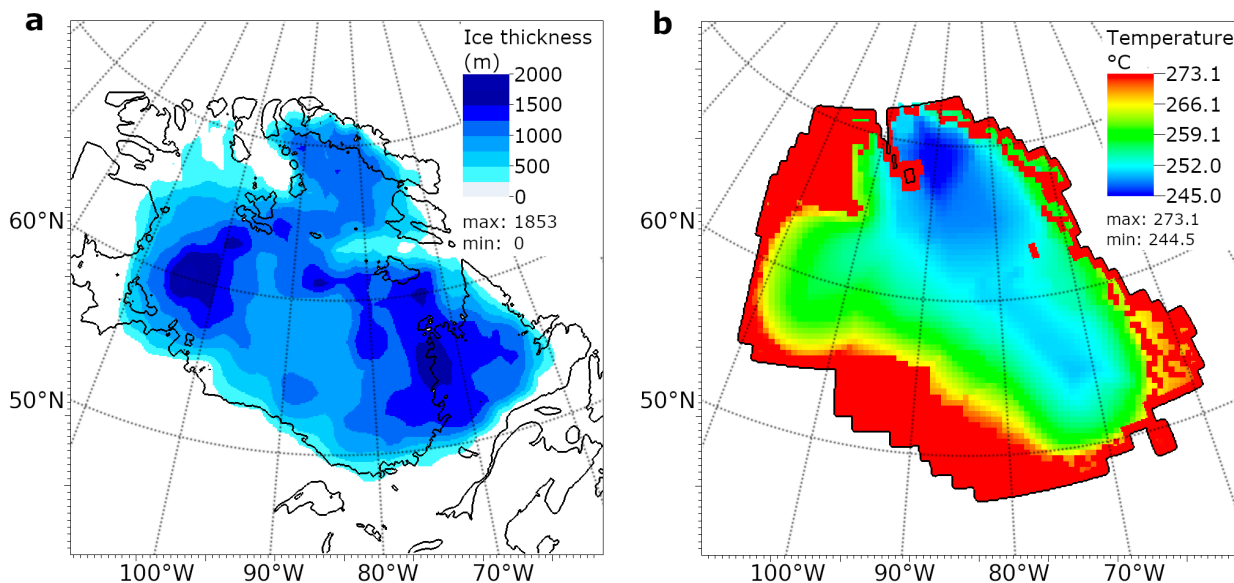
Figure 2. (a) Initial ice thickness (based on ICE-6G_c 10 ka time slice; Peltier et al., 2015), with the coastline shown in black. (b) Initial ice temperature at the lowest level of the ice sheet (based on 9 ka time slice of the simulation by Gregoire et al., 2012).
