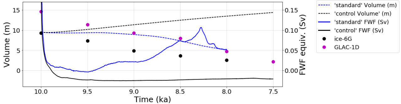
Figure 4. Evolution of ice sheet volume in metres of sea level rise equivalent (dashed line) and freshwater flux (FWF) equivalent in Sverdrups (solid lines). The volumetric SLR equivalent of the ice sheet is calculated from the volume above flotation, and the FWF from the total volumetric change between model years. The volume and FWF in the 'standard' simulation are shown in blue, and for the 'control' simulation in black. The black and magenta markers show the volume in metres of equivalent SLR in the ICE-6G_c (VM5a; Peltier et al., 2015), and the GLAC-1D (Tarasov et al., 2012) reconstructions.
