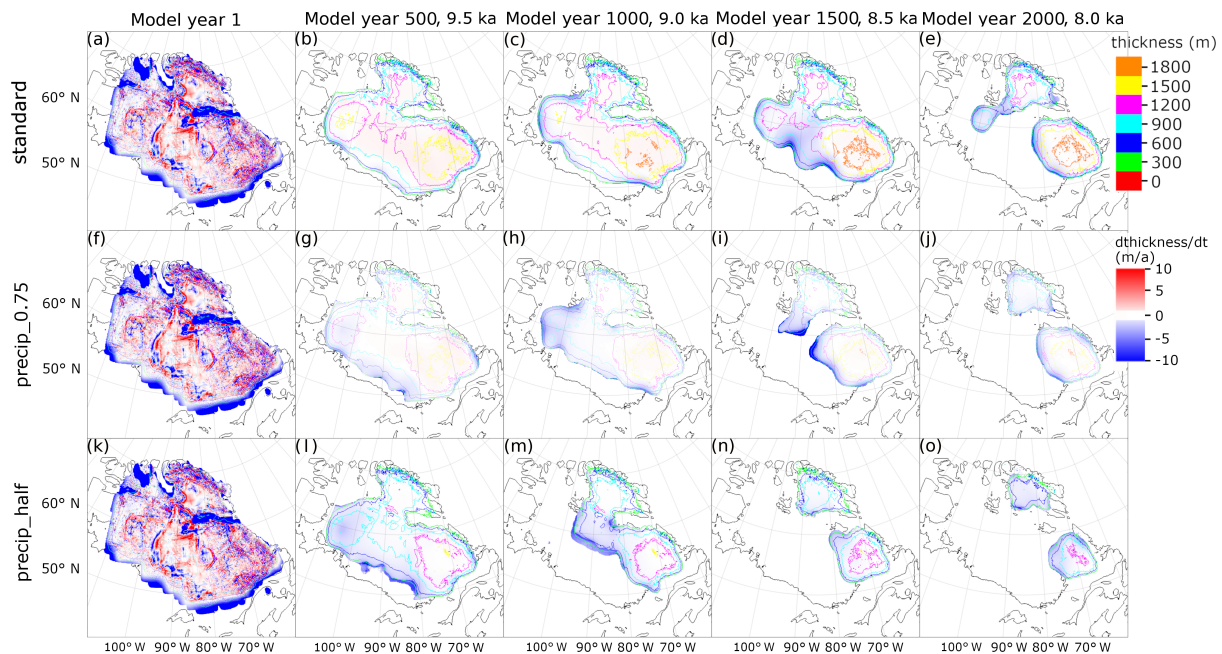
Figure 10. Laurentide Ice Sheet thickness evolution in the three simulations with varying precipitation fields in 500 -year intervals. (a)–(e) 'standard', (f)–(j) 'precip_0.75' ( P field in 'standard' multiplied by 0.75), and (k)–(o) 'precip_half' ( P field in 'standard' halved).
