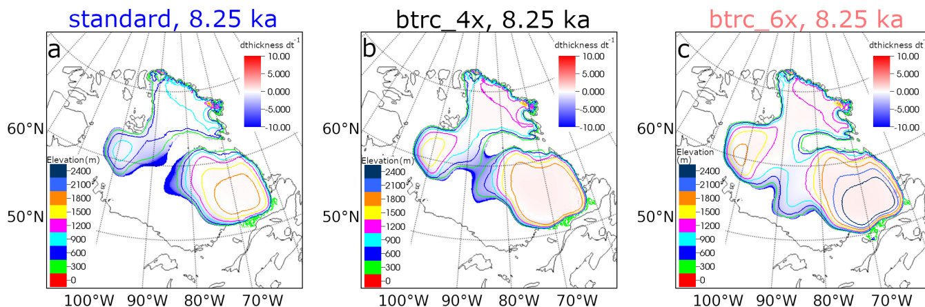
Figure 8. Modelled ice thickness and rate of change of thickness ( \text{m a}^{-1} ) at 8.25 ka in (a) the 'standard' simulation, (b) the 'btrc_4x' simulation in which the standard basal traction coefficient field is quadruple, and (c) 'btrc_6x' in which the standard basal traction coefficient field is multiplied by 6.
