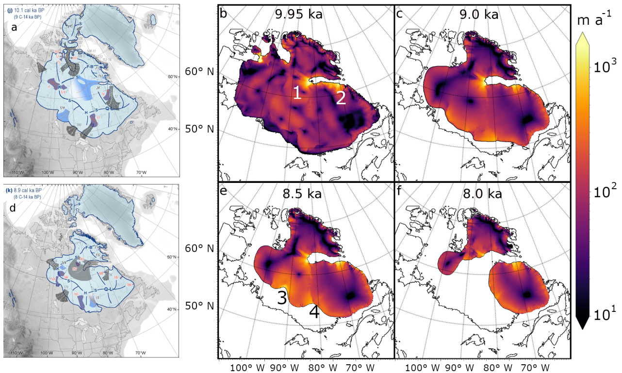
Figure 3. Comparison of modelled and observed ice stream activity. Reconstruction of LIS ice stream activity at 10.1 ka a and 8.9 ka d (adapted from Figure 5 in Margold et al., 2018). The ice streams that were active at the respective times are shown in light blue, ice streams that 'switched off' in the preceding 1000 years are shown in grey and those that 'switched on' shown in dark blue. Panels b , c , e and f show the magnitude of depth-integrated velocities ( ma^{-1} ) in the 'standard' simulation at 9.95 ka, 9.00 ka, 8.5 ka and at the end of the simulation (8.00 ka) respectively. In the panels showing the simulated ice velocities, modern coastlines are indicated by the black contour. The numbers 1 & 2 in panel b and numbers 3 & 4 in panel e show the approximate locations of four major reconstructed ice streams, and correspond to locations numbered 24, 16, 179 and 33 in fig. 5 in Margold et al. (2018) respectively.
