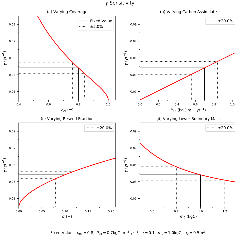
Figure C1. The sensitivity of the mortality rate to assumed input variables: coverage, \nu_{eq} (a), and carbon assimilate rate, P_{eq} (b), and model parameters: reseed fraction, \alpha (c) and boundary mass, m_0 (d). The solid black line indicates the fixed values with corresponding \pm 20\% (b,c,d) or \pm 5\% (a) variation (dotted black lines).
