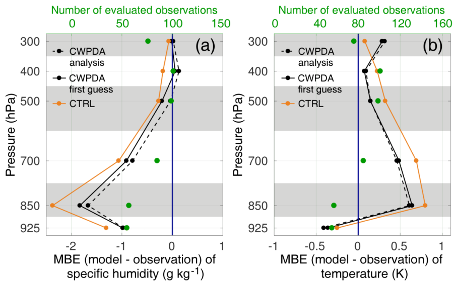
Figure 5. Vertical profiles of the MBE per bins of pressure for specific humidity (a) and temperature (b), for the two experiments CWPDA (black) and CTRL (orange), with respect to independent radiosonde observations. The solid lines show the ensemble mean first guesses. The dashed line shows the analyses of CWPDA. A dashed line does not exist for CTRL since prior and posterior are identical. The number of evaluated observations per pressure bin is shown in green. All cycling periods listed in Table 1 including 43 radiosoundings at 1200 UTC at Gillot-Aeroport are considered.
