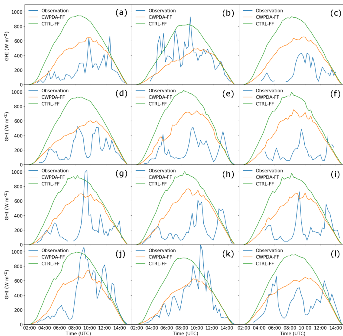
Figure 8. GHI on Reunion Island on 12 January 2018 as observed (blue), and forecasted by CWPDA-FF (orange) and CTRL-FF (green) with IDW post-processing for the sites Plaine des Cafres (a), Gros Piron Sainte-Rose (b), Cilaos (c), Bellevue Bras-Panon (d), Le Port (e), Colimacons (f), Piton-Maido (g), Pointe des Trois-Bassins (h), Petite-France (i), Pierrefonds-Aéroport (j), Le Baril (k), Gillot-Aéroport (l).
