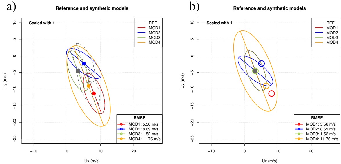
Figure 4. Uncentered (left) and centered (right) versions of the Sailor diagram after placing the ellipses from all the synthetic datasets in the same plot.
