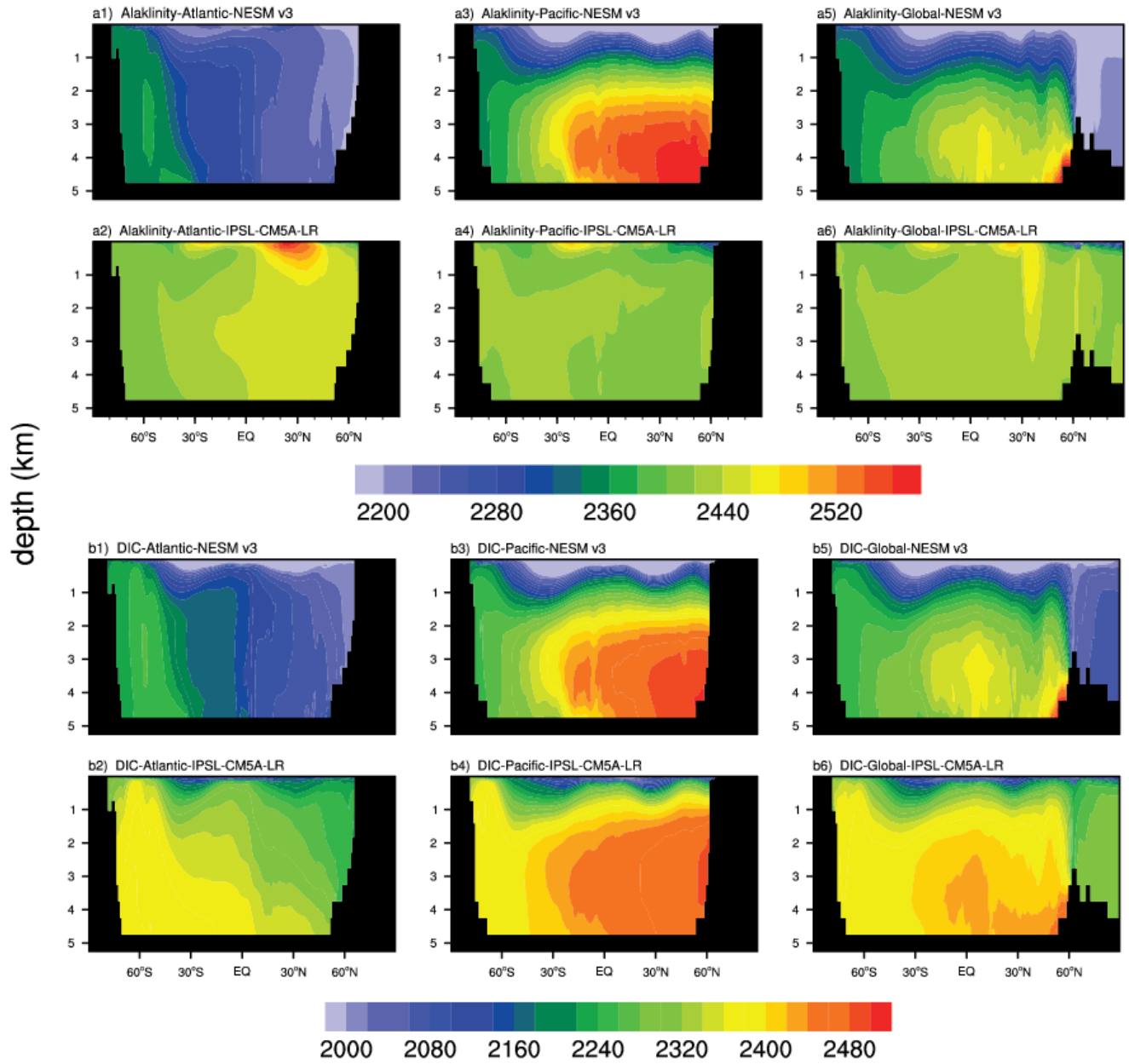
Fig. S4. The latitude-depth distribution of alkalinity and DIC from the PI-experiment of NESM v3 and IPSL-CM5A-LR (with a unit of \text{mmol m}^{-3} ).
