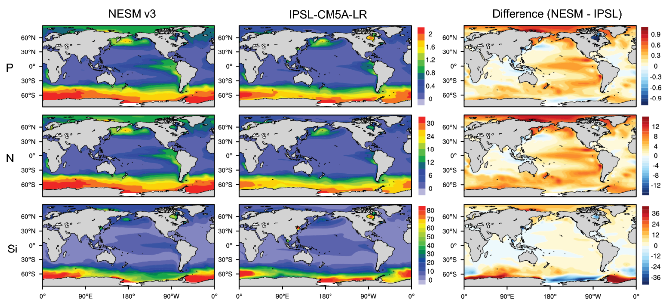
Fig. S1. Annual mean upper ocean (averaged in the upper 100m) distribution of phosphate ( \text{PO}_4^{3-} ), nitrate ( \text{NO}_3^- ), and silicate ( \text{SiO}_4^{2-} ) from the PI-experiment of NESM v3 and IPSL-CM5A-LR.
