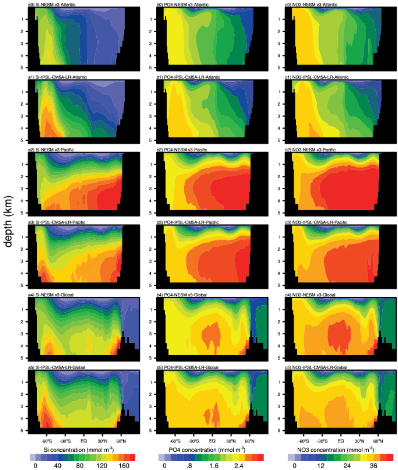
Fig. S2. The latitude-depth distribution of silicate (a), phosphate (b), and nitrate (c) from the PI-experiment of NESM v3 and IPSL-CM5A-LR (with a unit of mmol m -3 ).
