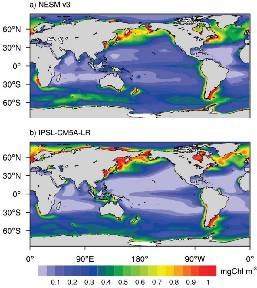
Fig. S5. Annual mean upper ocean (0-50m) chlorophyll concentration (mg Chl m -3 ) climatology from PI-experiment of the NESM v3 (a) and IPSL-CM5A-LR (b).
