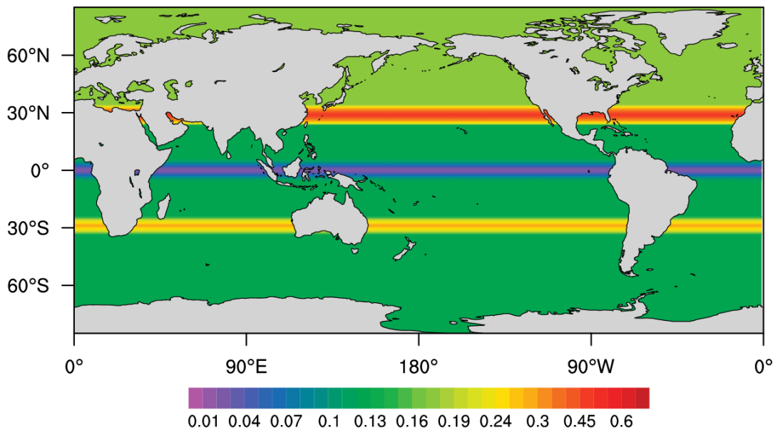
Fig. S0. Latitude-dependent vertical diffusivity distribution (in unit of \text{cm}^2 \text{ s}^{-1} ).
