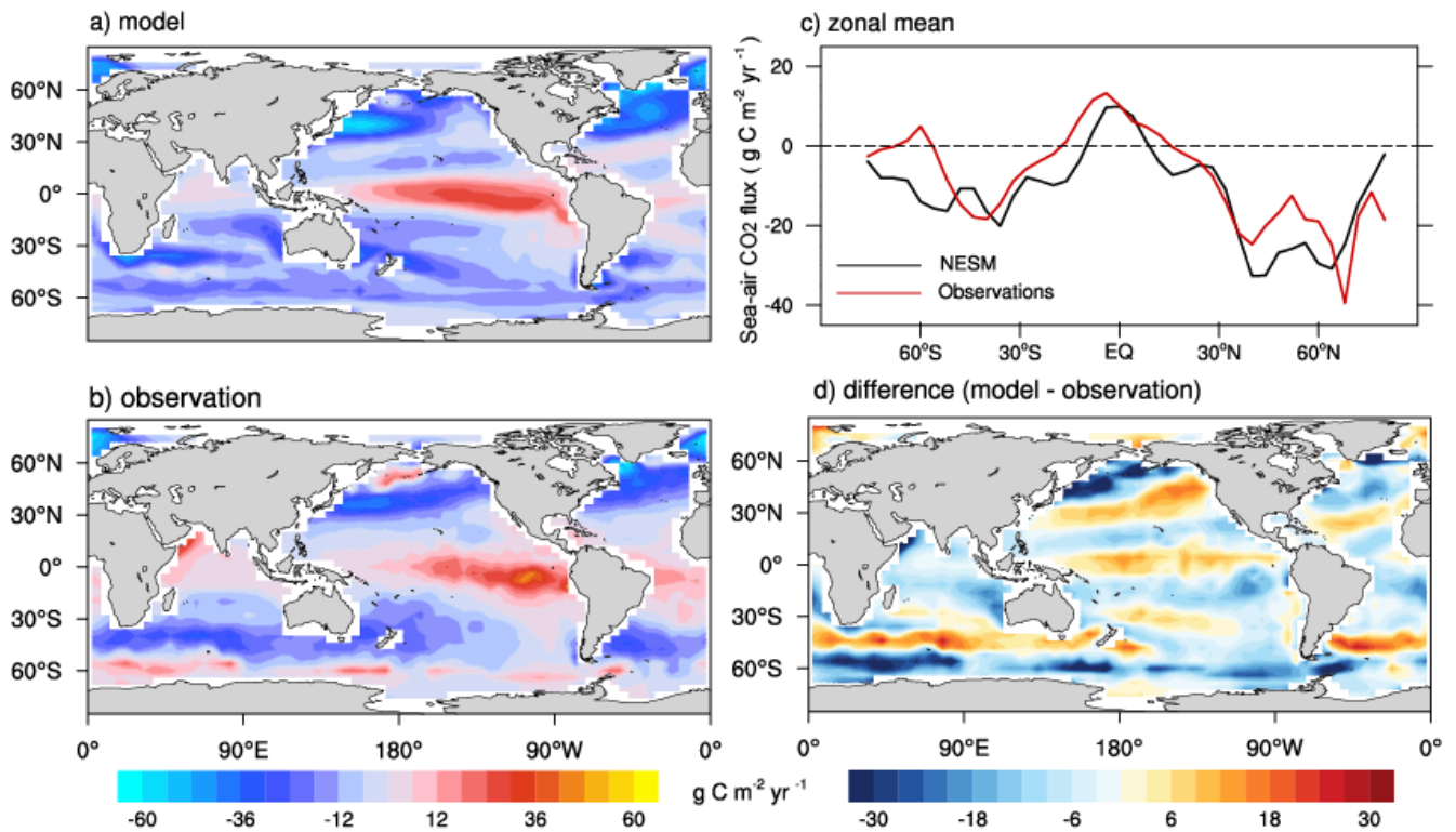
Figure 10. Model-simulated sea-air CO 2 flux ( \text{g C m}^{-2} \text{yr}^{-1} ) in the year 2000 compared with data-based observational estimates (Takahashi et al., 2009). Spatial distributions of model simulation (a), observation (b), zonal mean pattern of model simulation and observation (c), and the difference between model and observation (d). Positive values represent CO 2 flux out of the ocean, and negative values represent CO 2 flux into the ocean.
